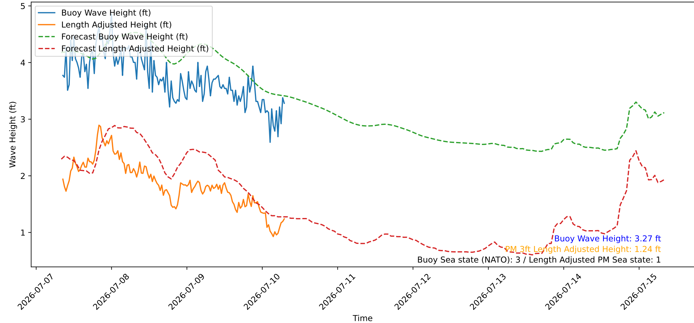
Wave Heights over Time for Red Beach at 2026-07-10 08:00:45
