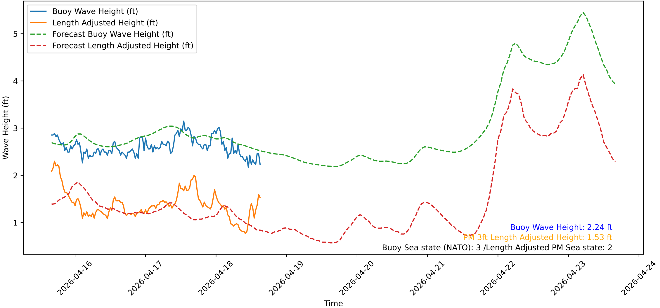
Wave Heights over Time for Red Beach at 2026-04-18 15:50:51
