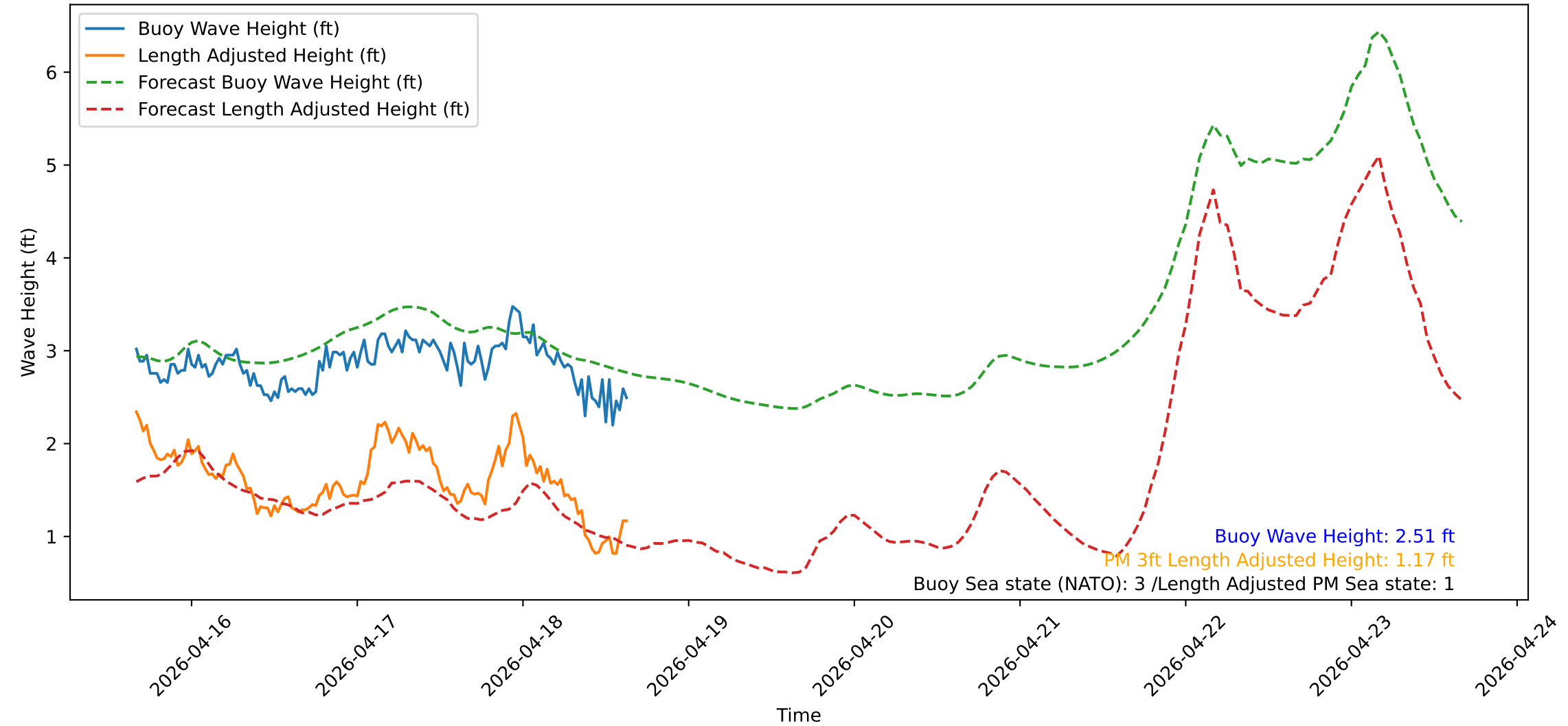
Wave Heights over Time for Green Beach at 2026-04-18 15:51:13
