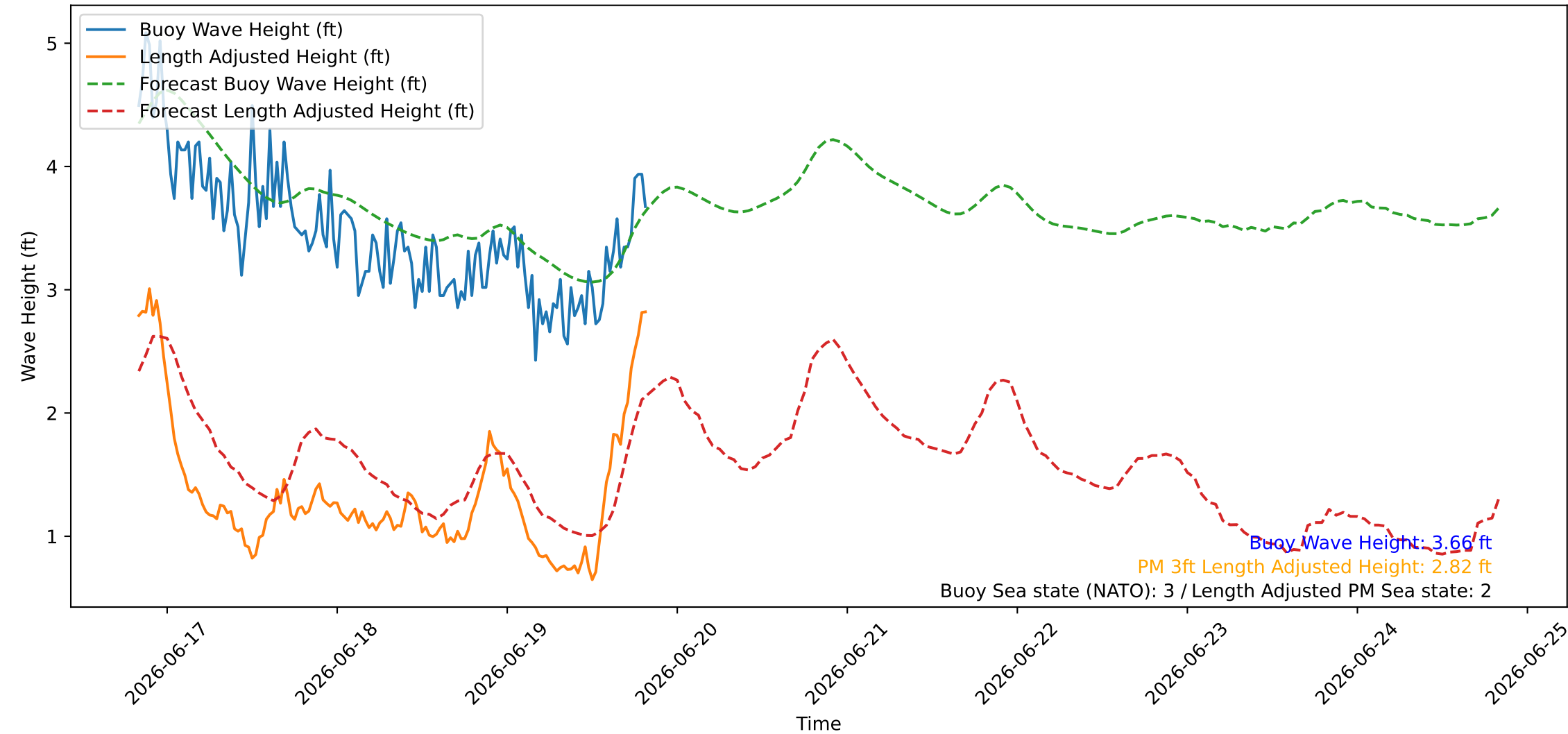
Wave Heights over Time for Green Beach at 2026-06-19 20:11:08
