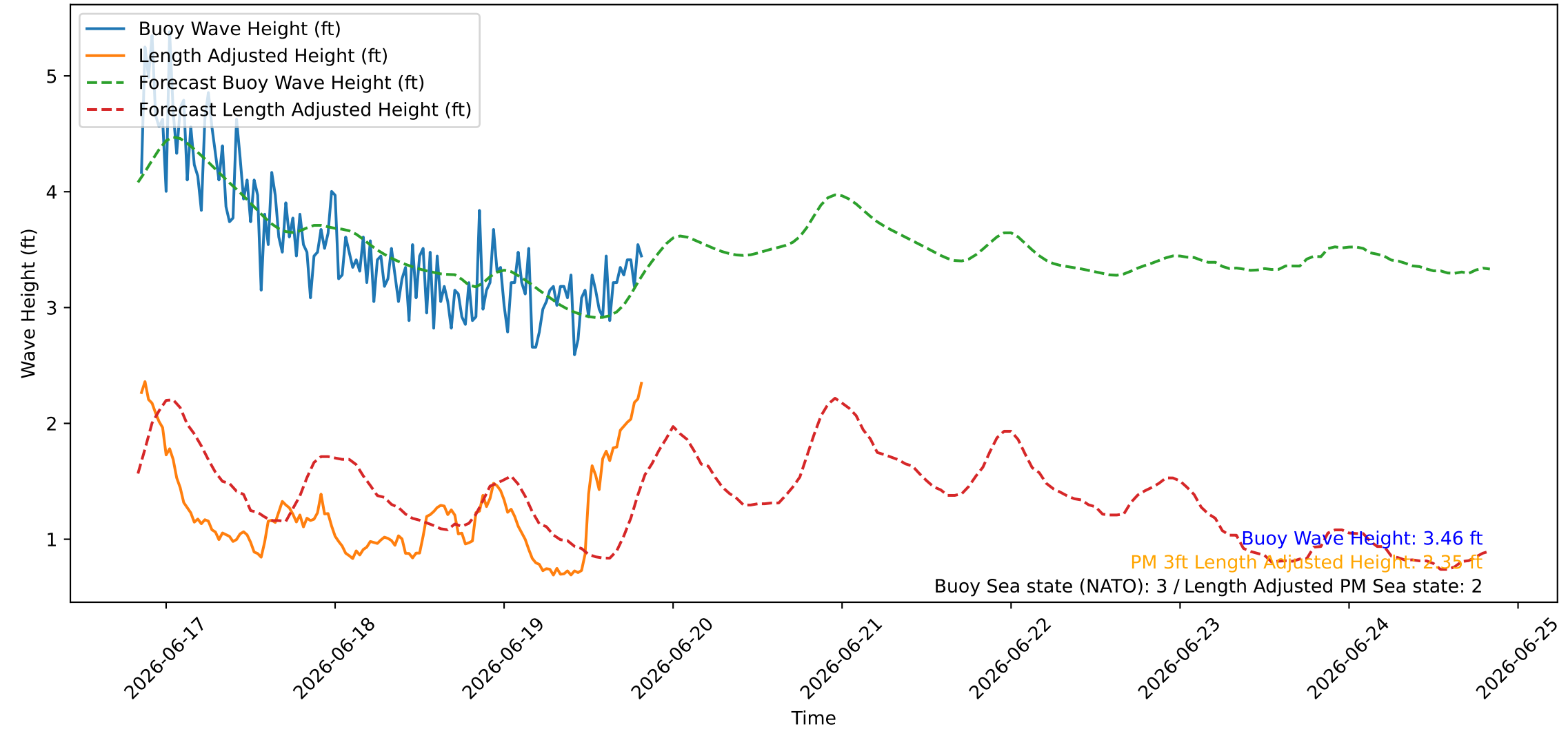
Wave Heights over Time for Red Beach at 2026-06-19 20:10:45
