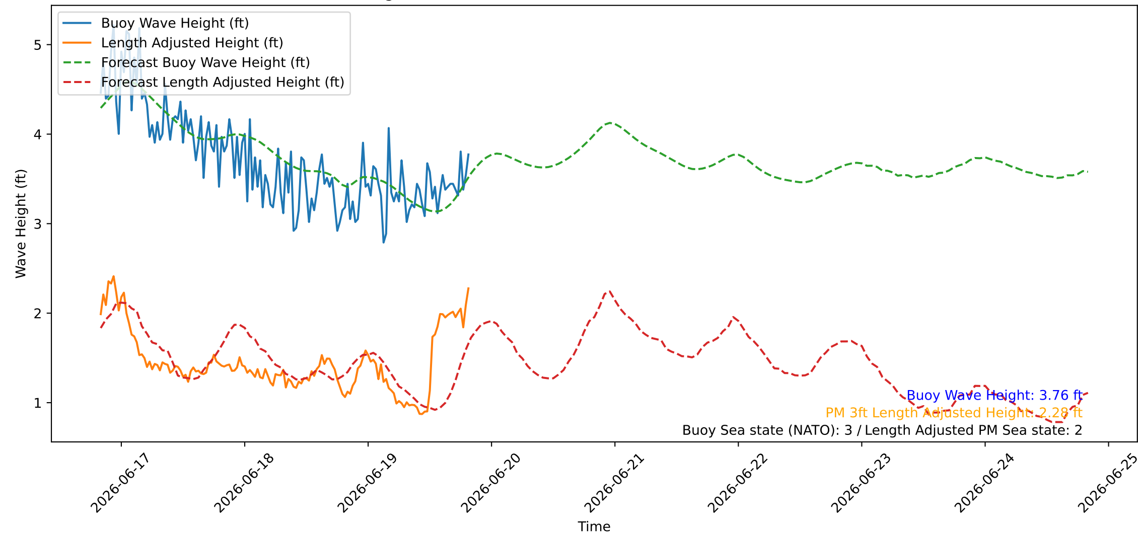
Wave Heights over Time for Oceanside Harbor at 2026-06-19 20:10:26
