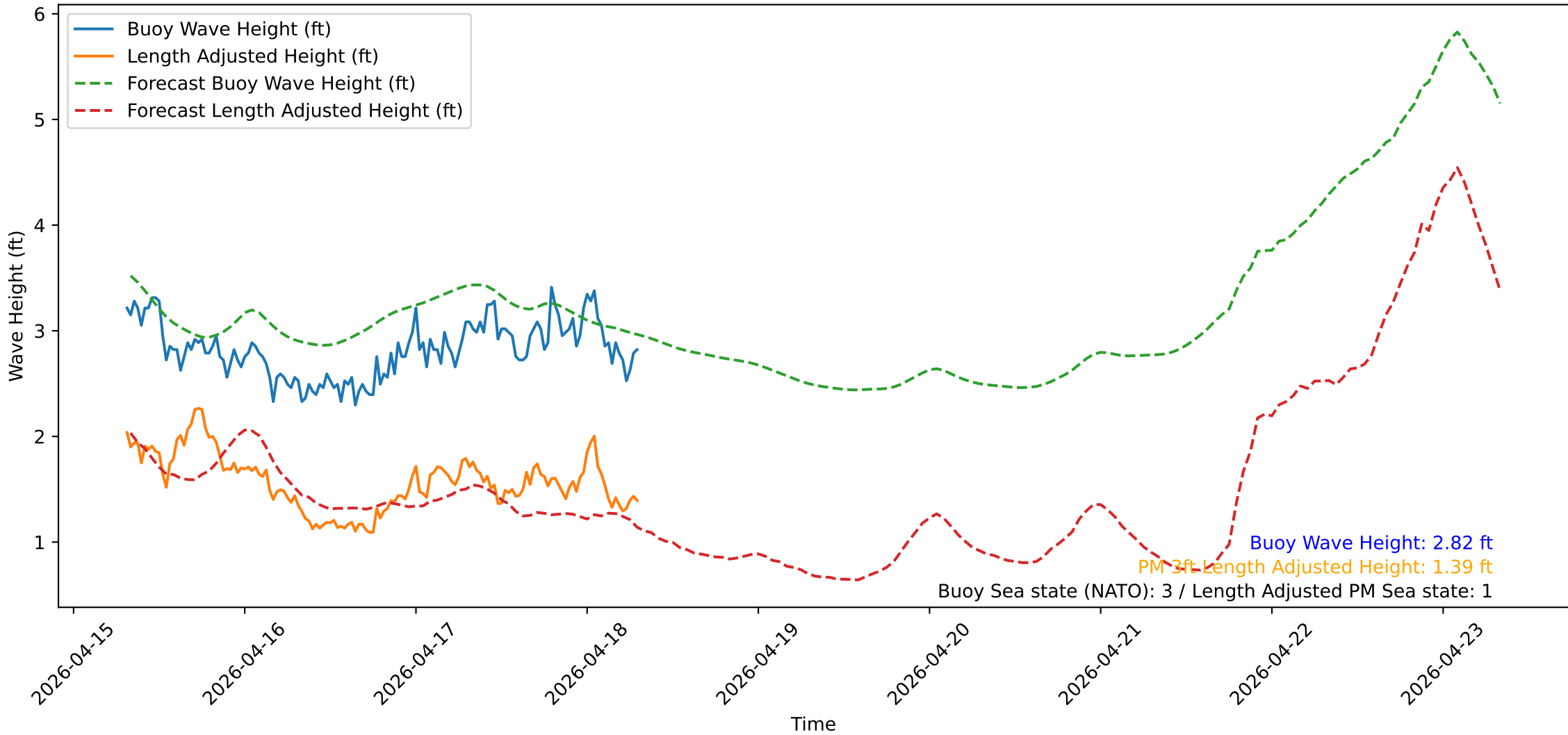
Wave Heights over Time for Oceanside Harbor at 2026-04-18 07:40:31
