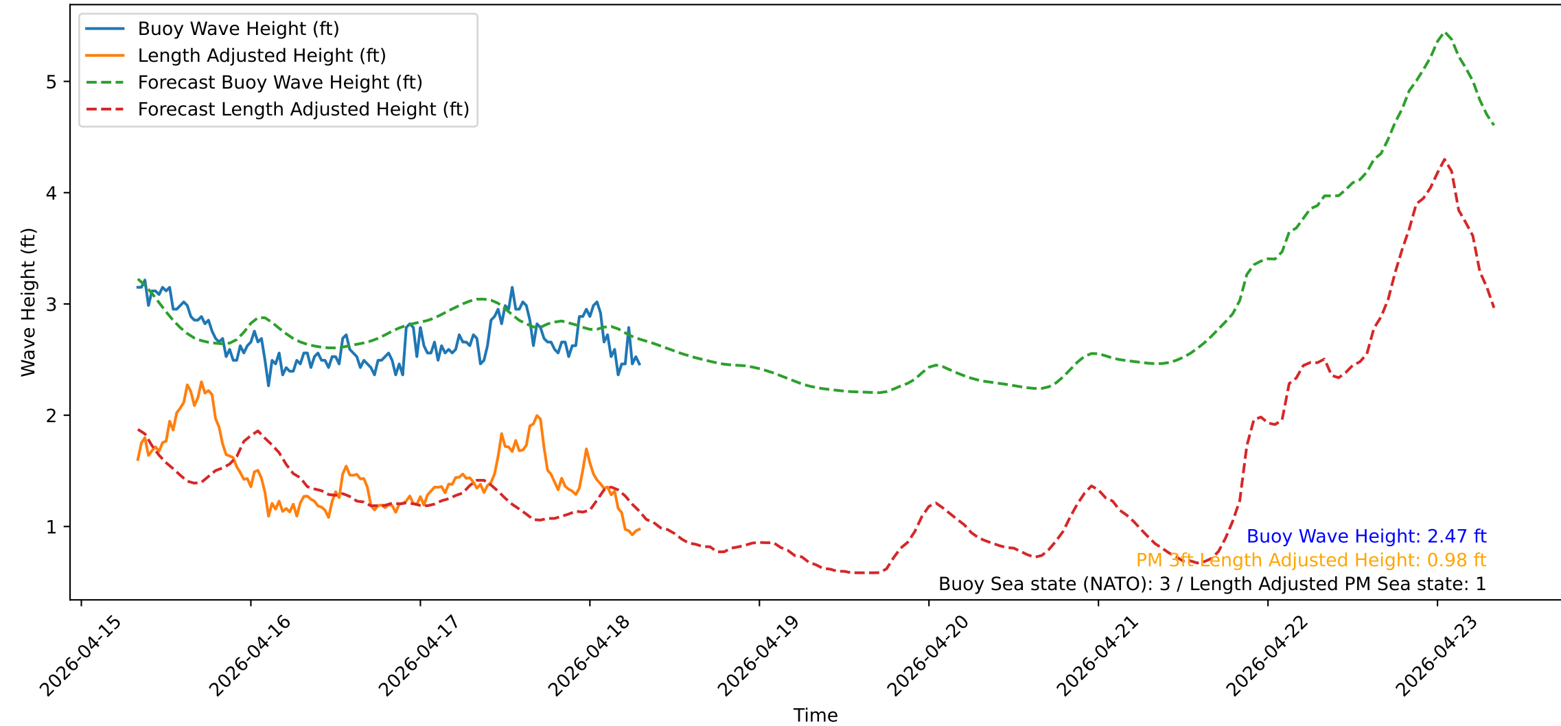
Wave Heights over Time for Red Beach at 2026-04-18 07:40:50
