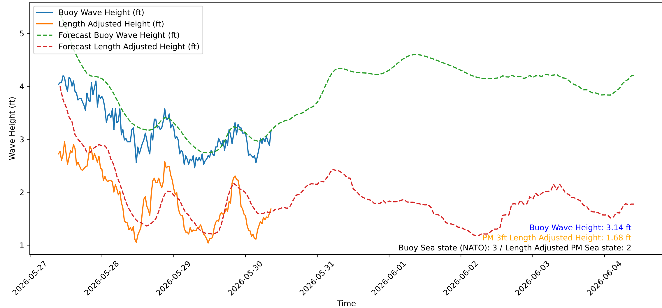
Wave Heights over Time for Green Beach at 2026-05-30 09:31:05
