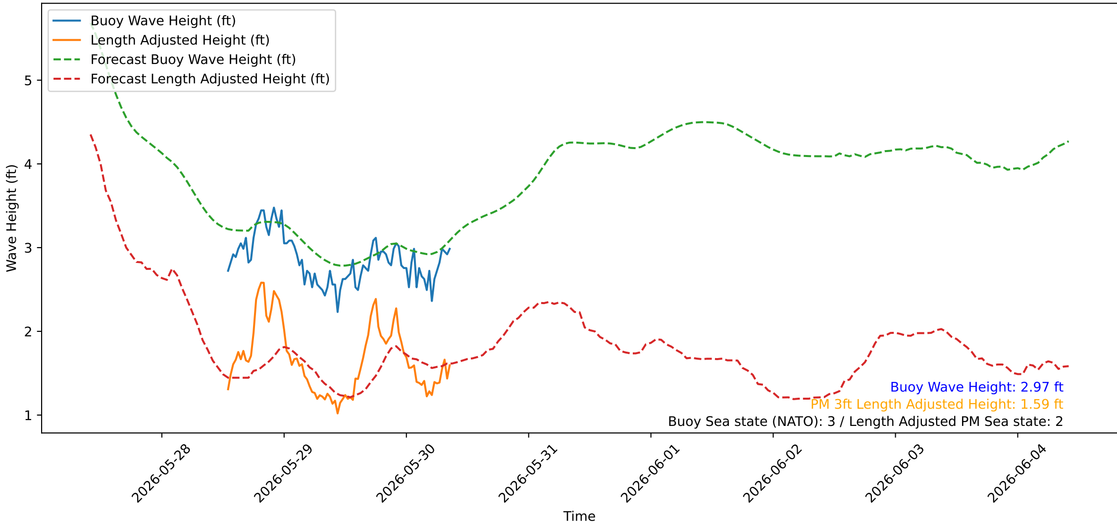
Wave Heights over Time for Oceanside Harbor at 2026-05-30 09:30:24
