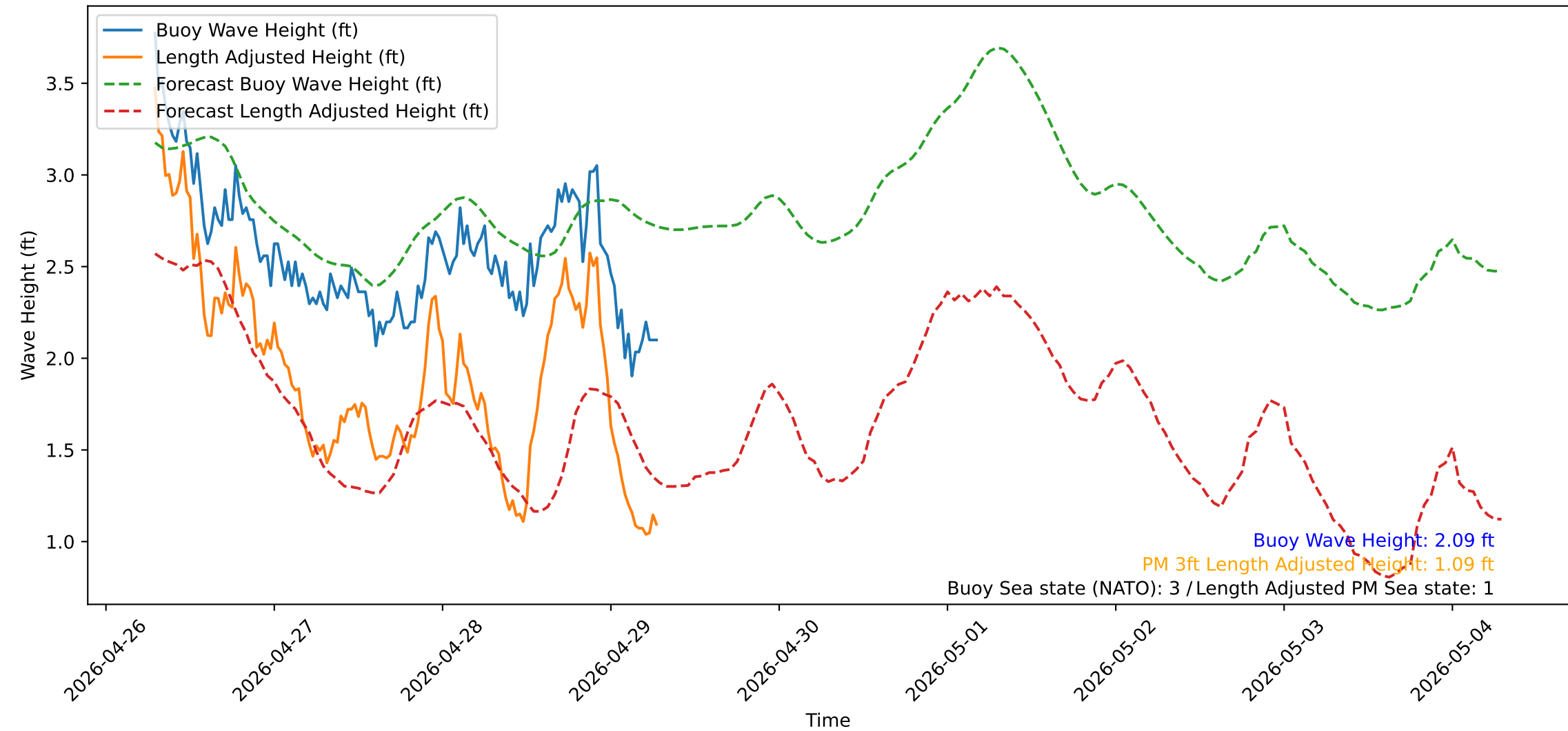
Wave Heights over Time for Oceanside Harbor at 2026-04-29 07:00:31
