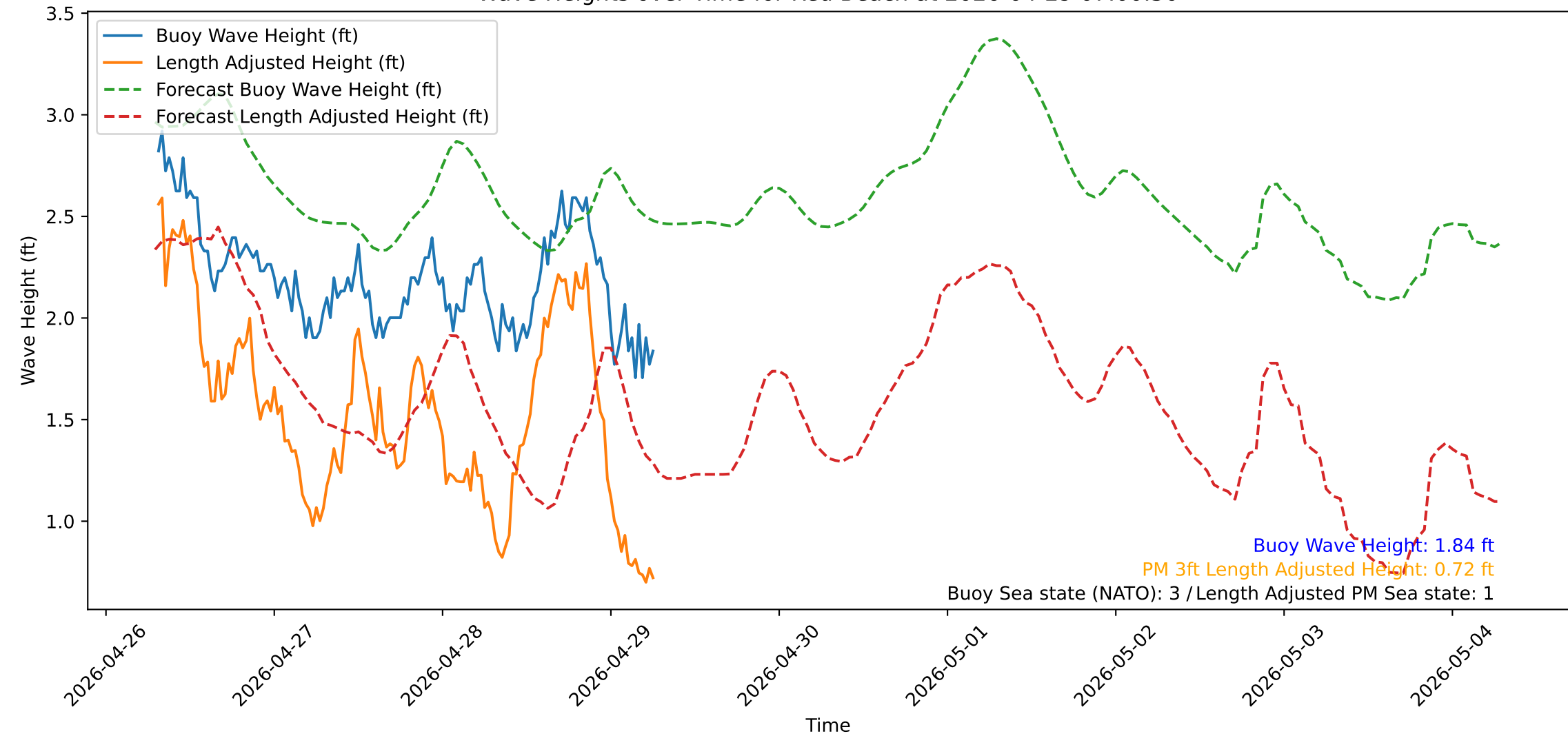
Wave Heights over Time for Red Beach at 2026-04-29 07:00:50
