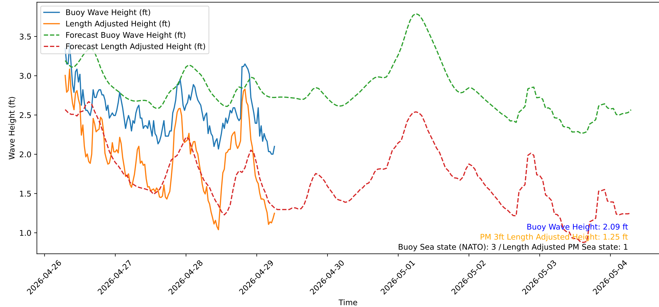
Wave Heights over Time for Green Beach at 2026-04-29 07:01:13
