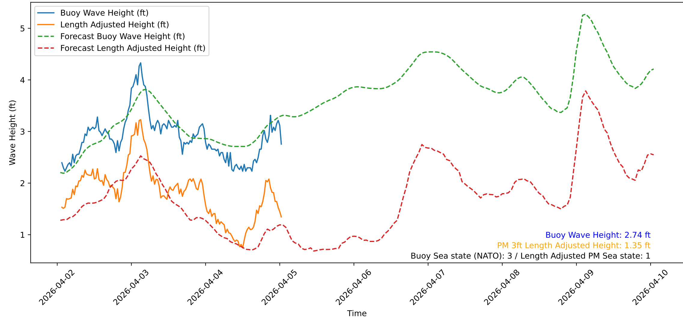
Wave Heights over Time for Green Beach at 2026-04-05 01:21:09
