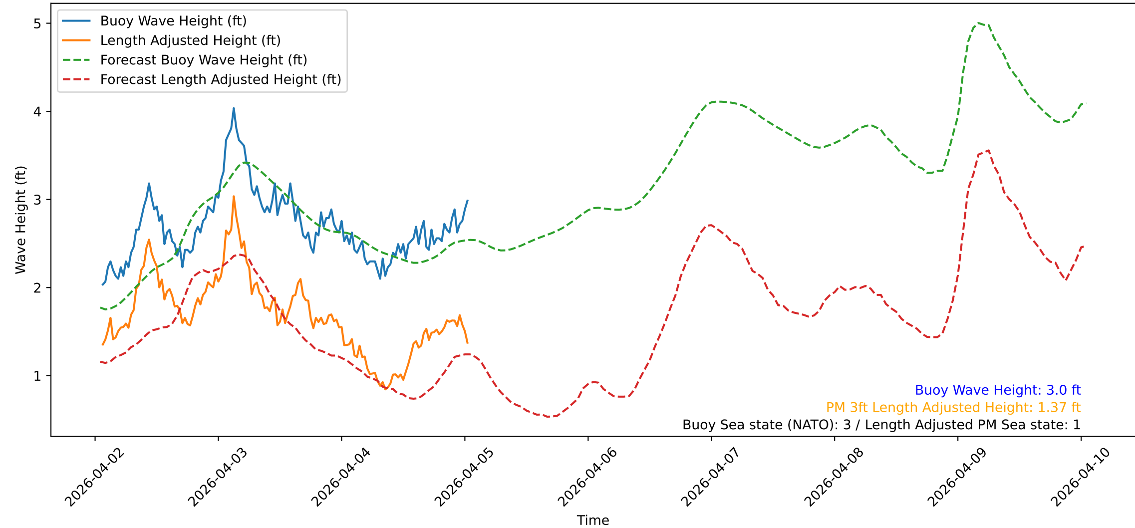
Wave Heights over Time for Oceanside Harbor at 2026-04-05 01:20:31
