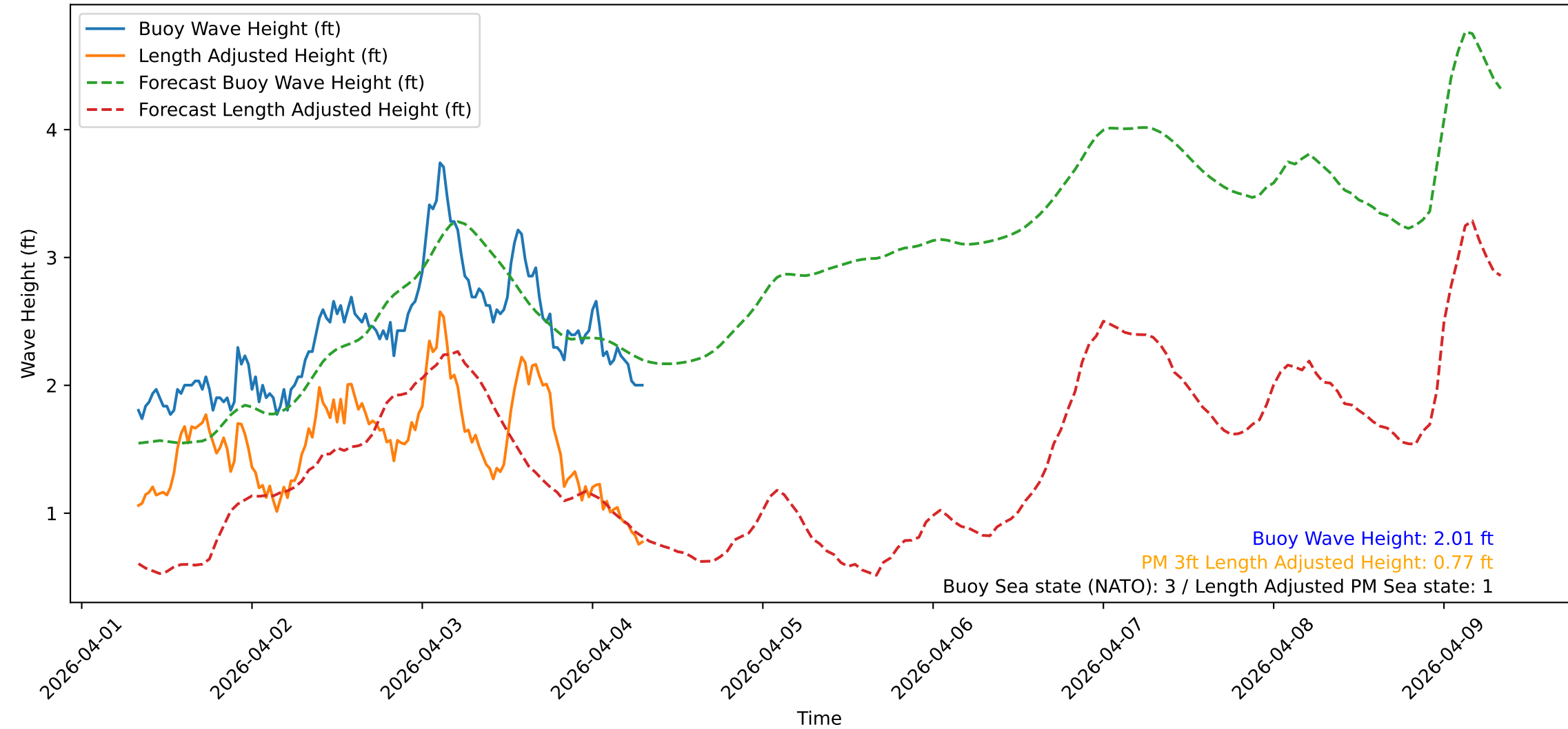
Wave Heights over Time for Red Beach at 2026-04-04 07:50:48
