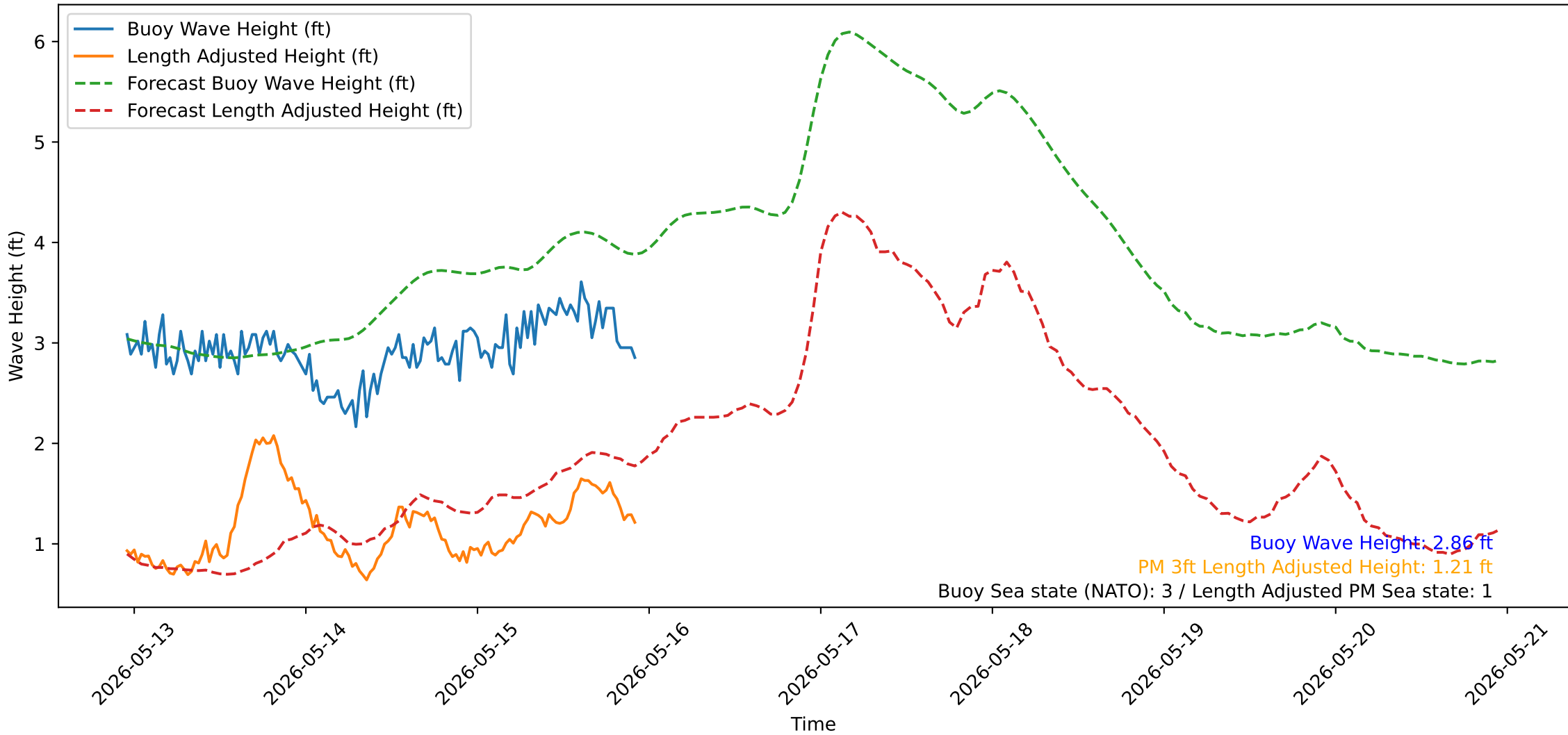
Wave Heights over Time for Oceanside Harbor at 2026-05-15 22:50:32
