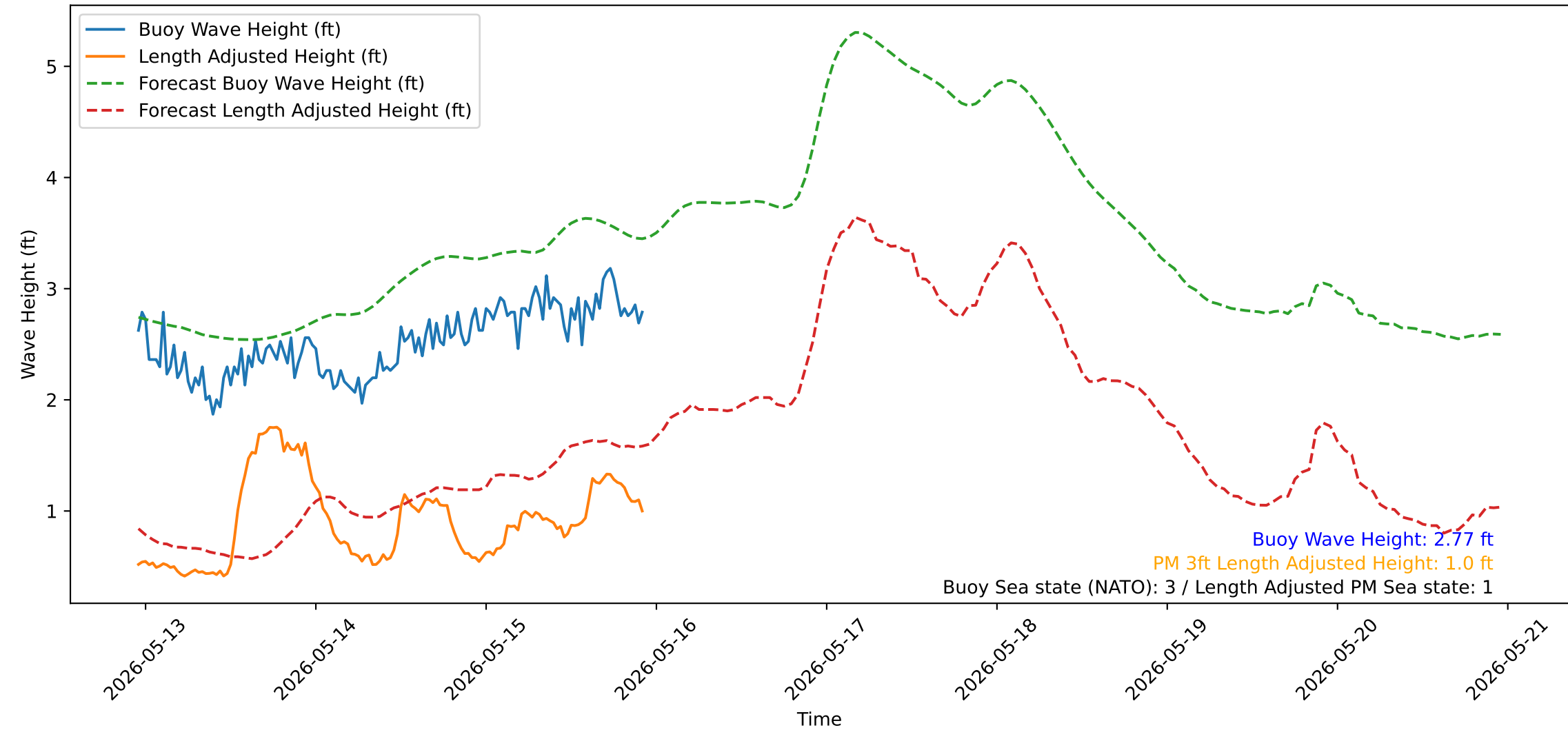
Wave Heights over Time for Red Beach at 2026-05-15 22:50:52
