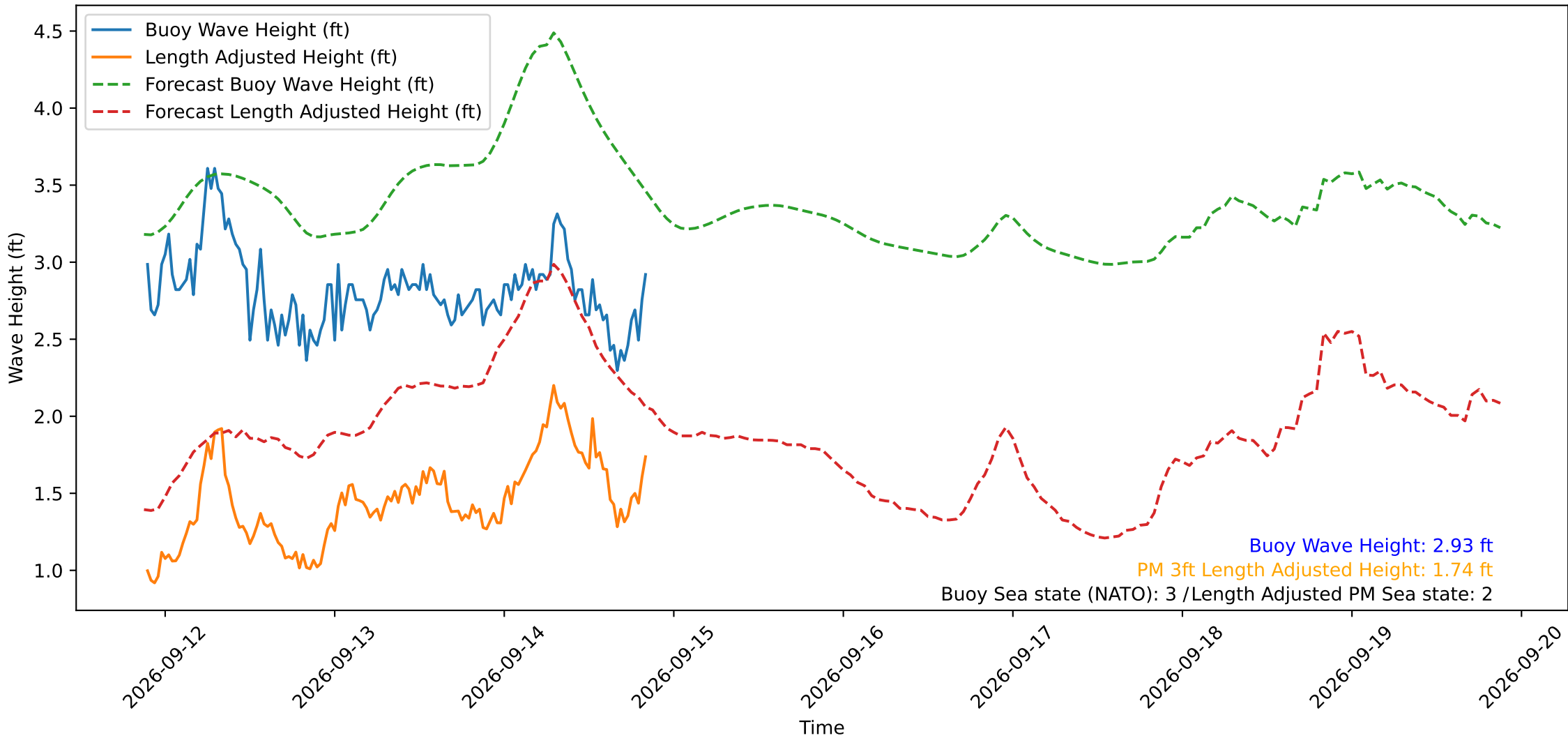
Wave Heights over Time for Green Beach at 2026-09-14 21:01:12
