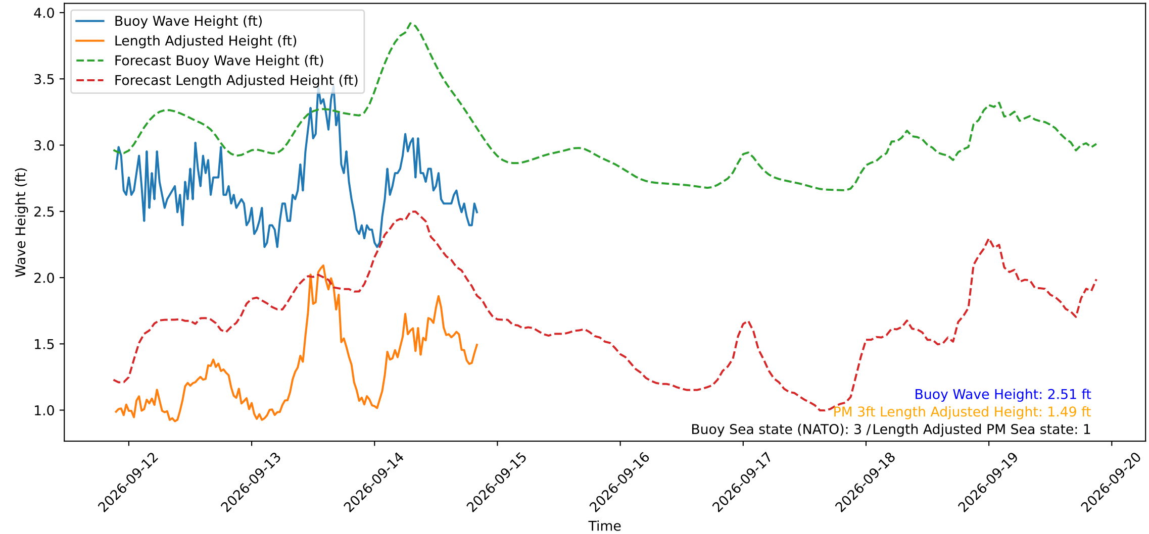
Wave Heights over Time for Red Beach at 2026-09-14 21:00:49
