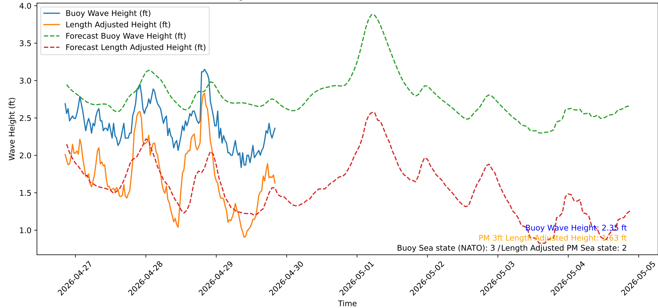
Wave Heights over Time for Green Beach at 2026-04-29 20:41:14
