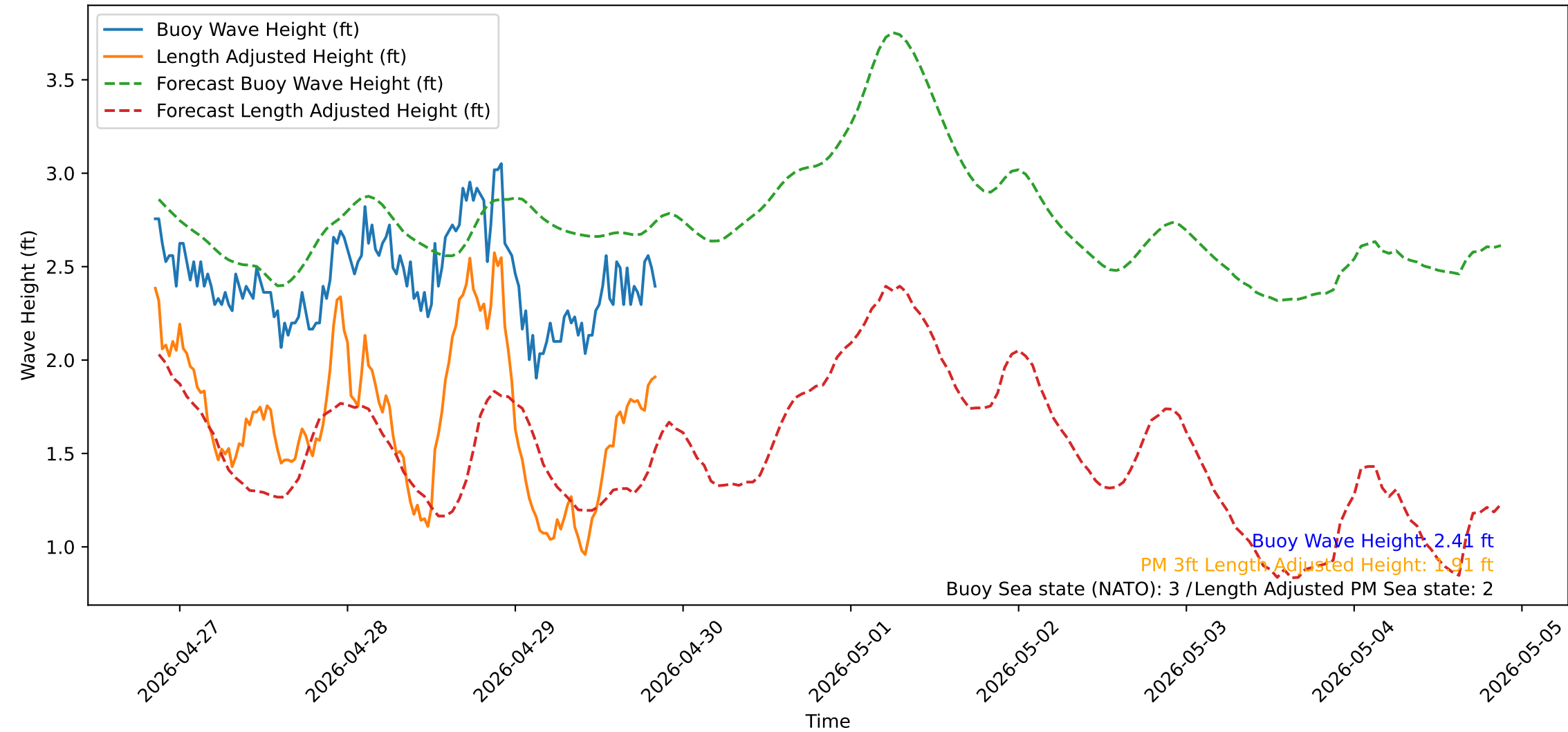
Wave Heights over Time for Oceanside Harbor at 2026-04-29 20:40:31
