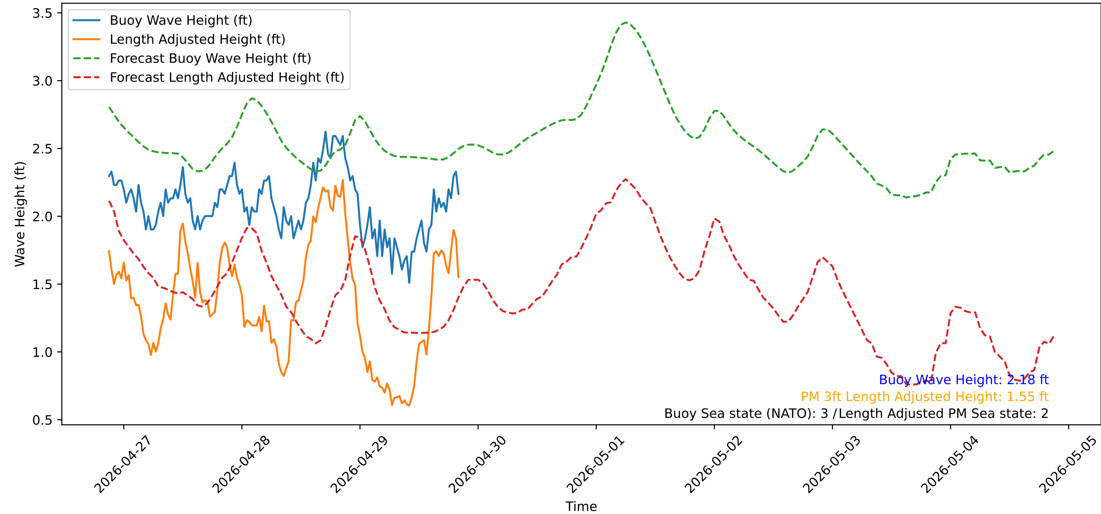
Wave Heights over Time for Red Beach at 2026-04-29 20:40:51
