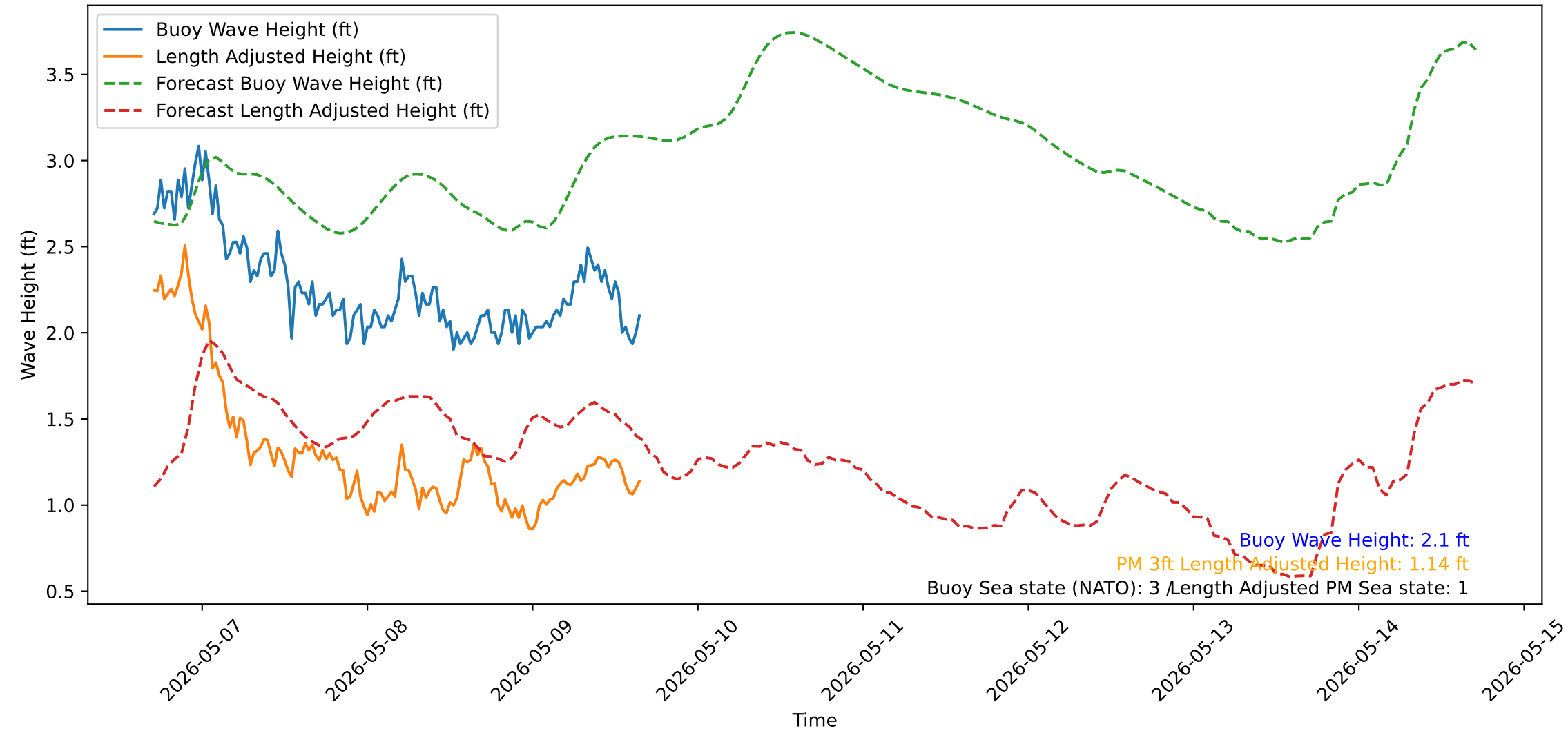
Wave Heights over Time for Red Beach at 2026-05-09 16:30:50
