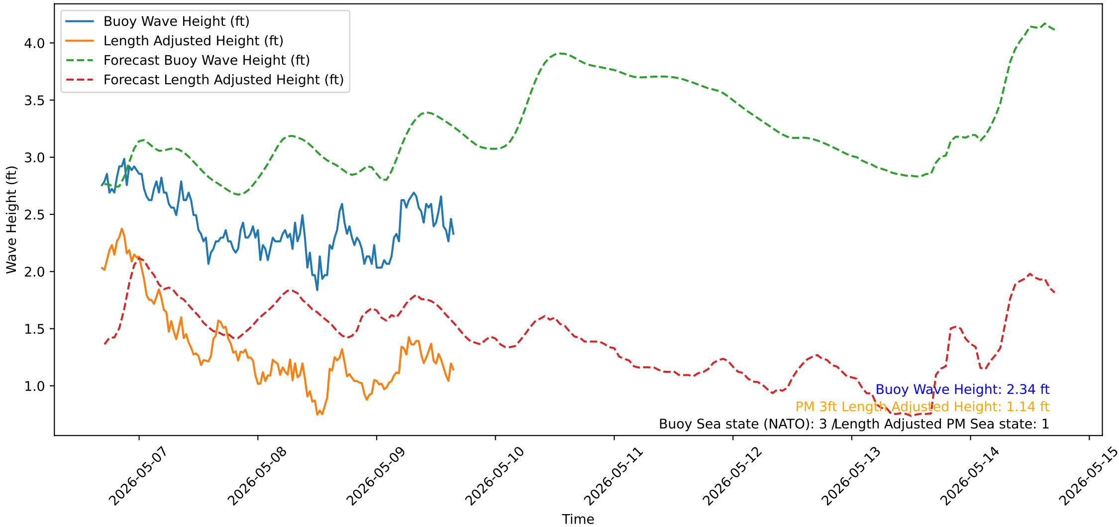
Wave Heights over Time for Green Beach at 2026-05-09 16:31:13
