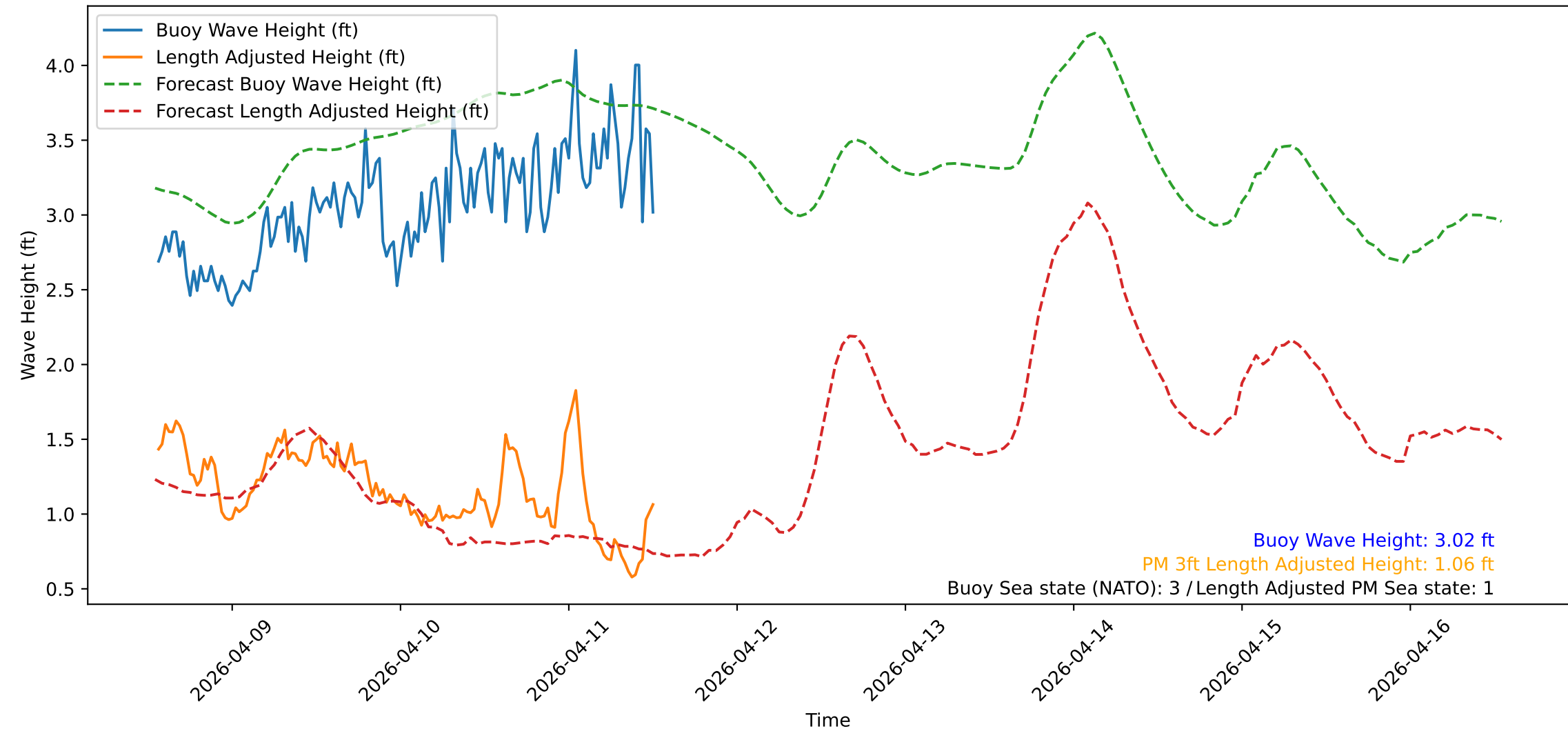
Wave Heights over Time for Red Beach at 2026-04-11 13:10:51
