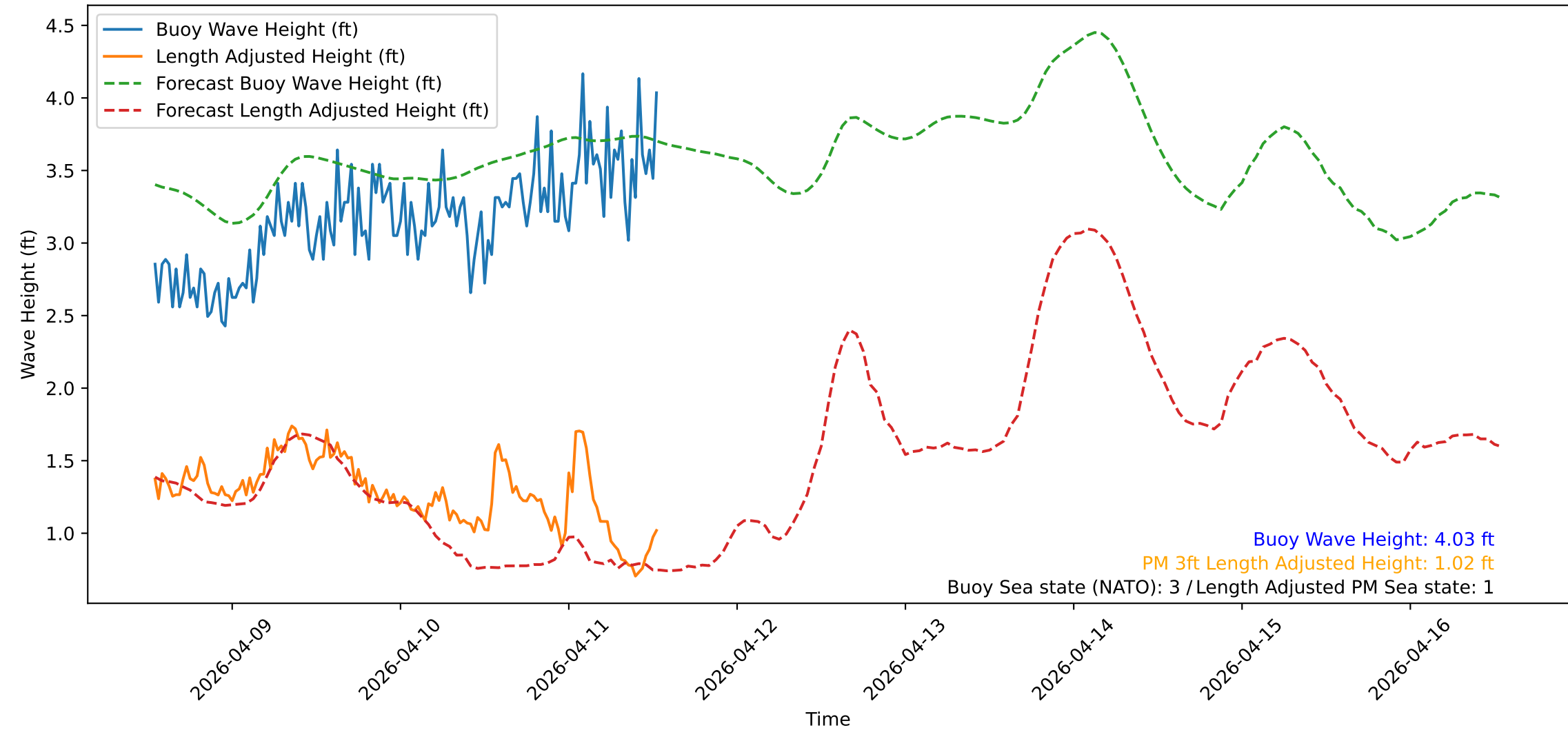
Wave Heights over Time for Oceanside Harbor at 2026-04-11 13:10:31
