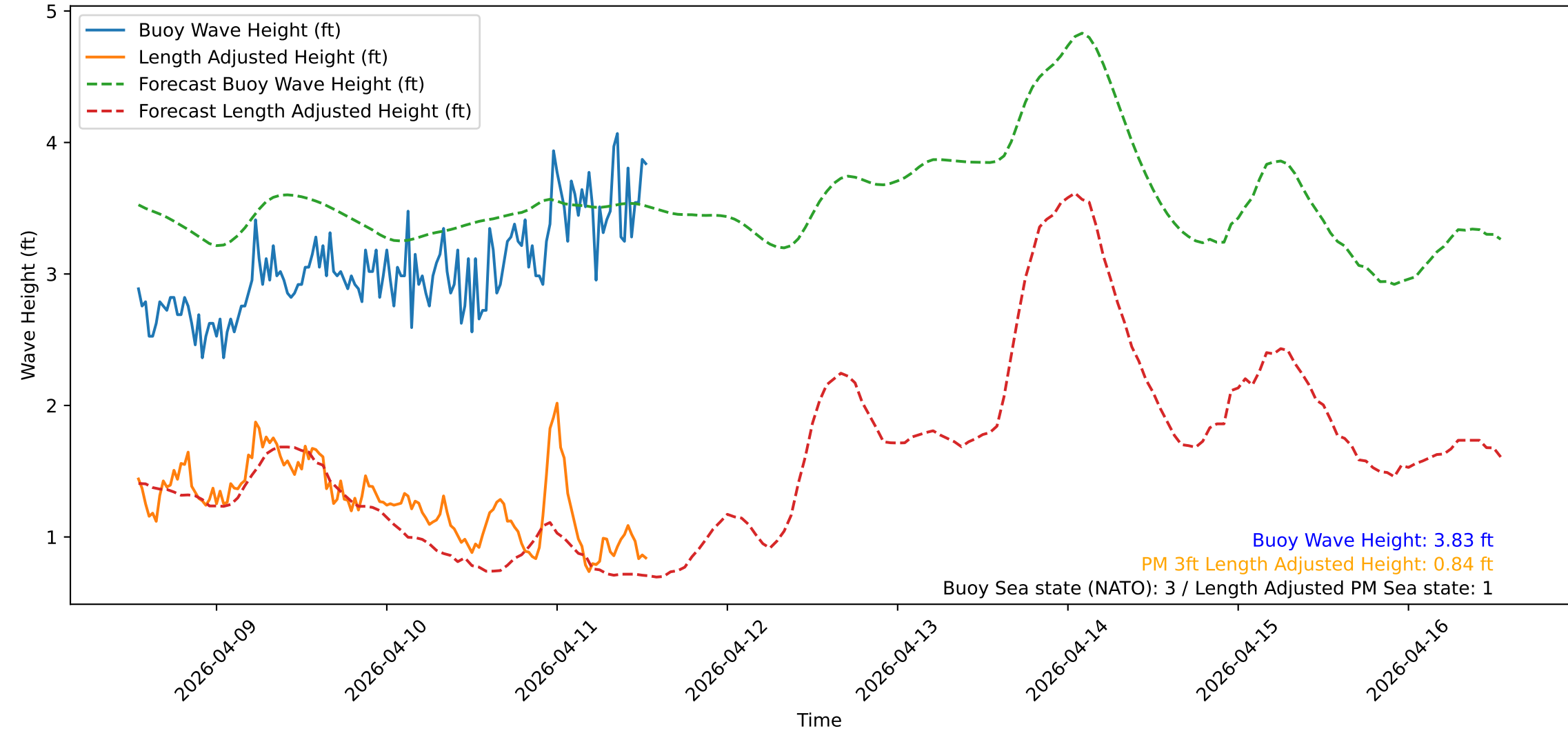
Wave Heights over Time for Green Beach at 2026-04-11 13:11:14
