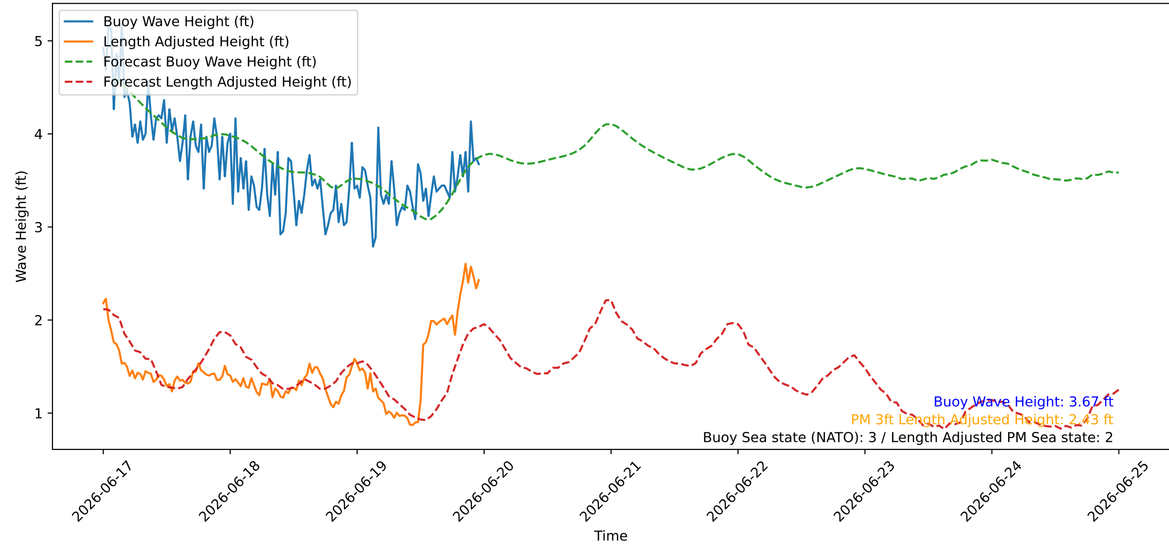
Wave Heights over Time for Oceanside Harbor at 2026-06-19 23:50:26
