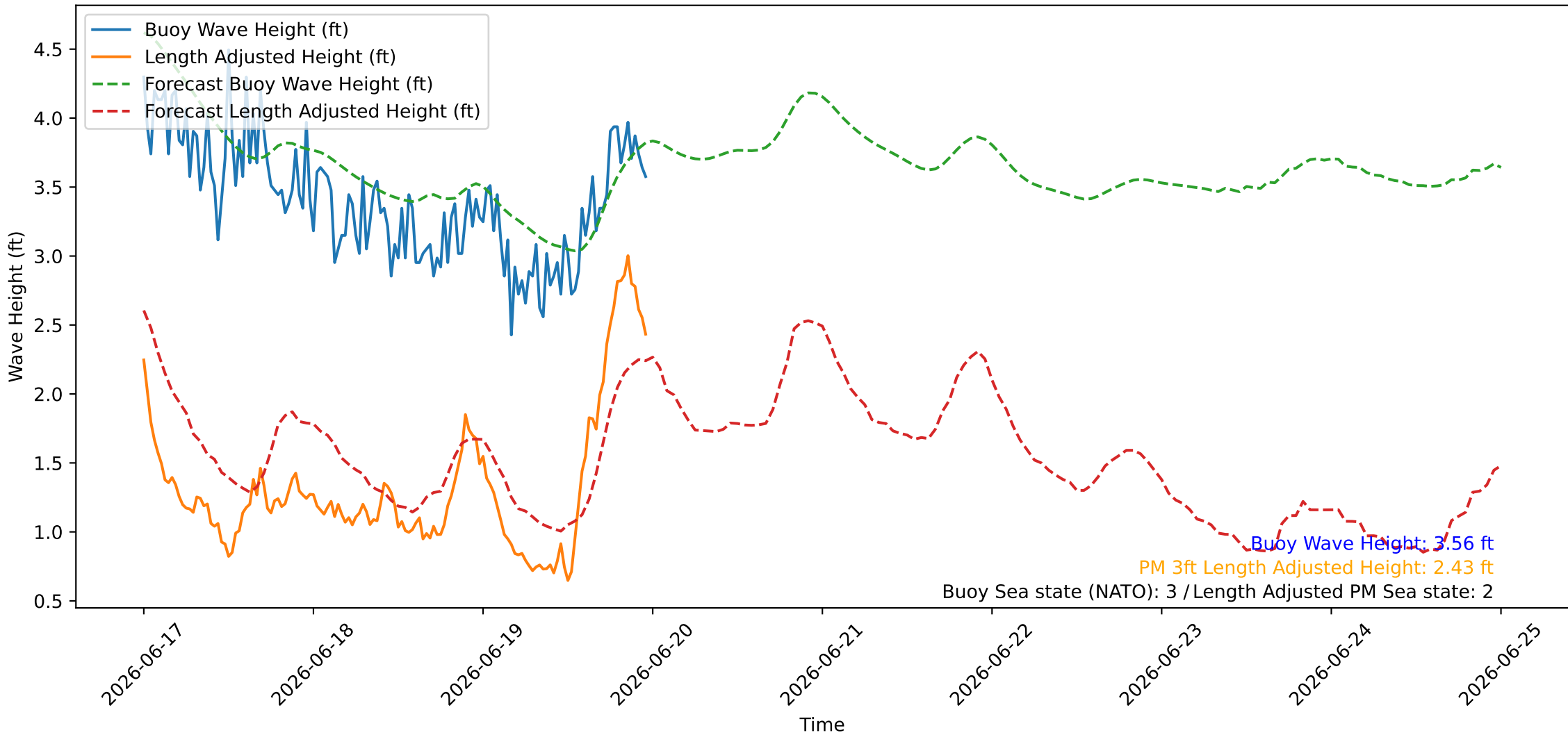
Wave Heights over Time for Green Beach at 2026-06-19 23:51:09
