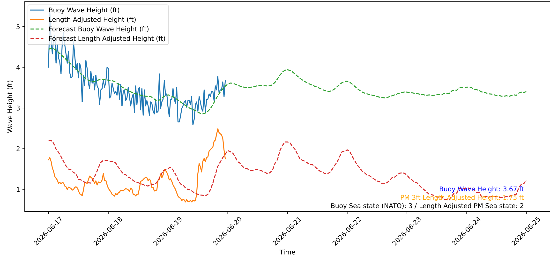
Wave Heights over Time for Red Beach at 2026-06-19 23:50:47
