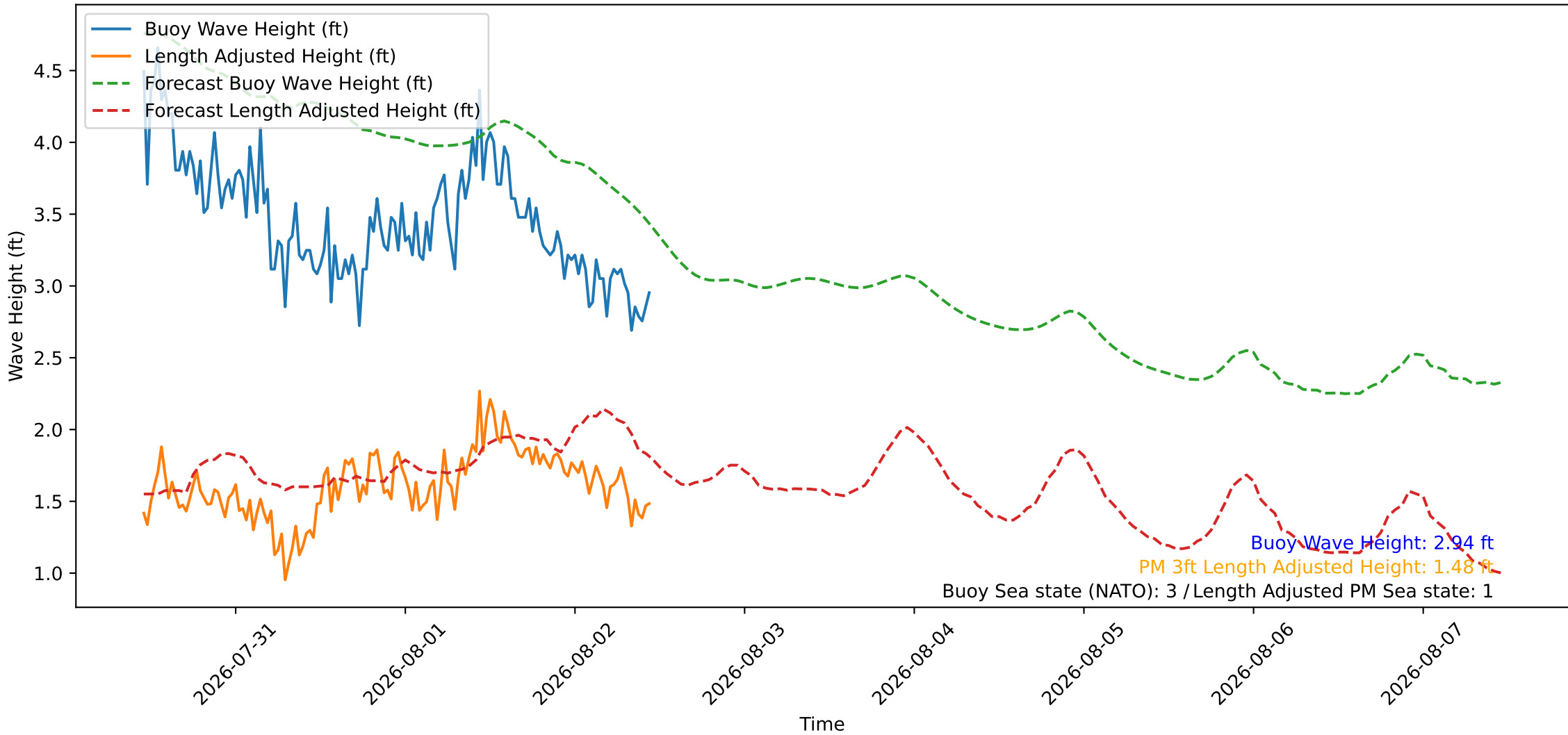
Wave Heights over Time for Oceanside Harbor at 2026-08-02 11:10:26
