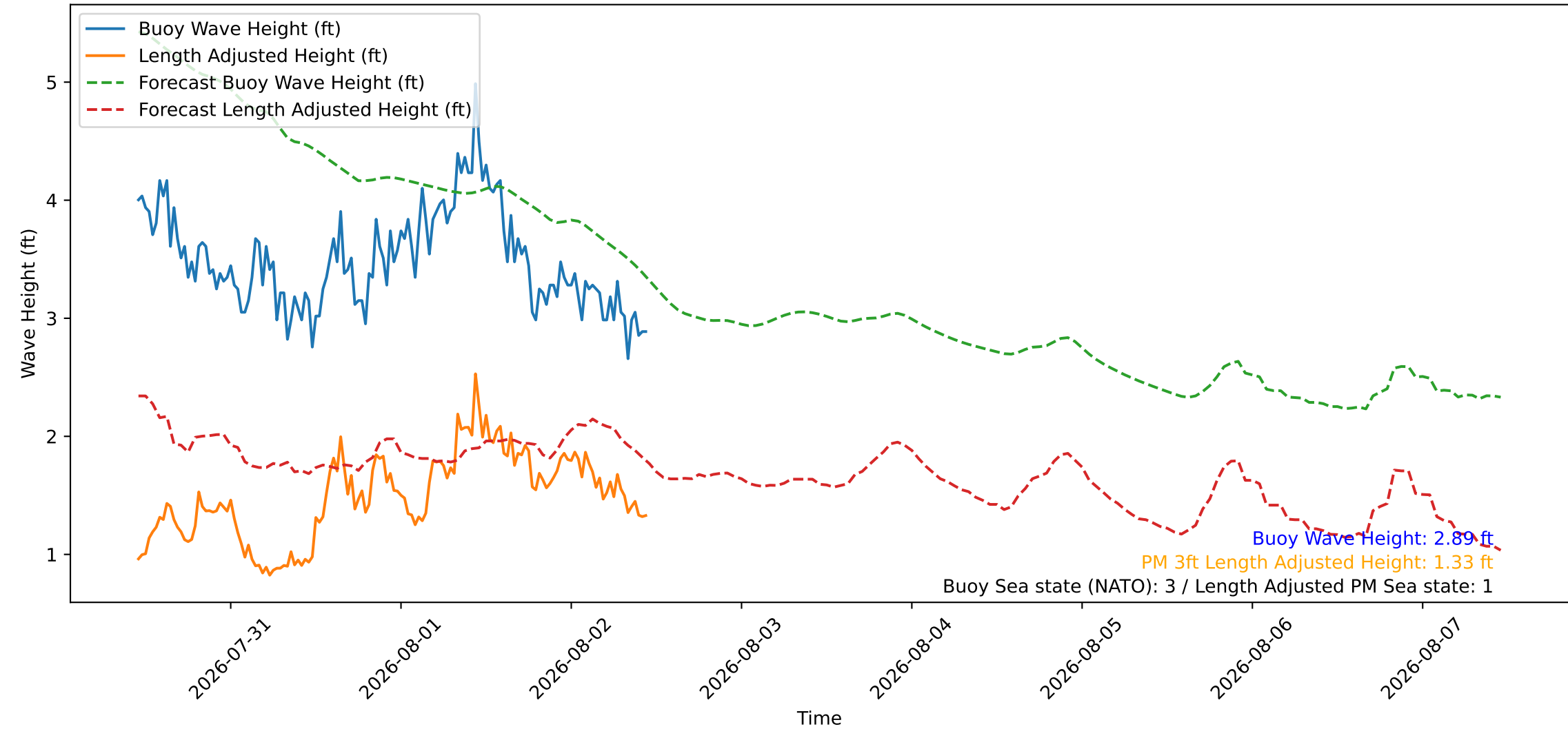
Wave Heights over Time for Green Beach at 2026-08-02 11:11:08
