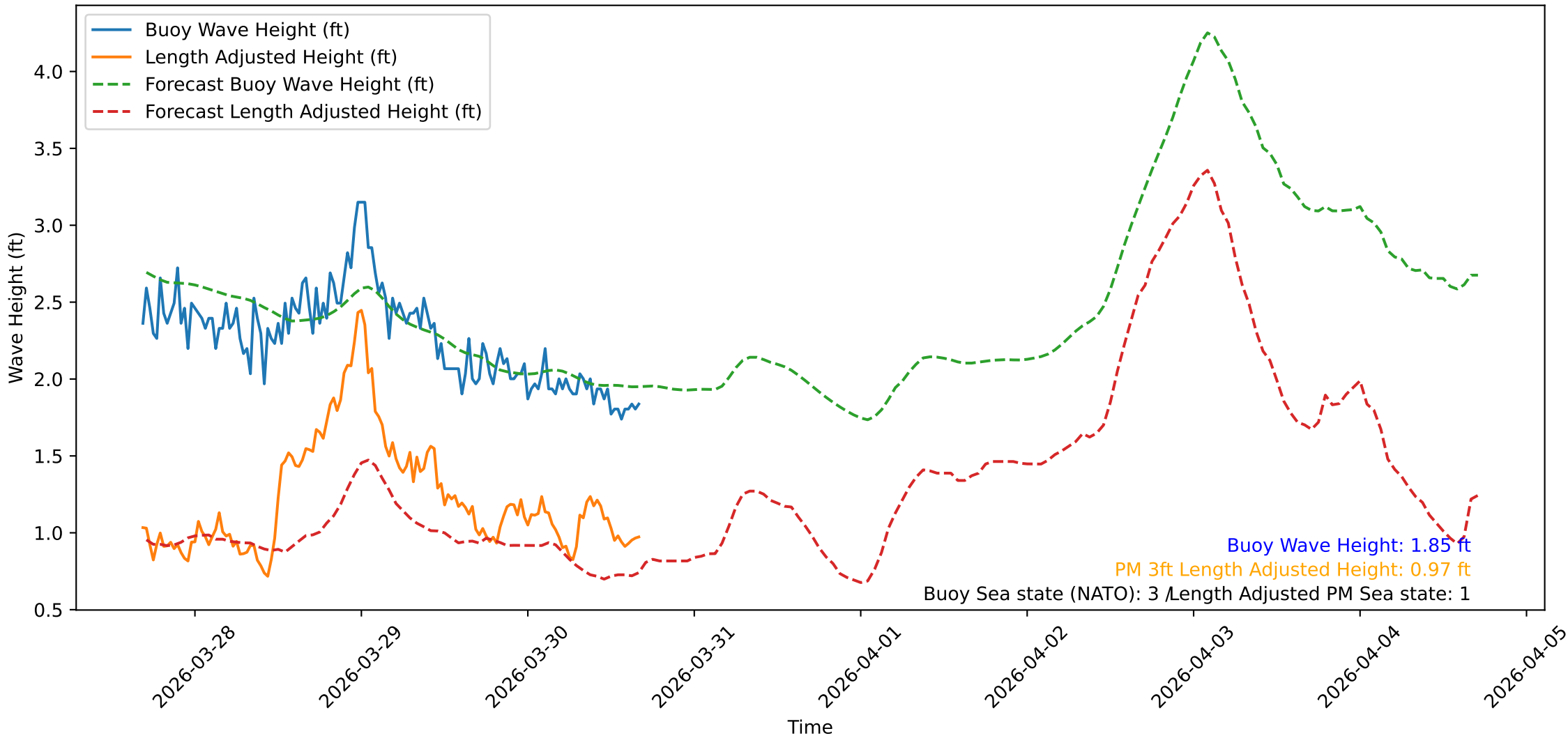
Wave Heights over Time for Oceanside Harbor at 2026-03-30 16:30:32
