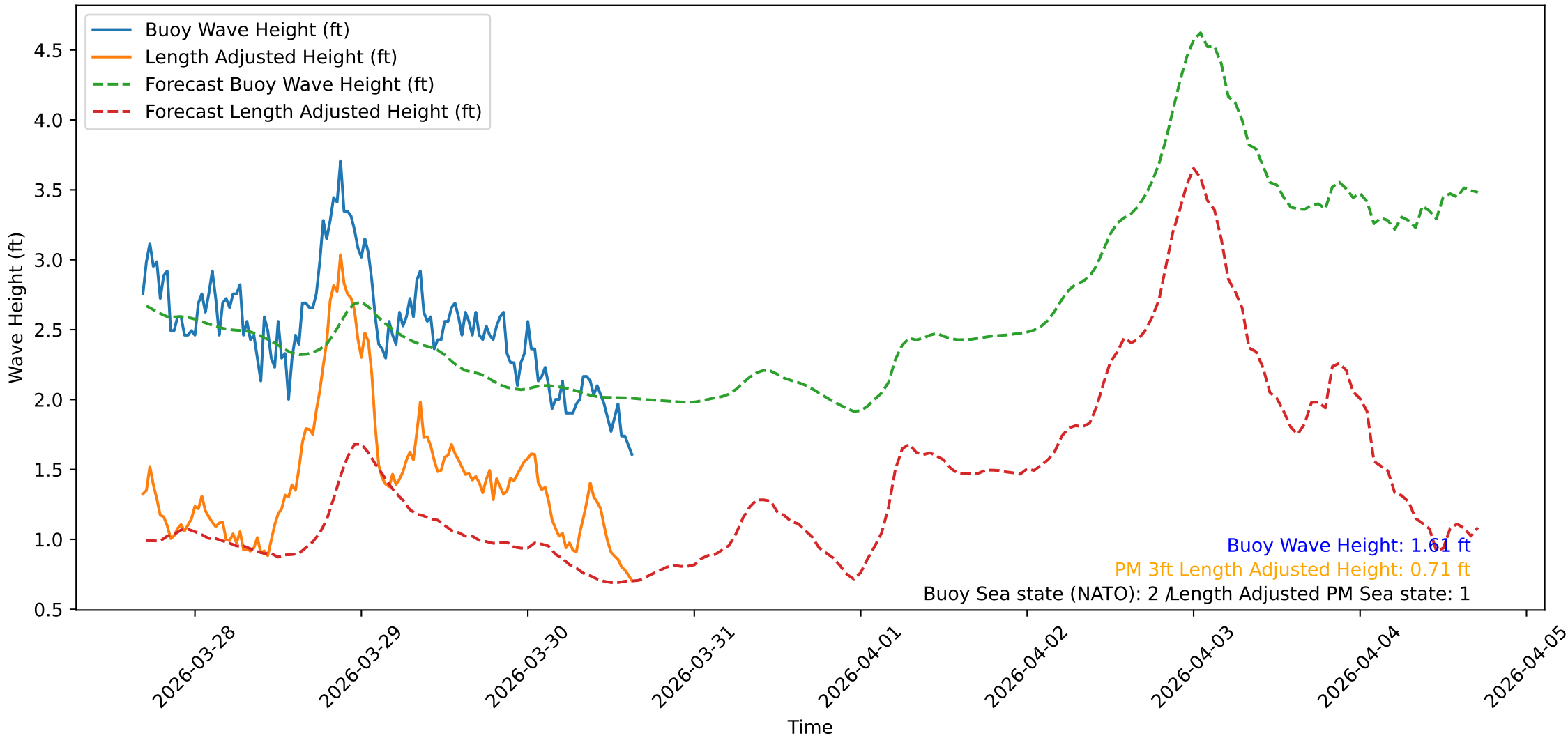
Wave Heights over Time for Green Beach at 2026-03-30 16:31:10
