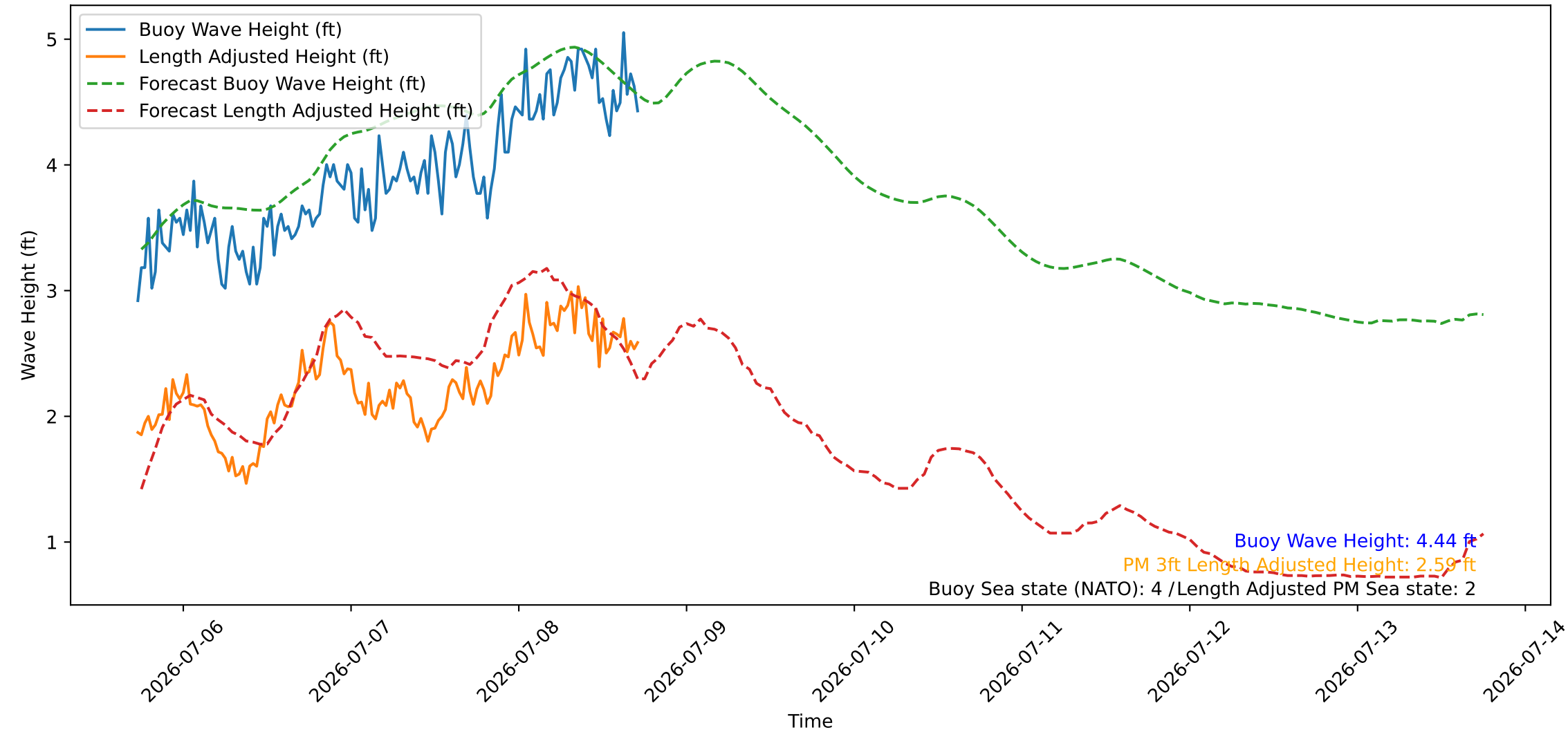
Wave Heights over Time for Oceanside Harbor at 2026-07-08 17:30:26
