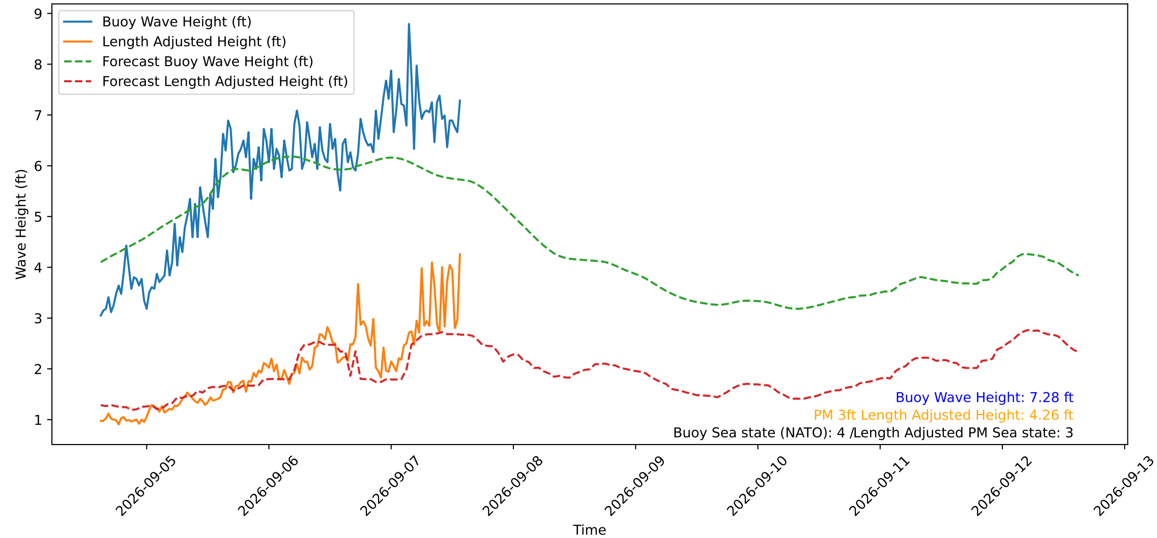
Wave Heights over Time for Green Beach at 2026-09-07 14:31:14
