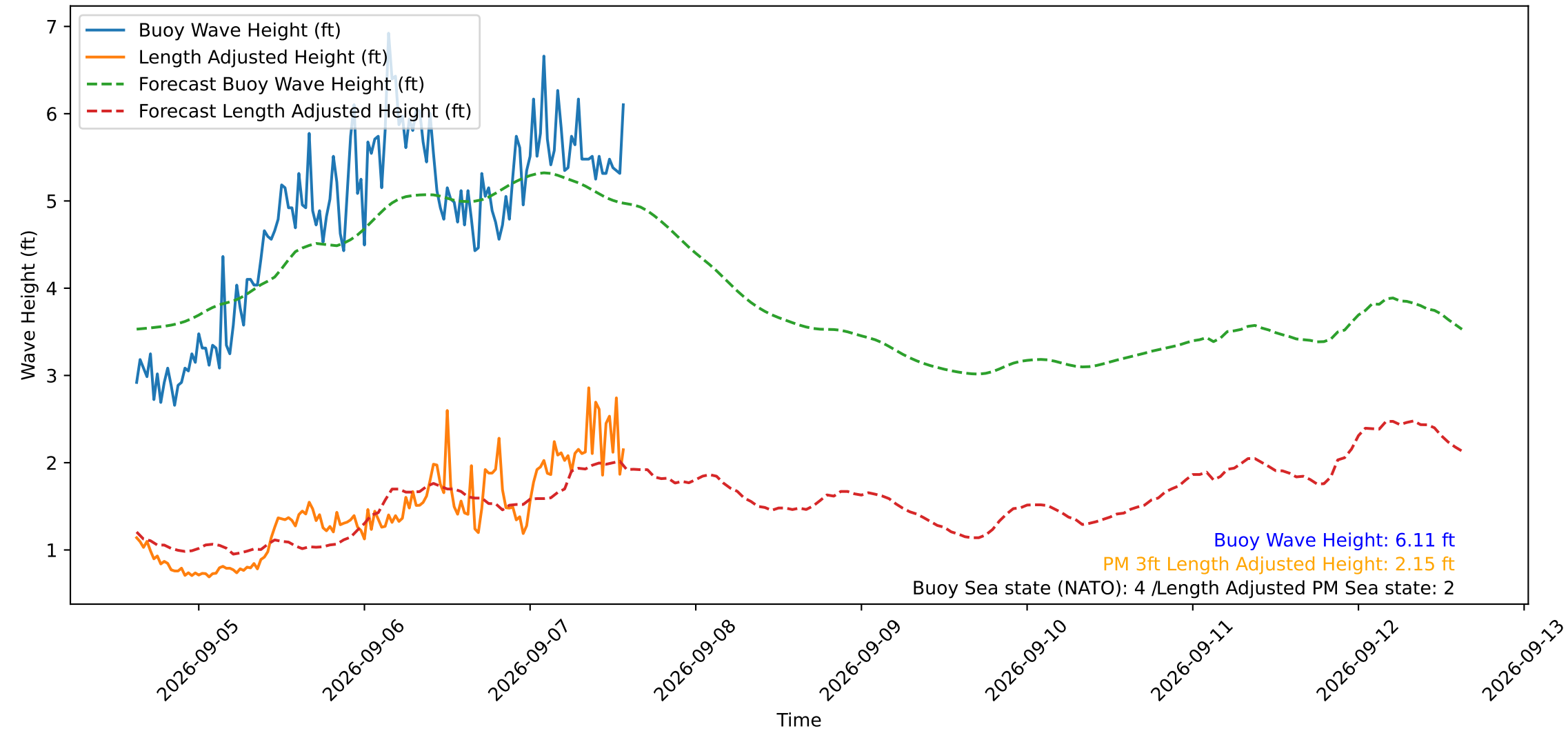
Wave Heights over Time for Red Beach at 2026-09-07 14:30:50
