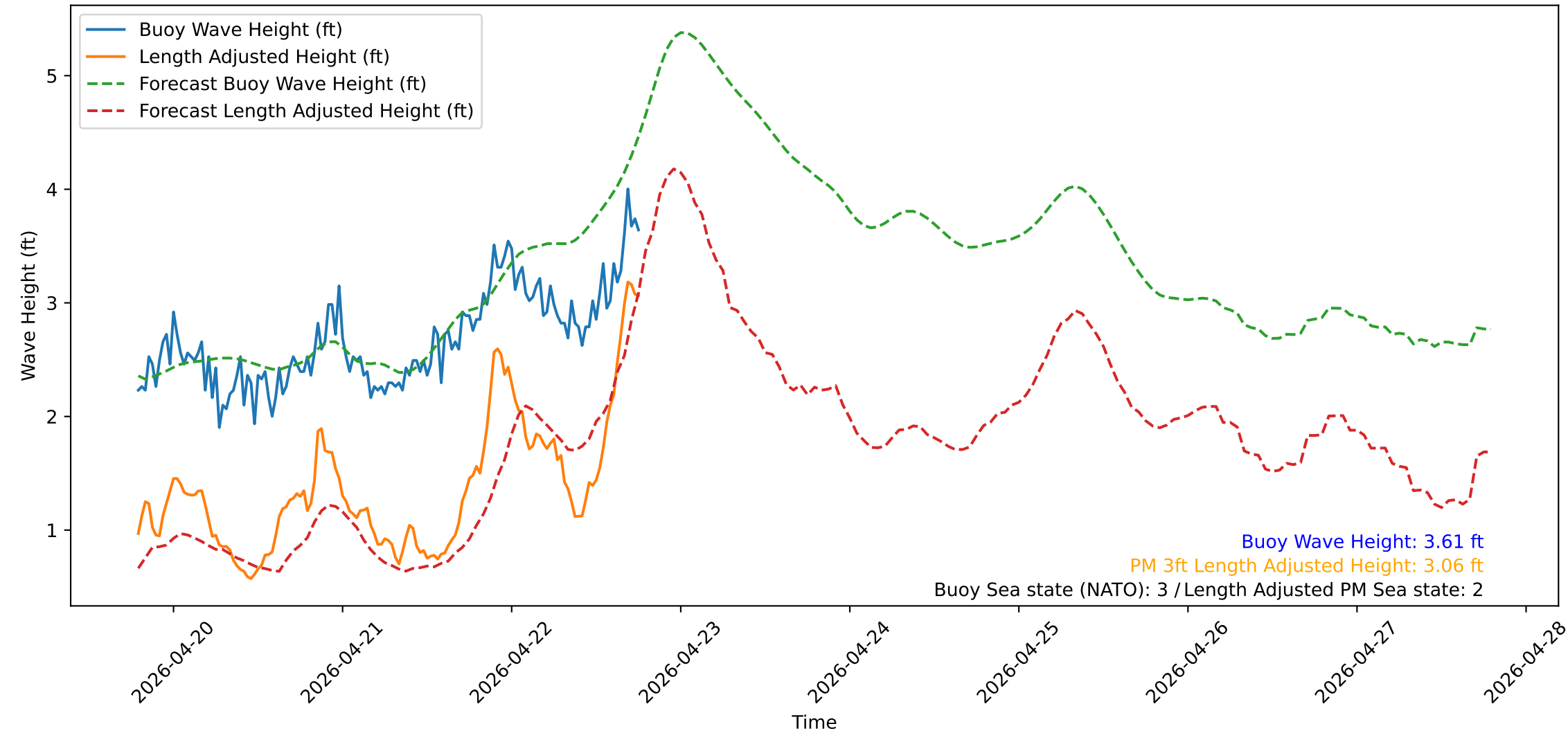
Wave Heights over Time for Green Beach at 2026-04-22 18:51:14
