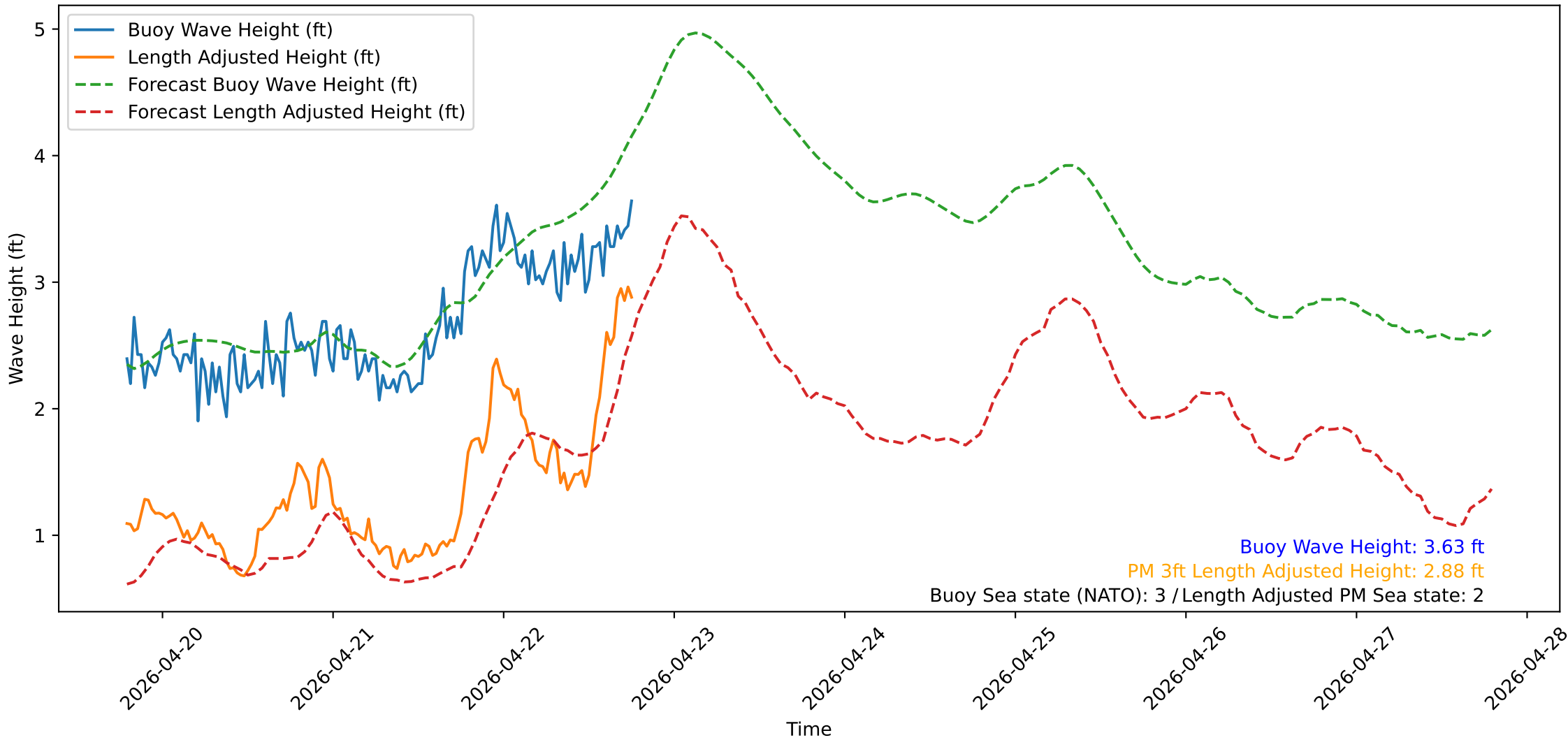
Wave Heights over Time for Oceanside Harbor at 2026-04-22 18:50:32
