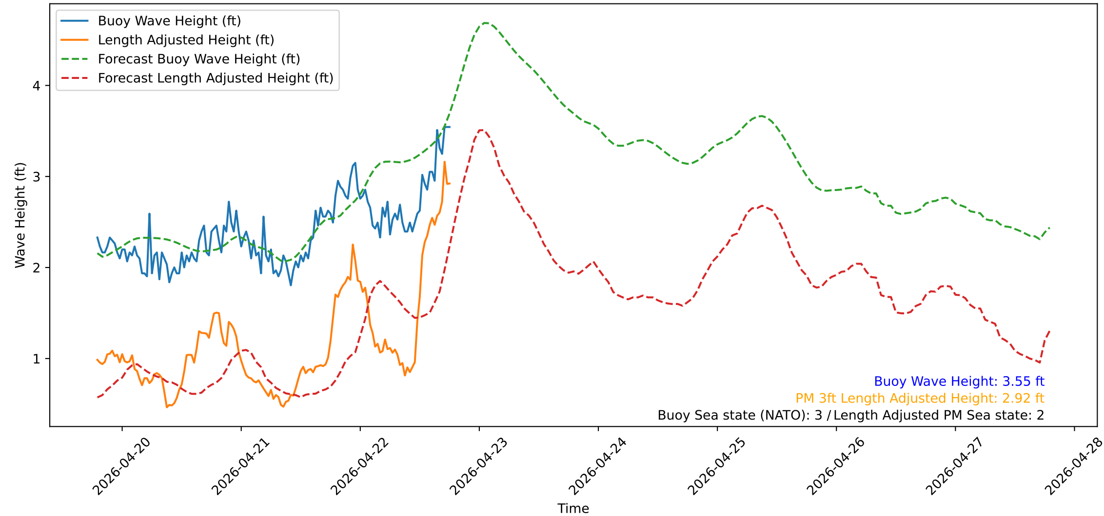
Wave Heights over Time for Red Beach at 2026-04-22 18:50:52
