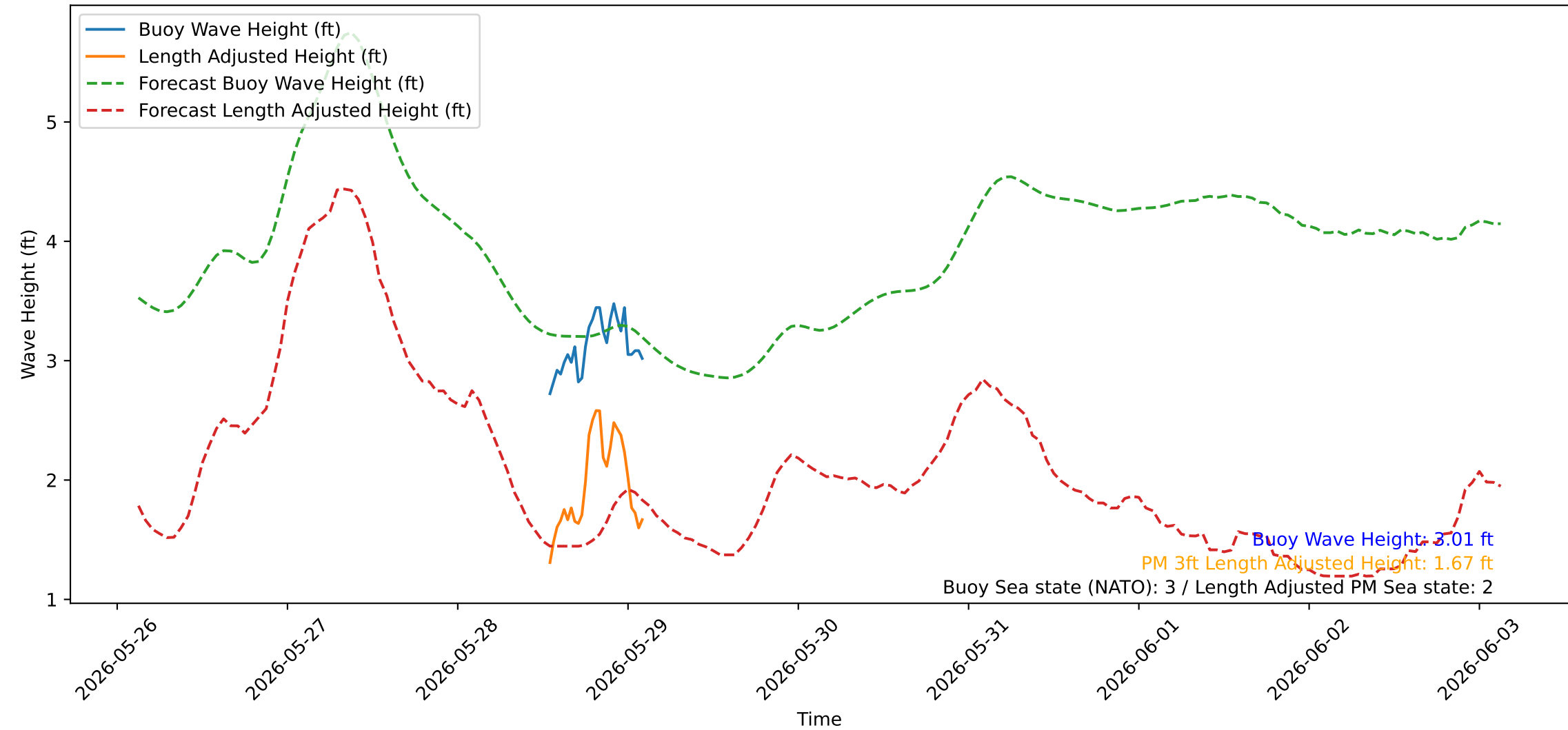
Wave Heights over Time for Oceanside Harbor at 2026-05-29 02:50:21
