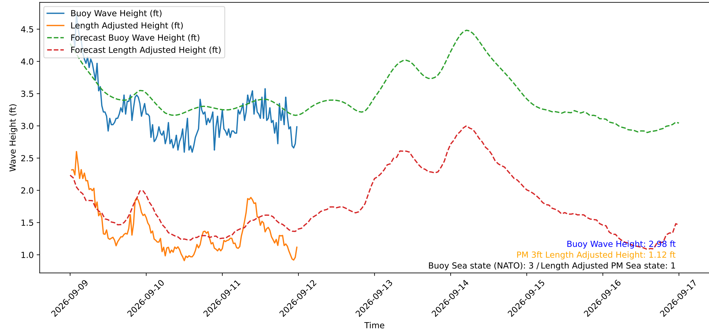
Wave Heights over Time for Green Beach at 2026-09-12 00:11:12
