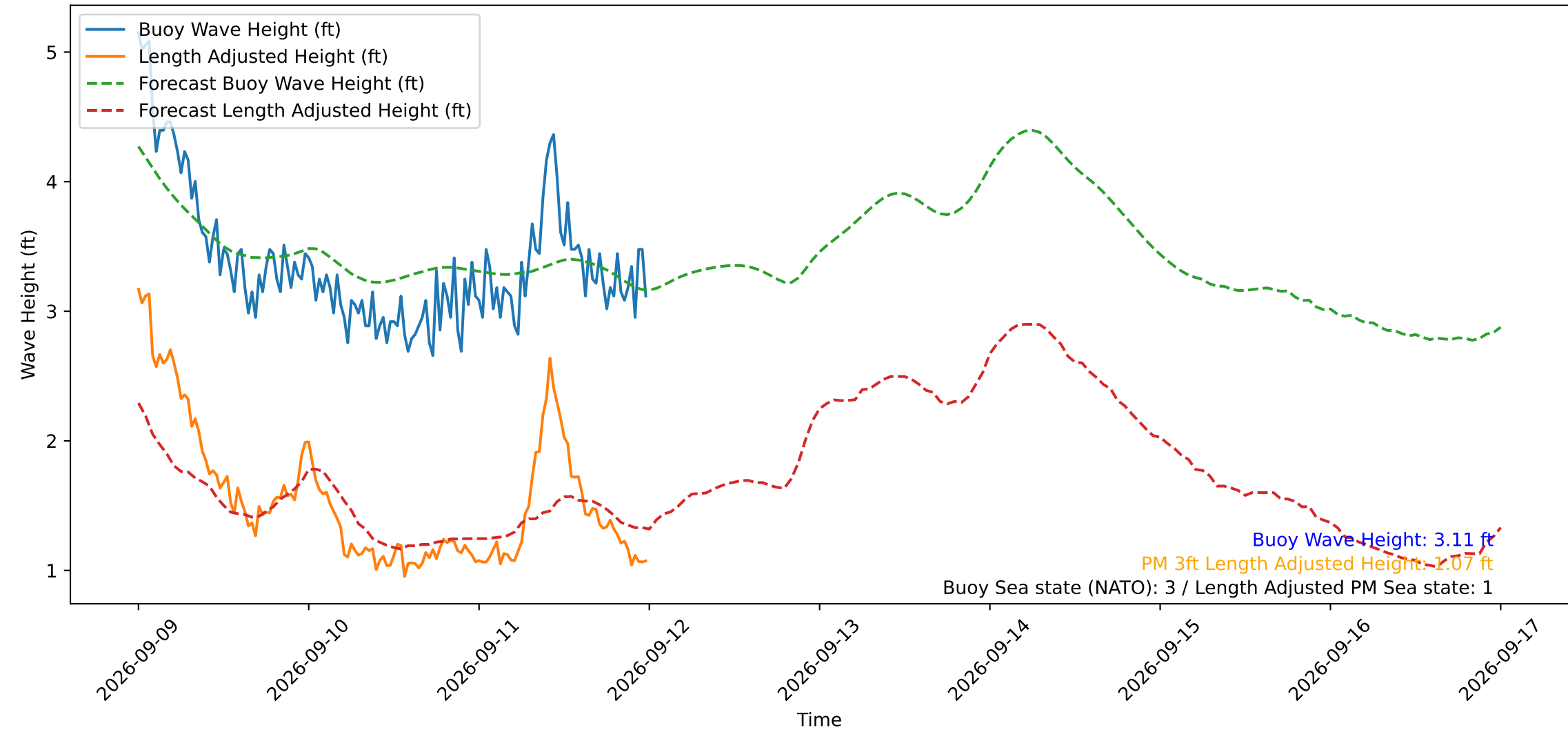
Wave Heights over Time for Oceanside Harbor at 2026-09-12 00:10:30
