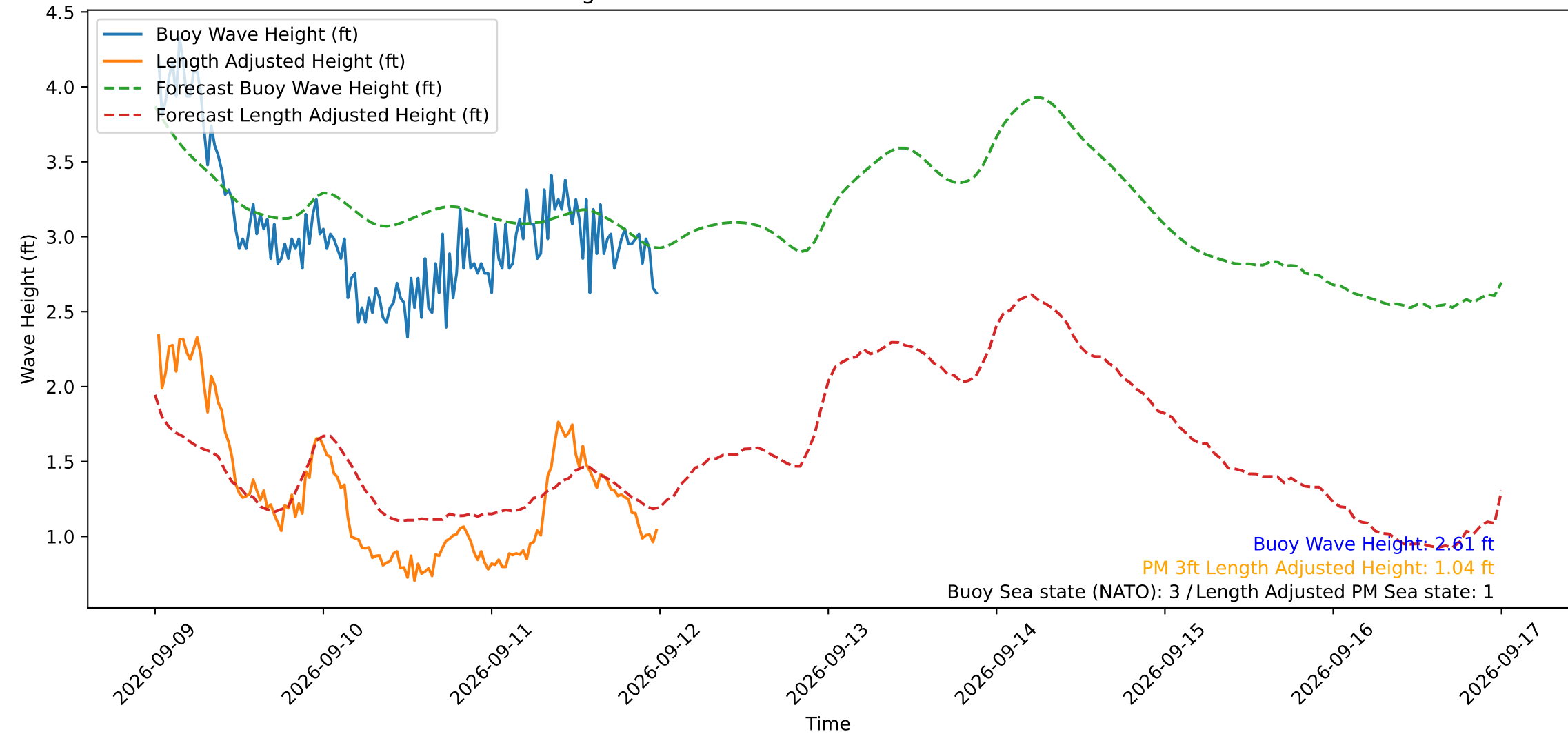
Wave Heights over Time for Red Beach at 2026-09-12 00:10:49
