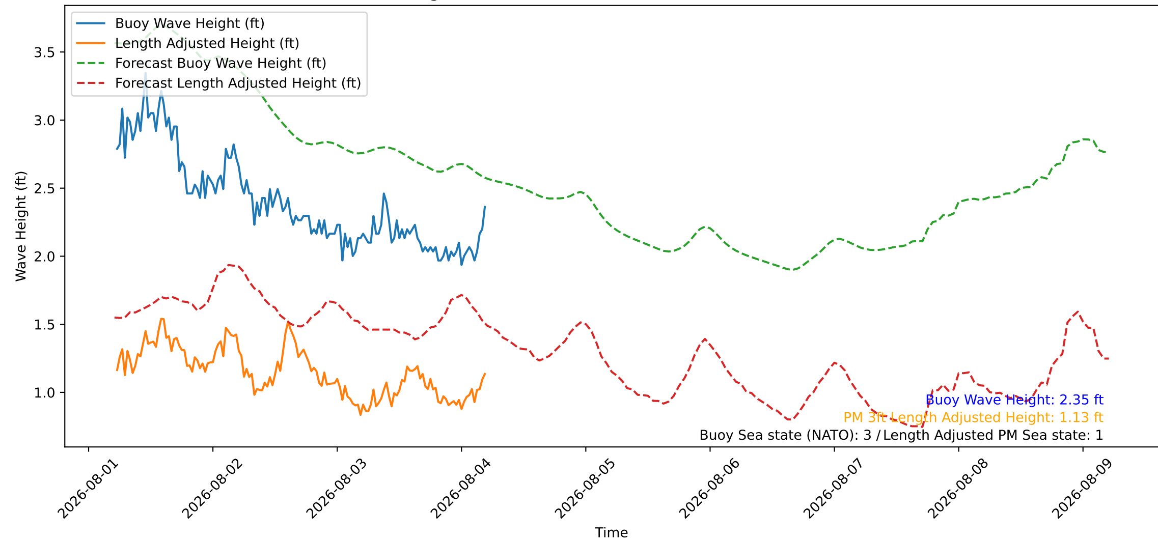
Wave Heights over Time for Red Beach at 2026-08-04 05:10:46
