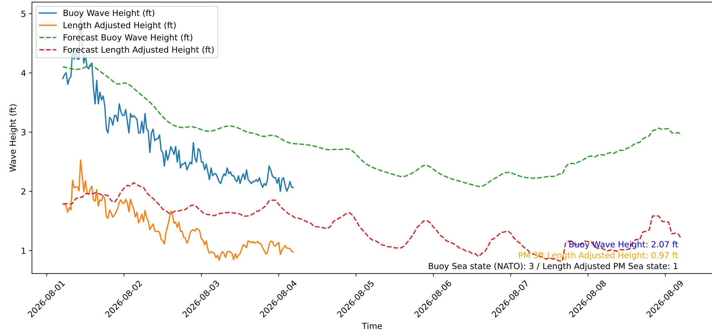
Wave Heights over Time for Green Beach at 2026-08-04 05:11:08
