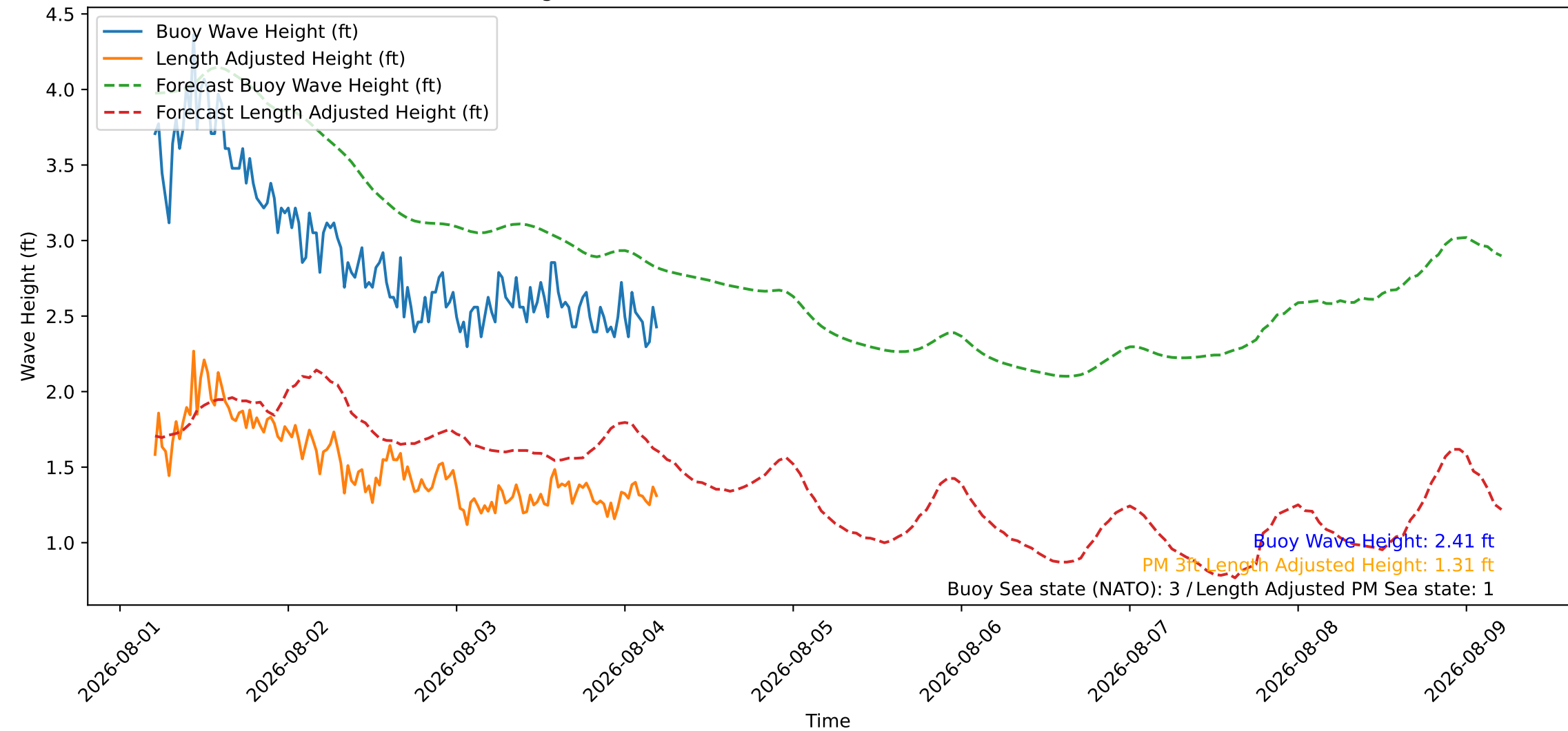
Wave Heights over Time for Oceanside Harbor at 2026-08-04 05:10:26
