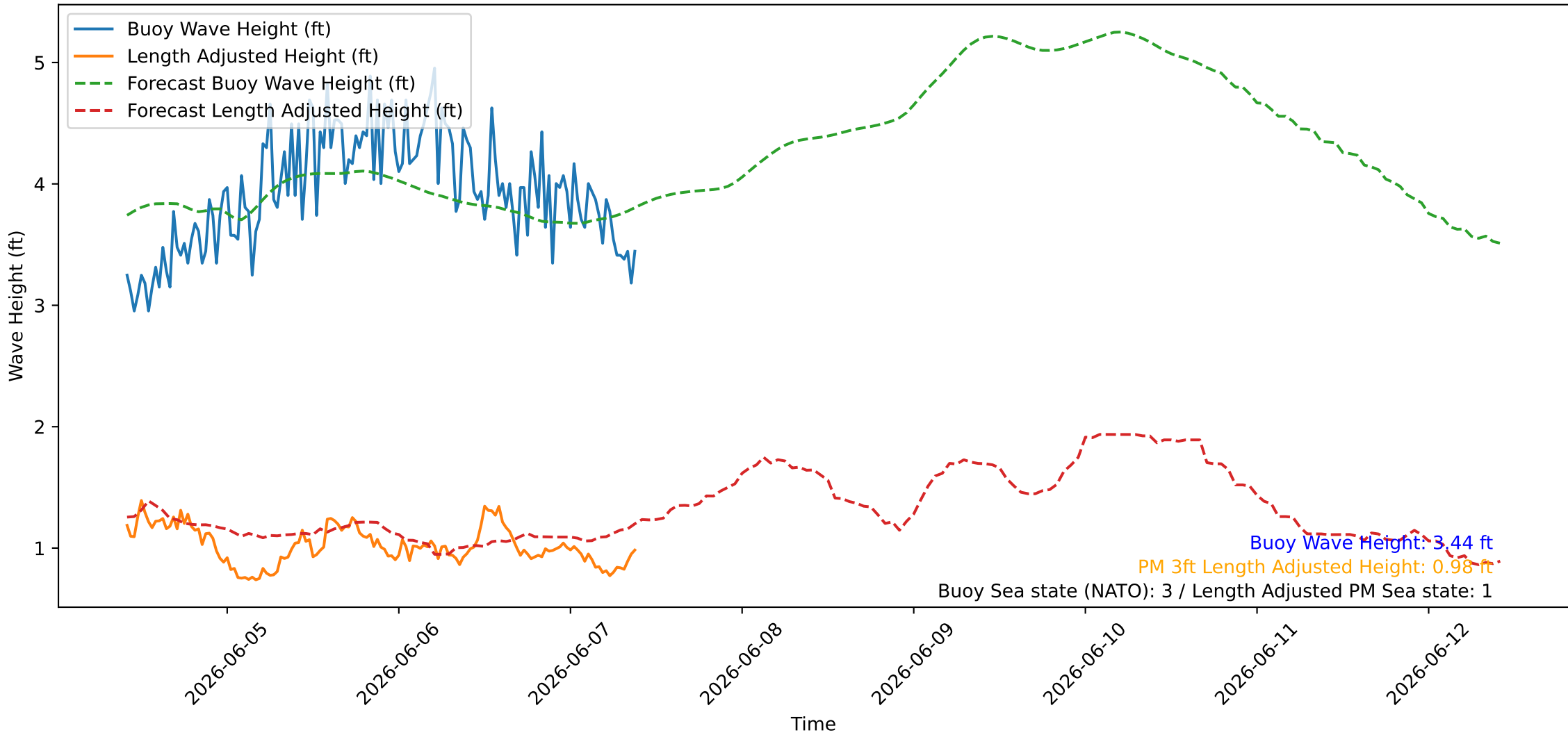
Wave Heights over Time for Red Beach at 2026-06-07 09:50:46
