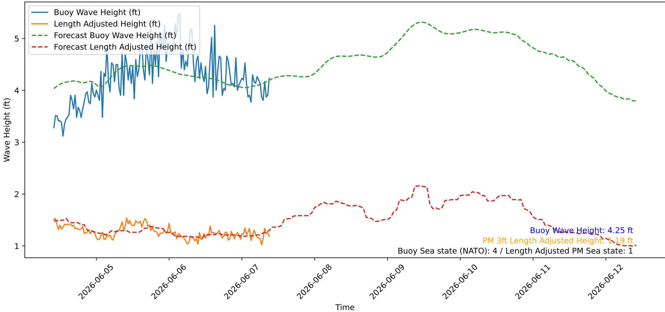
Wave Heights over Time for Oceanside Harbor at 2026-06-07 09:50:25
