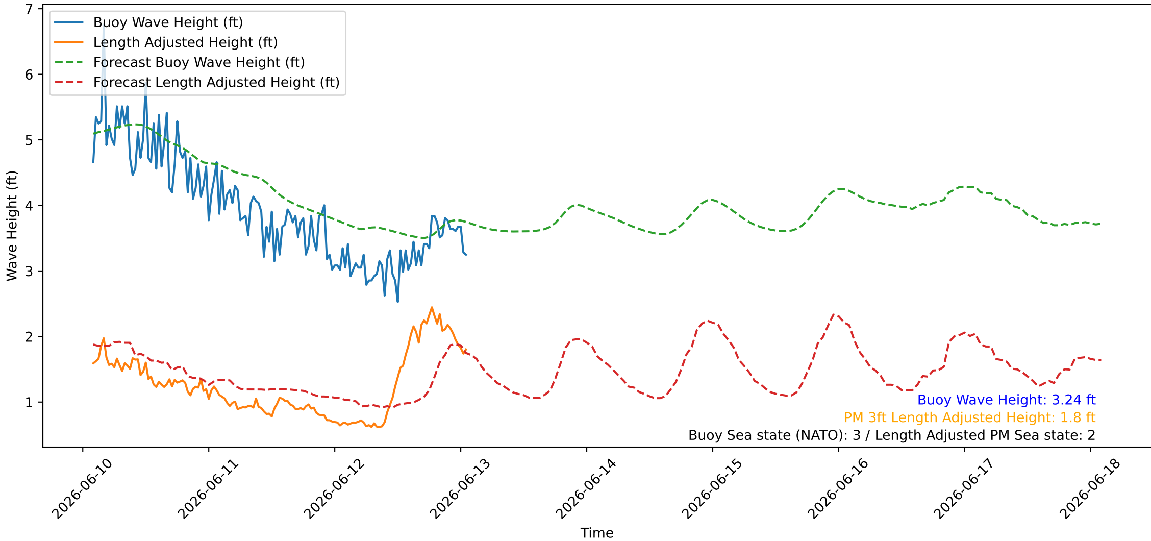
Wave Heights over Time for Red Beach at 2026-06-13 01:40:46
