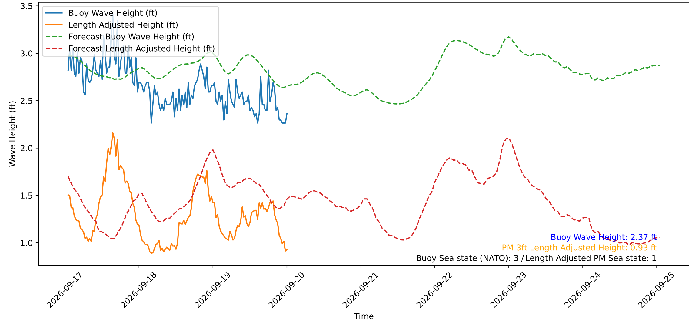
Wave Heights over Time for Red Beach at 2026-09-20 00:40:48
