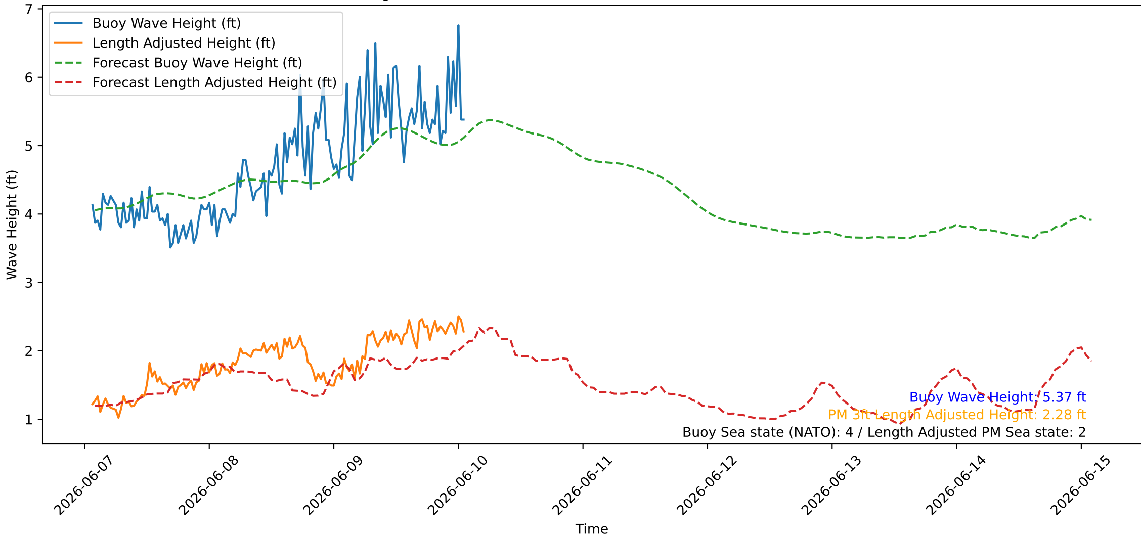
Wave Heights over Time for Oceanside Harbor at 2026-06-10 01:30:26
