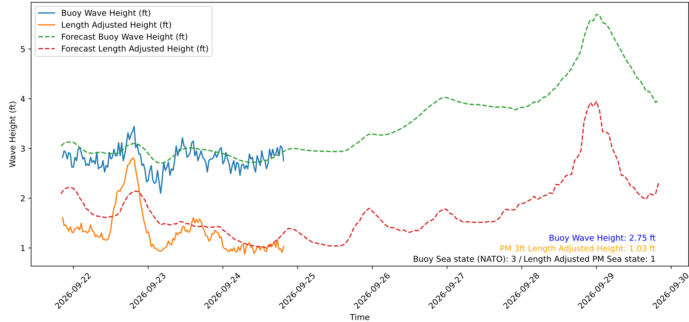
Wave Heights over Time for Green Beach at 2026-09-24 20:21:15
