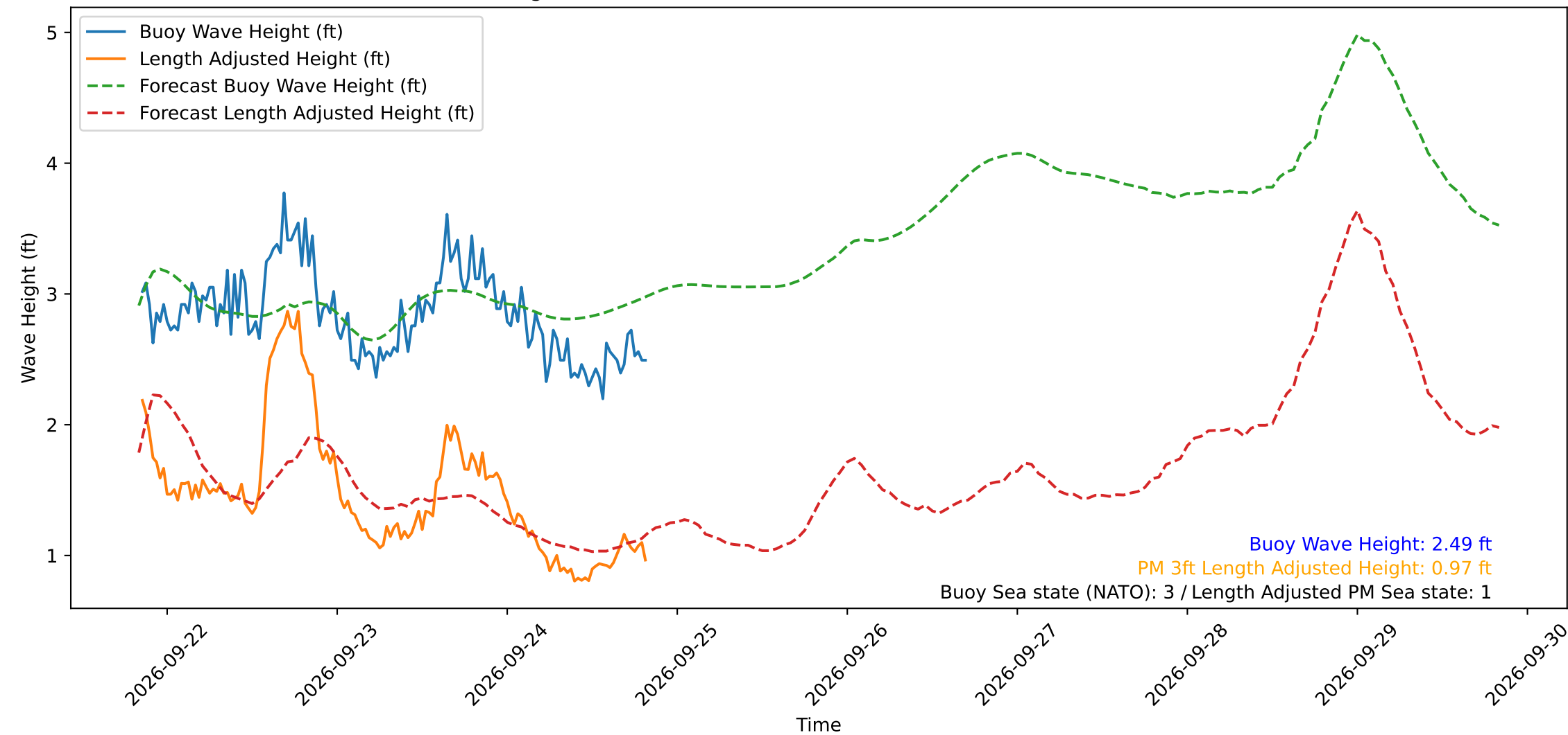
Wave Heights over Time for Oceanside Harbor at 2026-09-24 20:20:29
