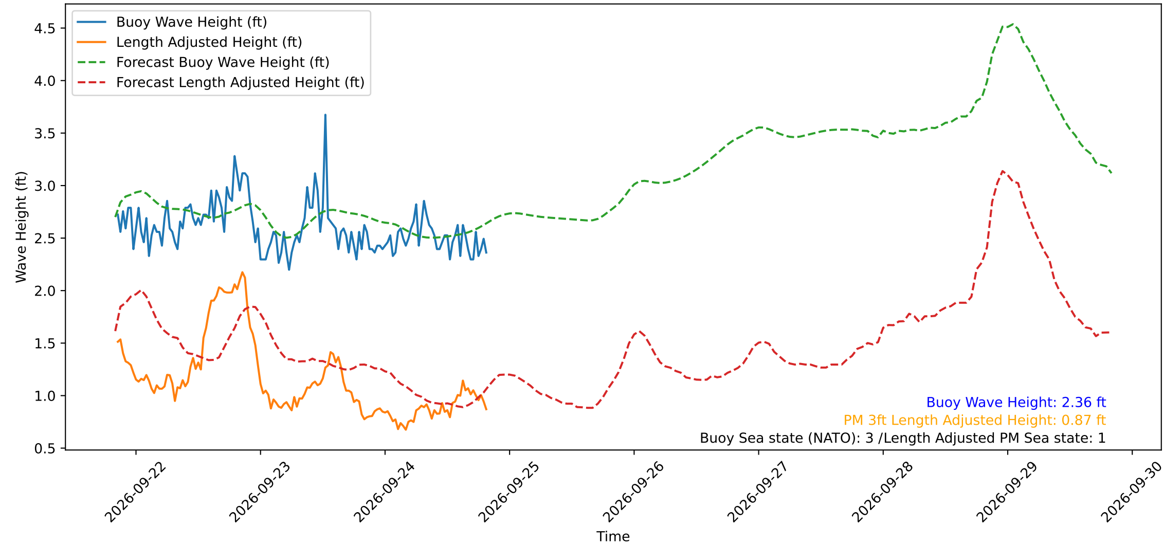
Wave Heights over Time for Red Beach at 2026-09-24 20:20:50
