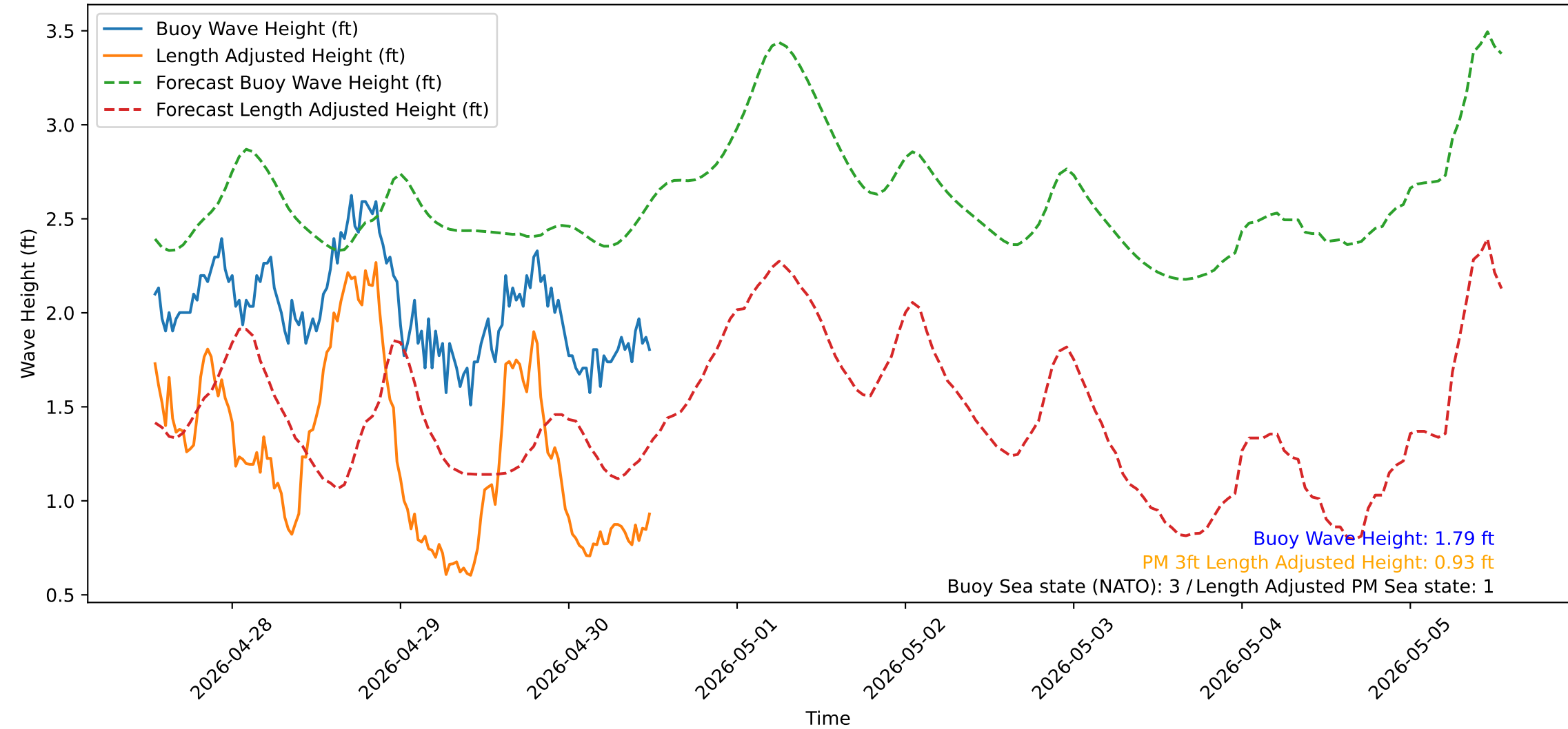
Wave Heights over Time for Red Beach at 2026-04-30 12:30:52
