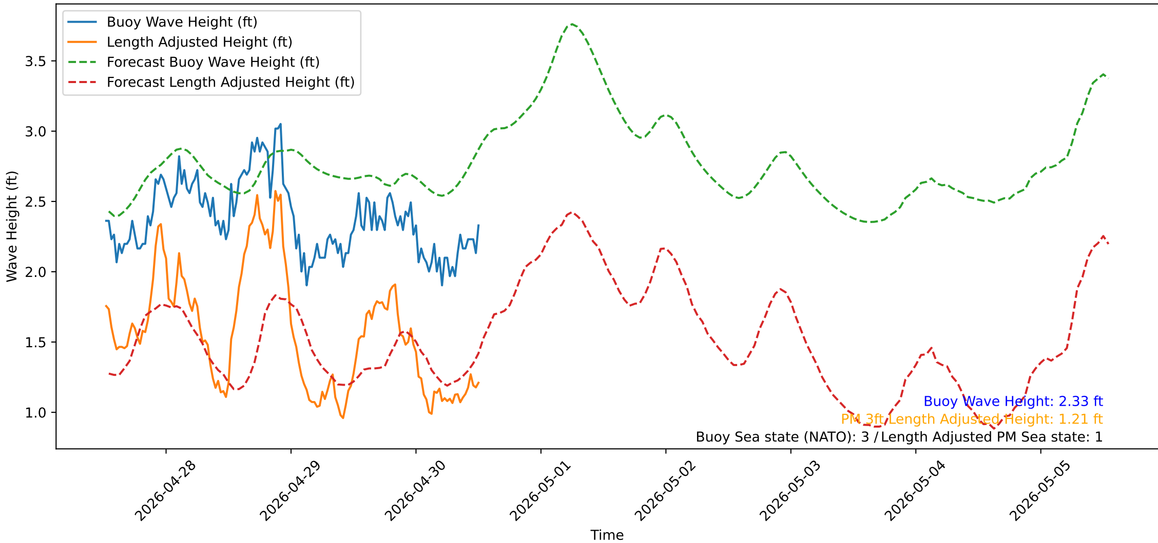
Wave Heights over Time for Oceanside Harbor at 2026-04-30 12:30:32
