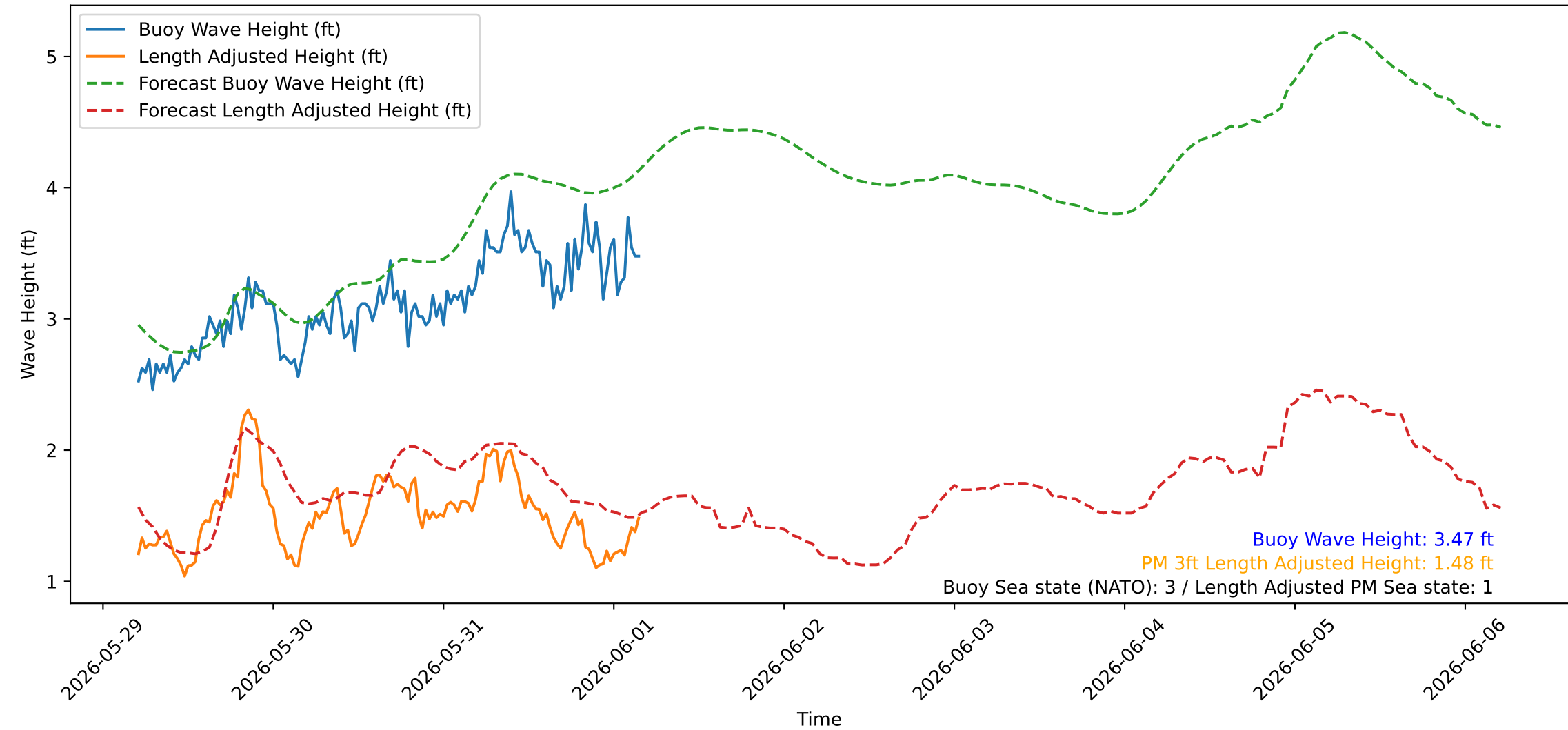
Wave Heights over Time for Green Beach at 2026-06-01 05:01:08
