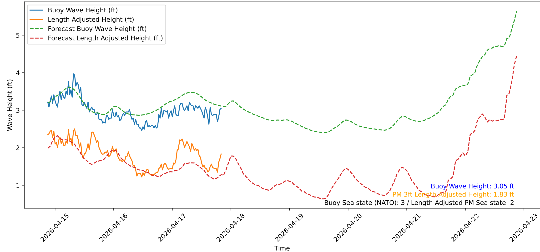
Wave Heights over Time for Green Beach at 2026-04-17 21:01:13
