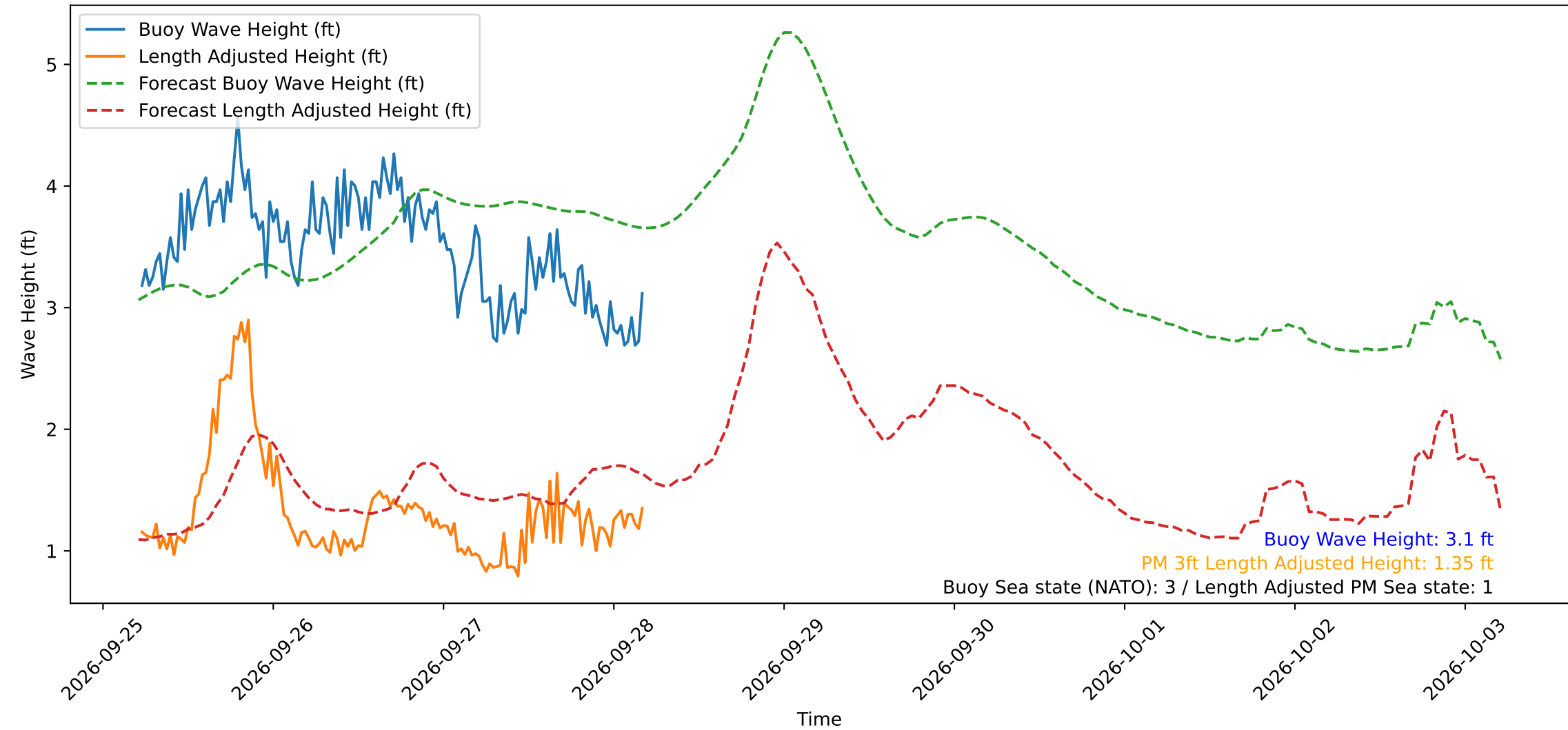
Wave Heights over Time for Green Beach at 2026-09-28 05:01:13
