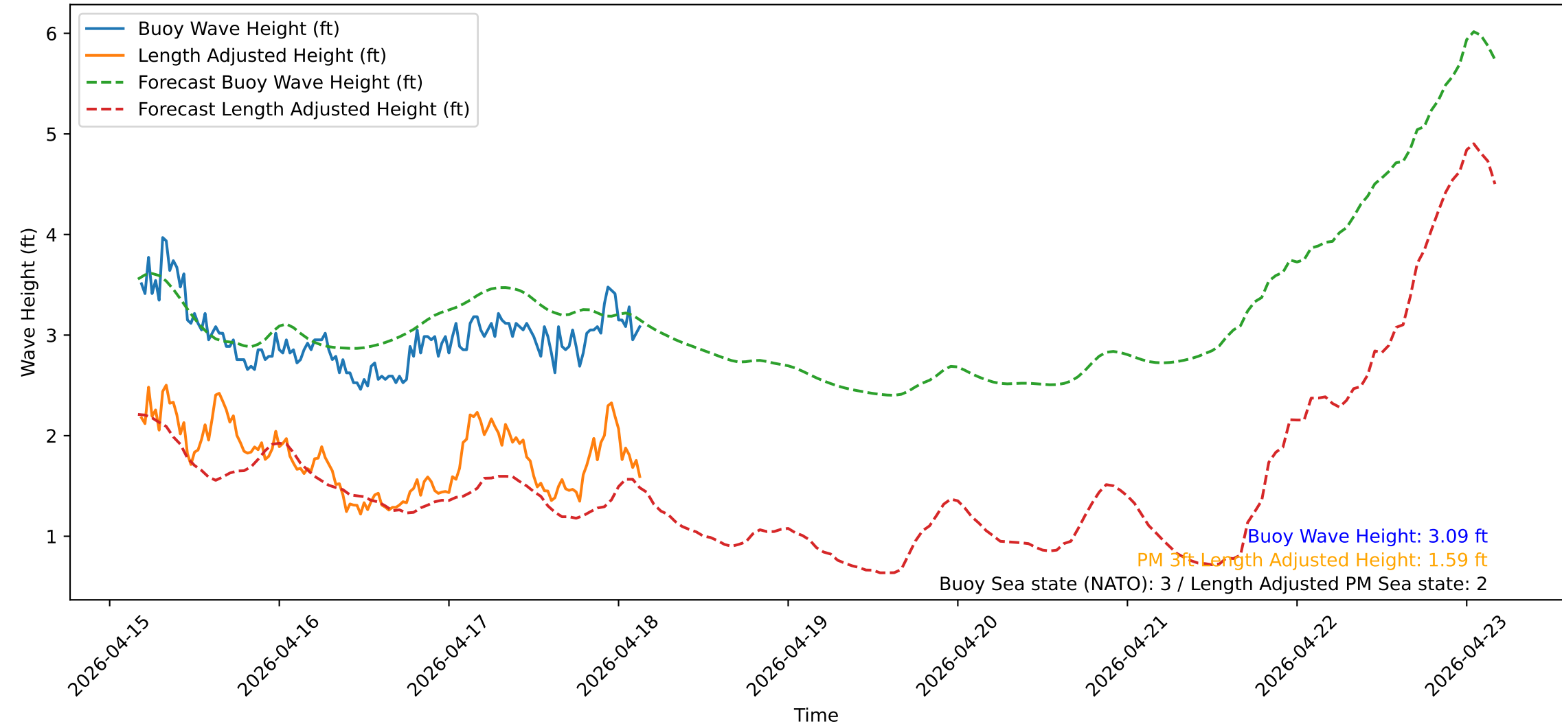
Wave Heights over Time for Green Beach at 2026-04-18 04:21:13
