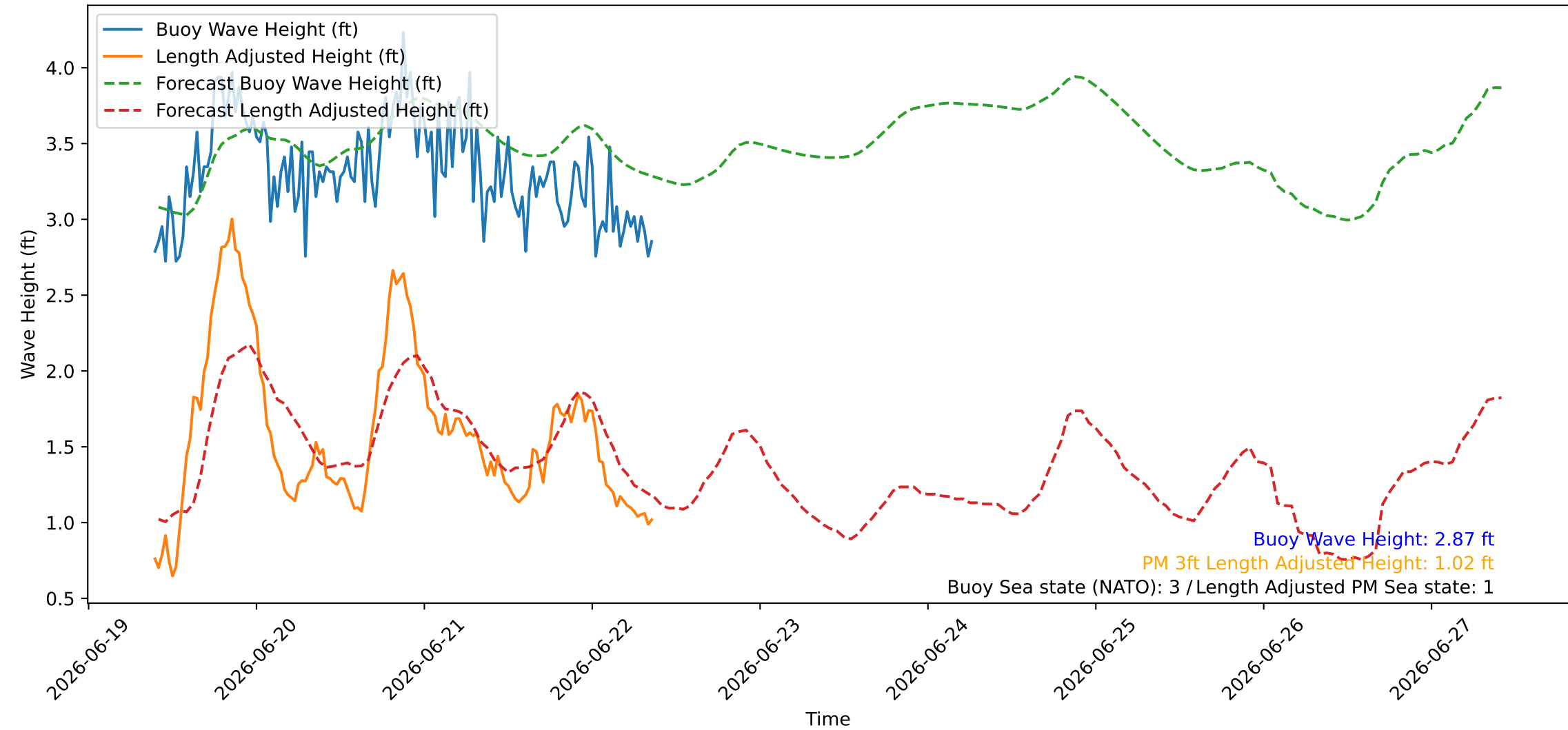
Wave Heights over Time for Green Beach at 2026-06-22 09:31:08
