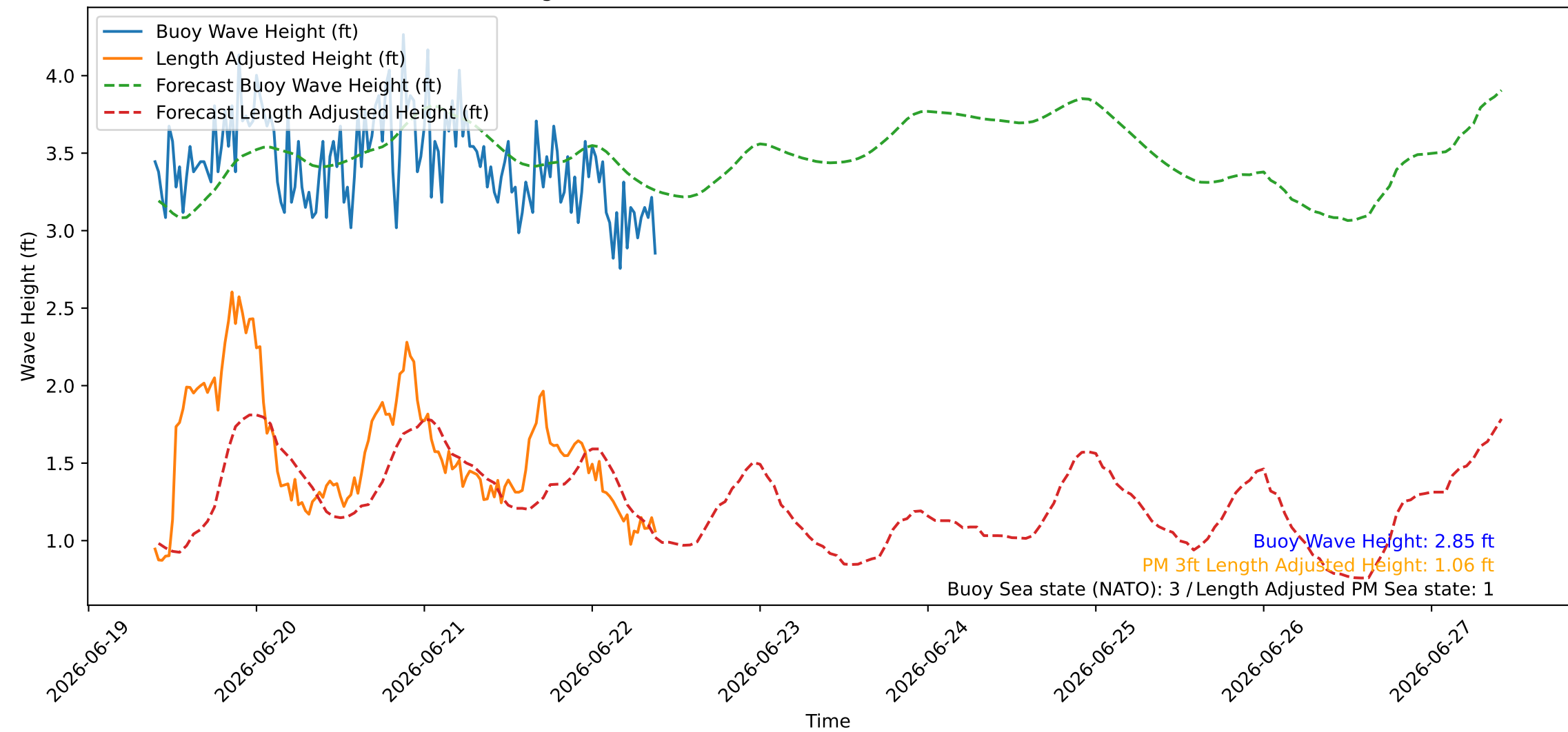
Wave Heights over Time for Oceanside Harbor at 2026-06-22 09:30:26
