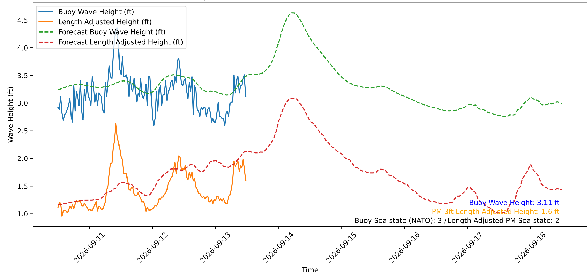
Wave Heights over Time for Oceanside Harbor at 2026-09-13 12:10:30
