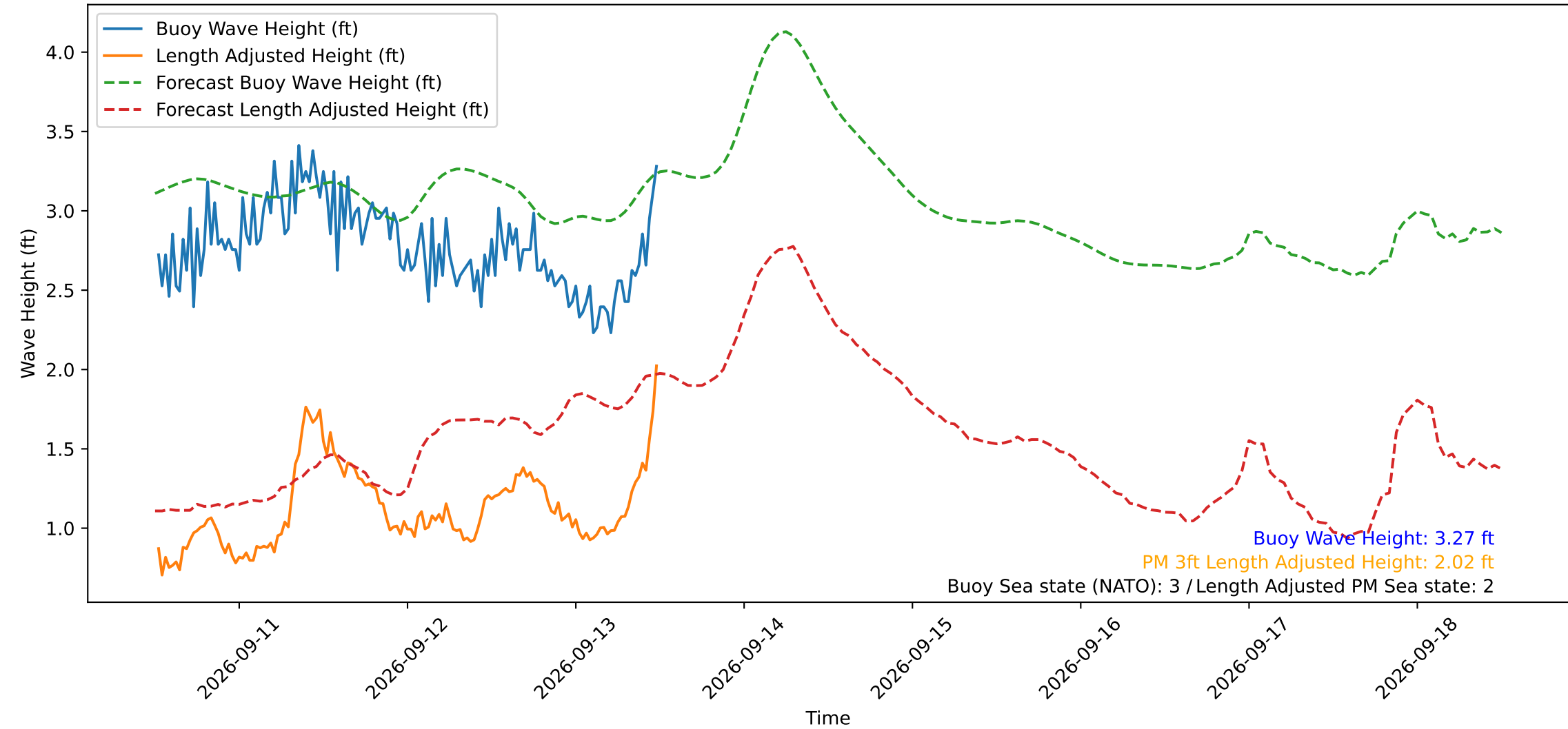
Wave Heights over Time for Red Beach at 2026-09-13 12:10:50
