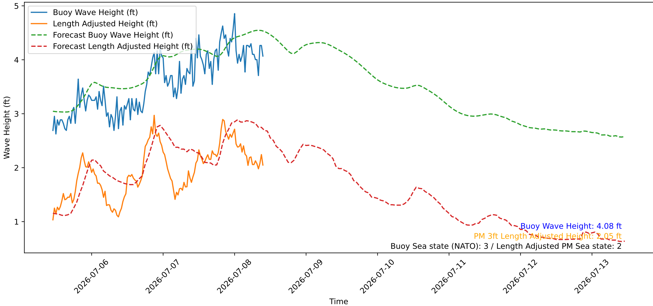
Wave Heights over Time for Red Beach at 2026-07-08 10:50:47
