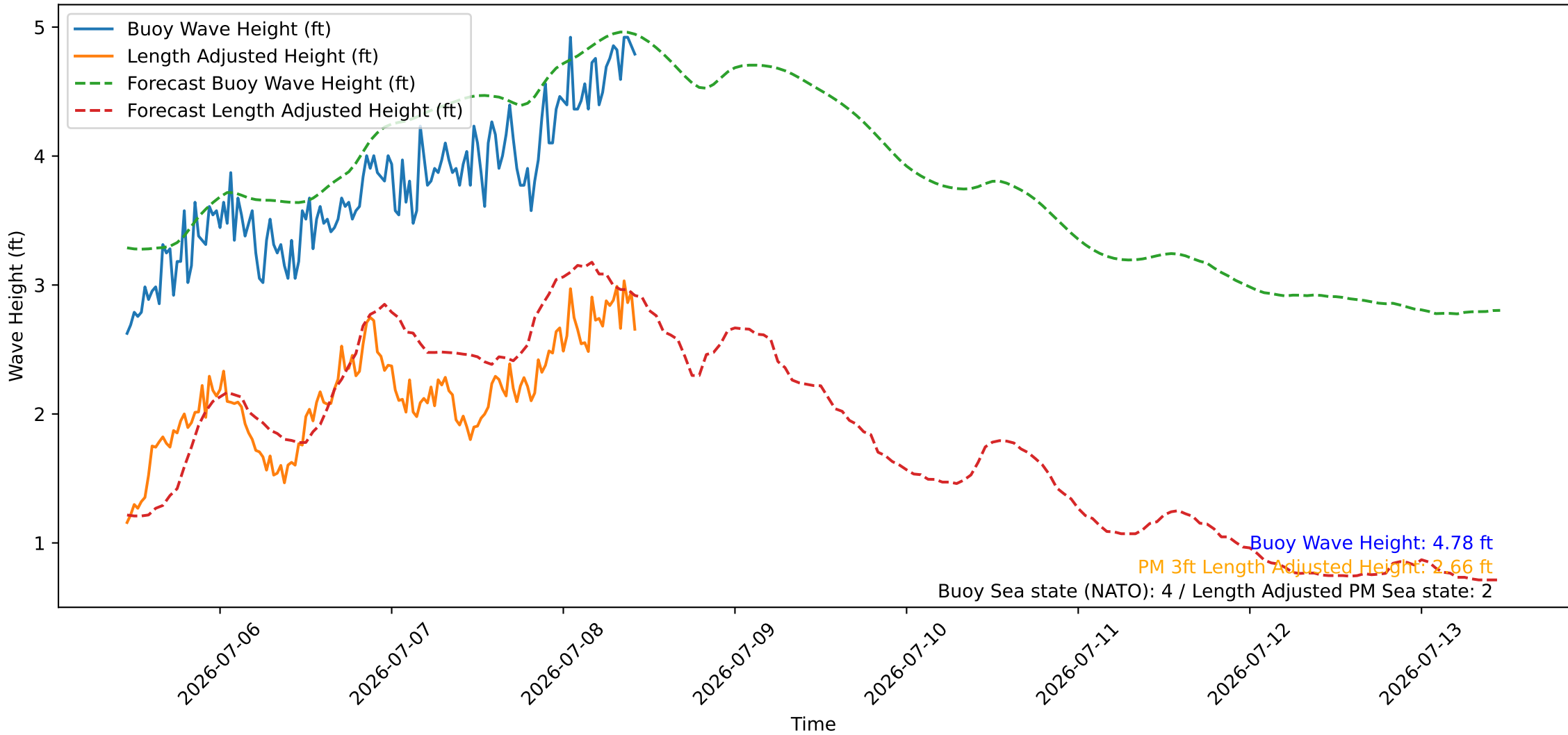
Wave Heights over Time for Oceanside Harbor at 2026-07-08 10:50:26
