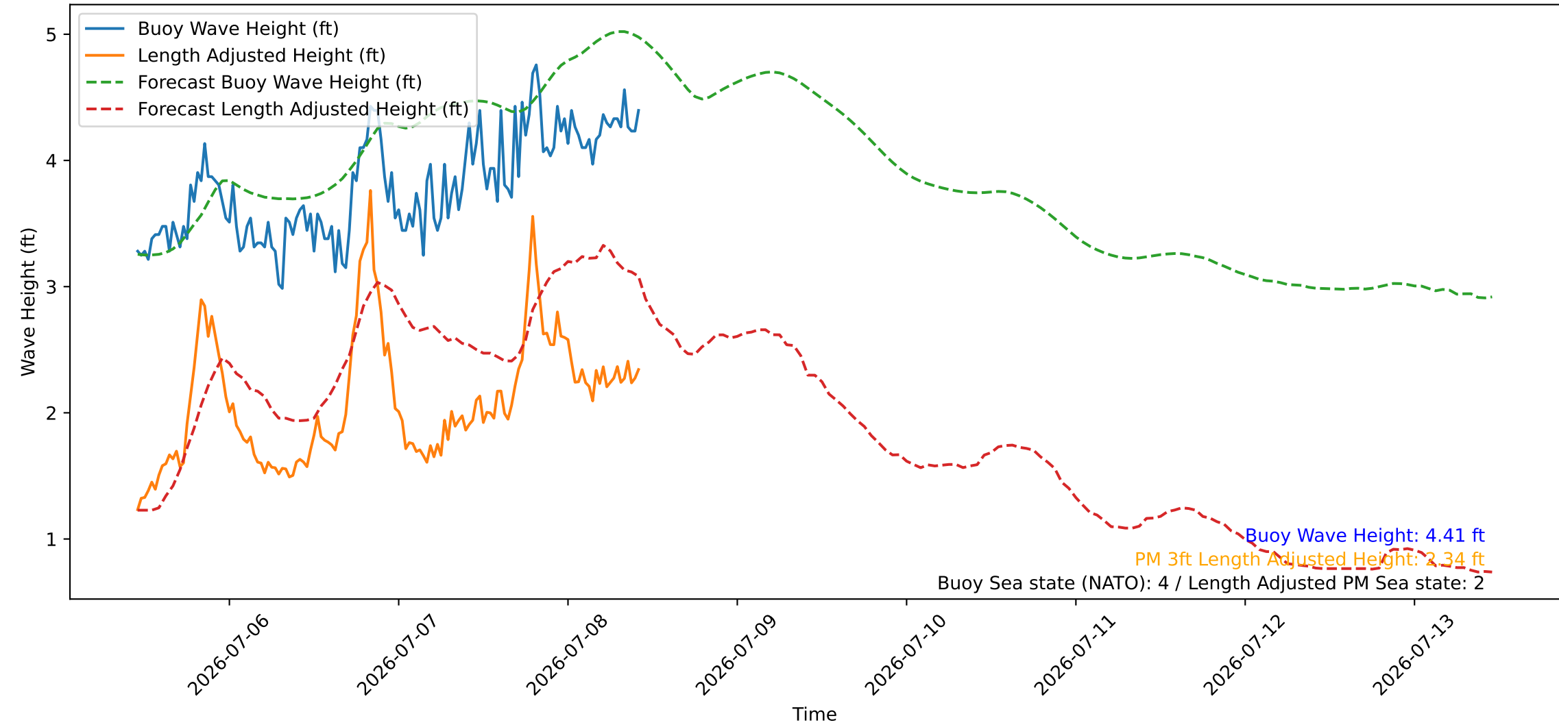
Wave Heights over Time for Green Beach at 2026-07-08 10:51:09
