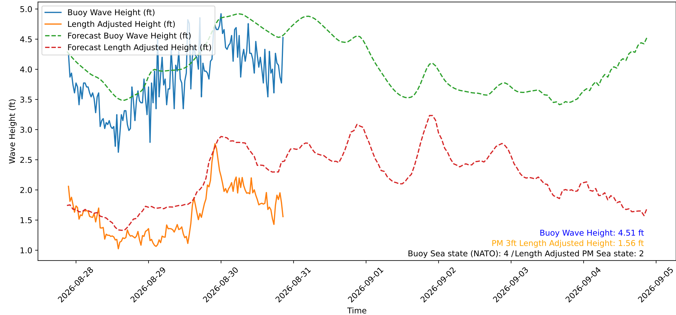
Wave Heights over Time for Green Beach at 2026-08-30 21:11:12
