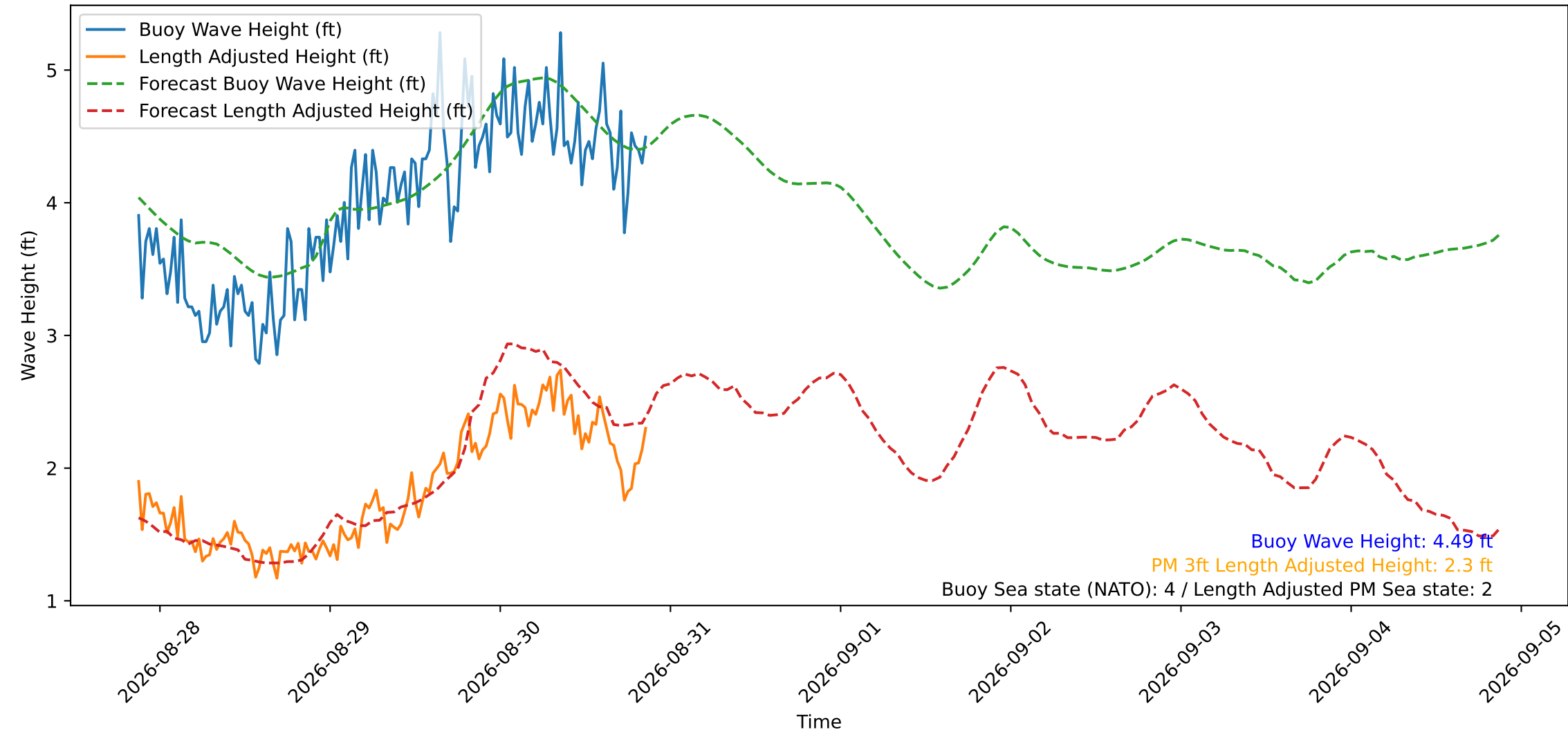
Wave Heights over Time for Oceanside Harbor at 2026-08-30 21:10:30
