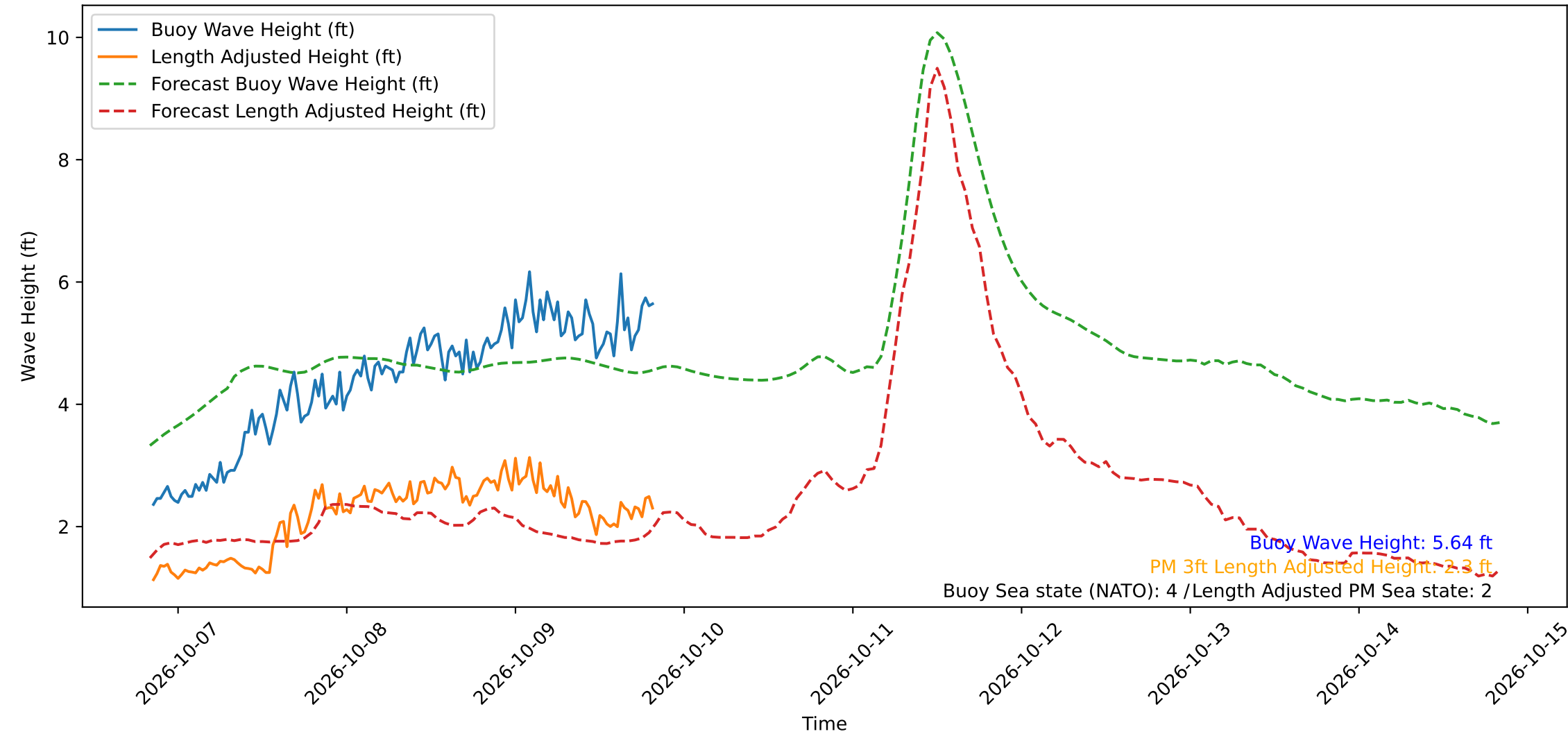
Wave Heights over Time for Green Beach at 2026-10-09 20:11:11
