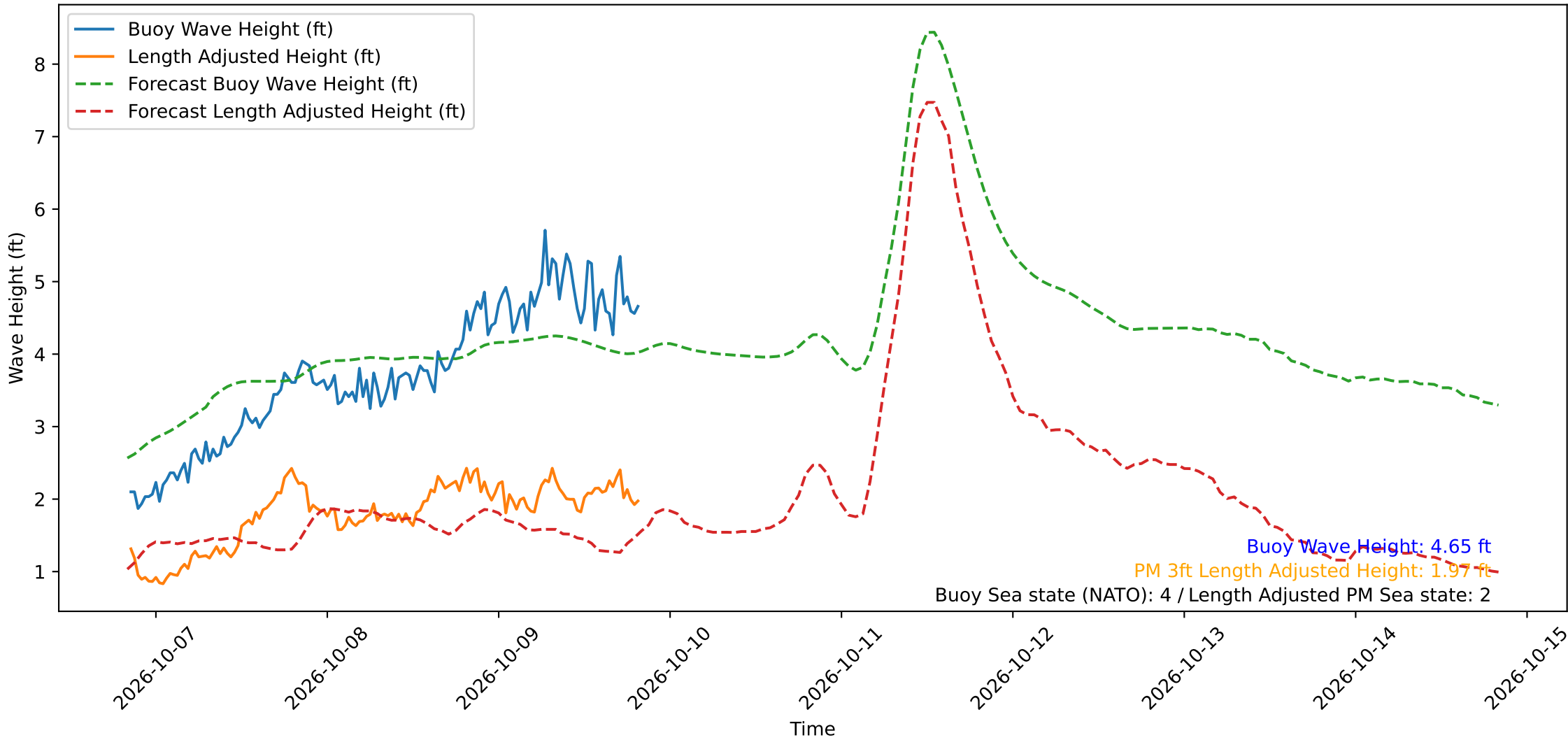
Wave Heights over Time for Red Beach at 2026-10-09 20:10:49
