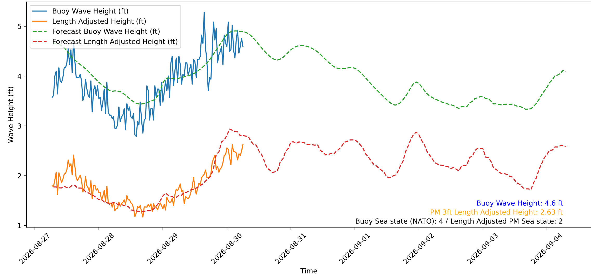
Wave Heights over Time for Oceanside Harbor at 2026-08-30 06:40:29
