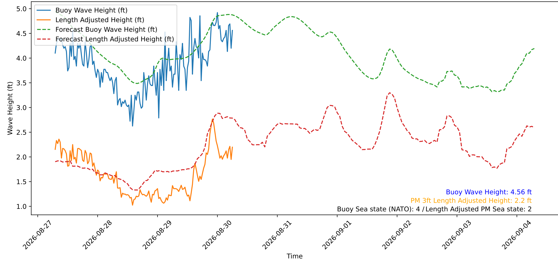
Wave Heights over Time for Green Beach at 2026-08-30 06:41:12
