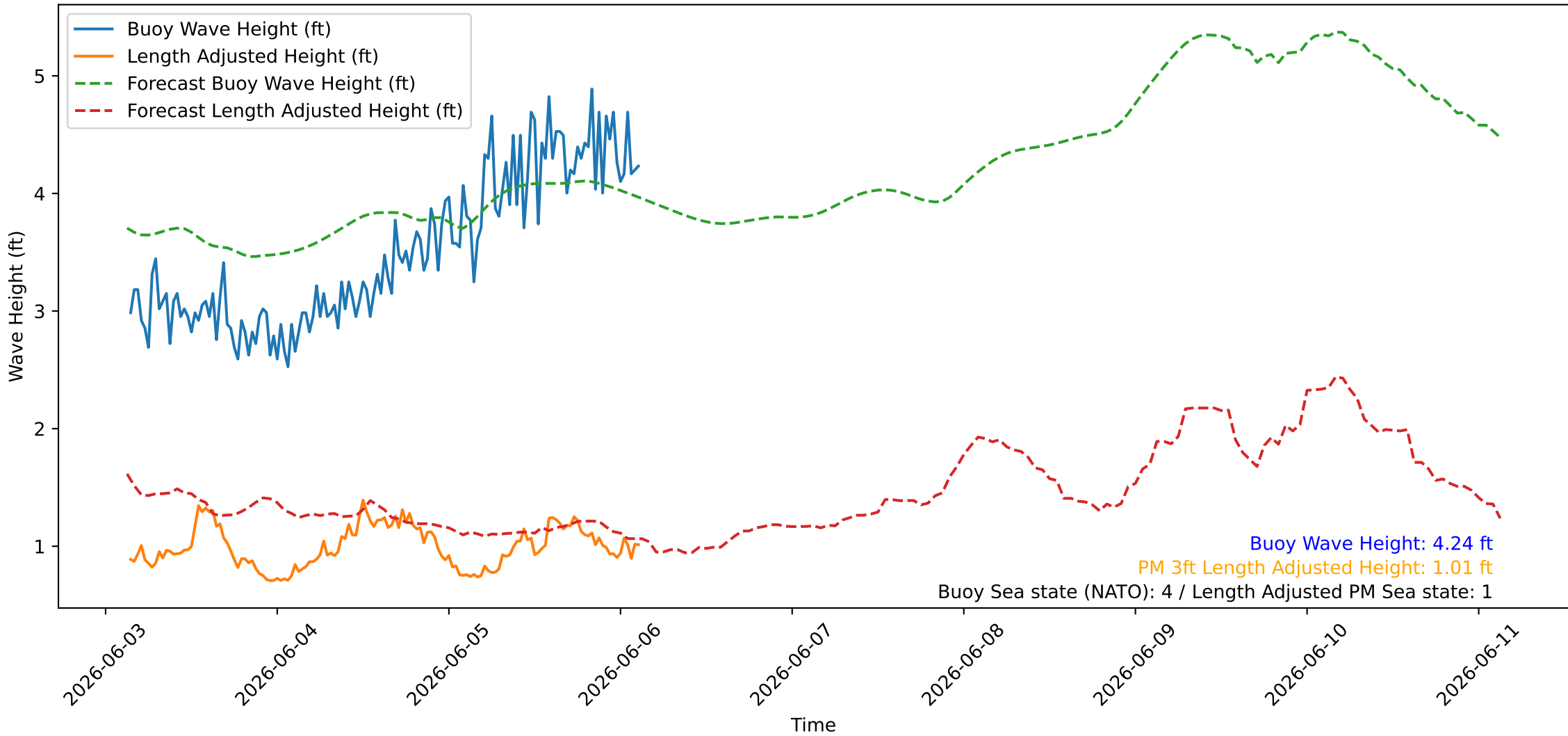
Wave Heights over Time for Red Beach at 2026-06-06 03:10:45
