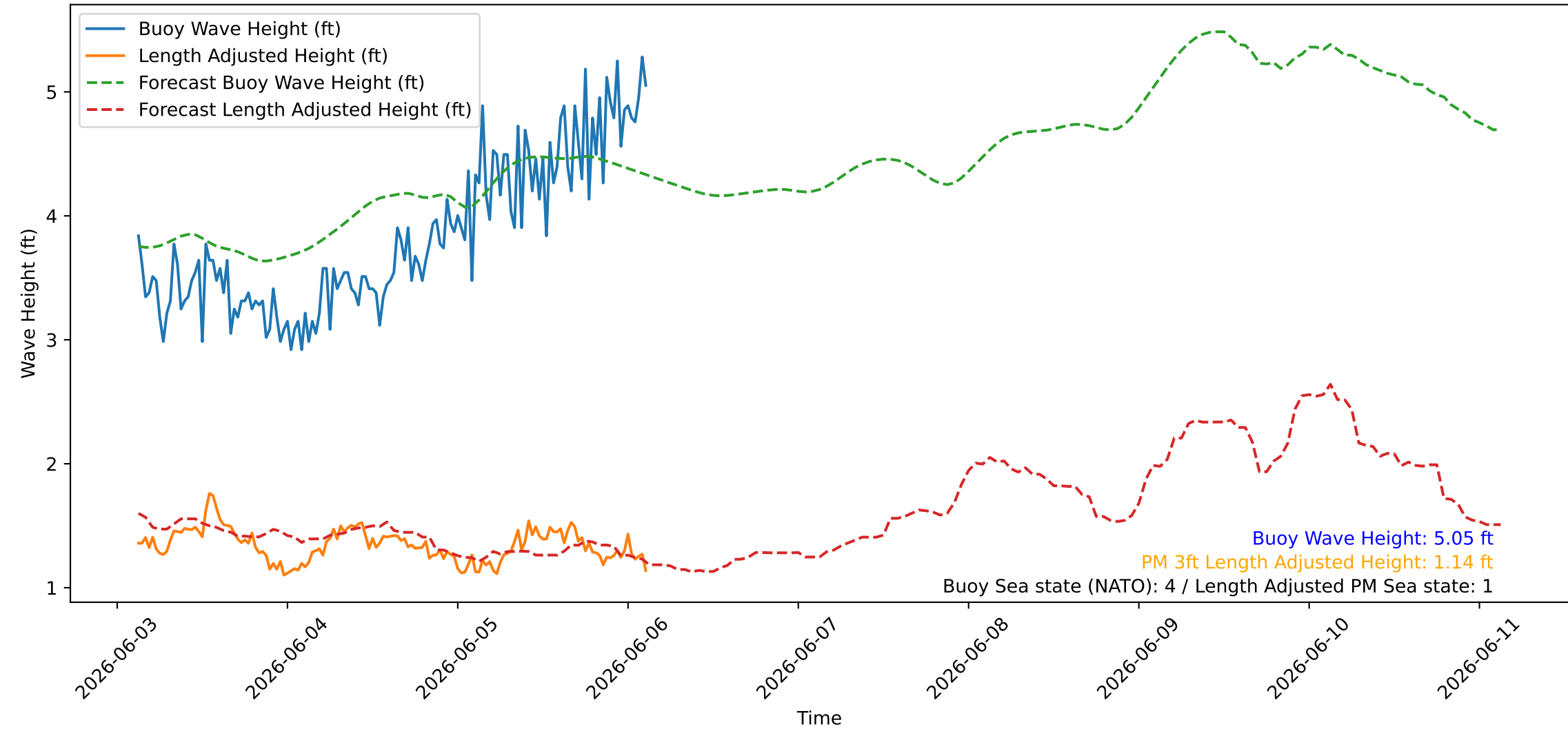
Wave Heights over Time for Oceanside Harbor at 2026-06-06 03:10:26
