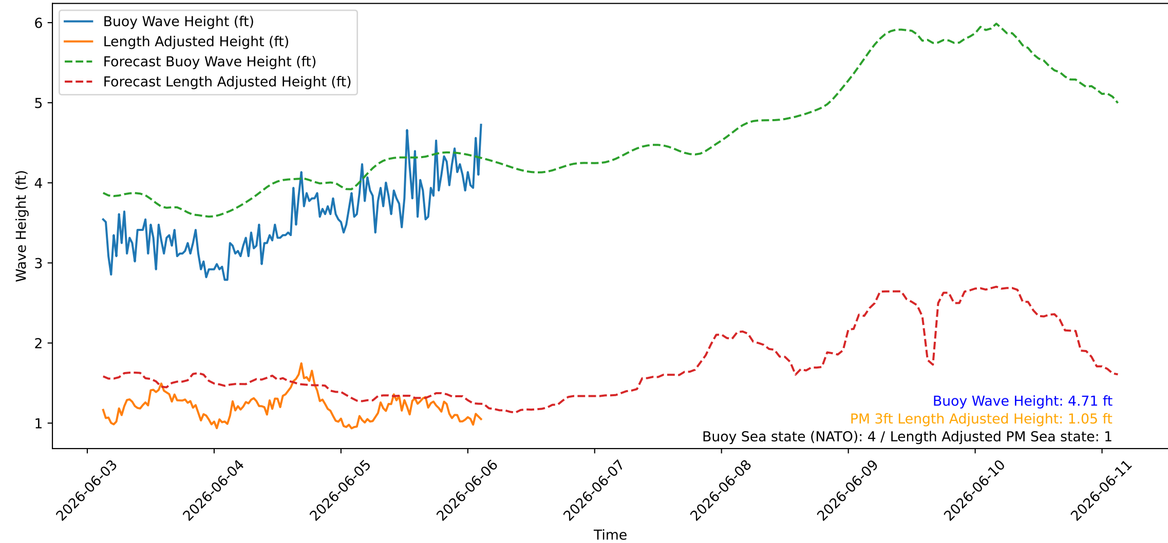
Wave Heights over Time for Green Beach at 2026-06-06 03:11:08
