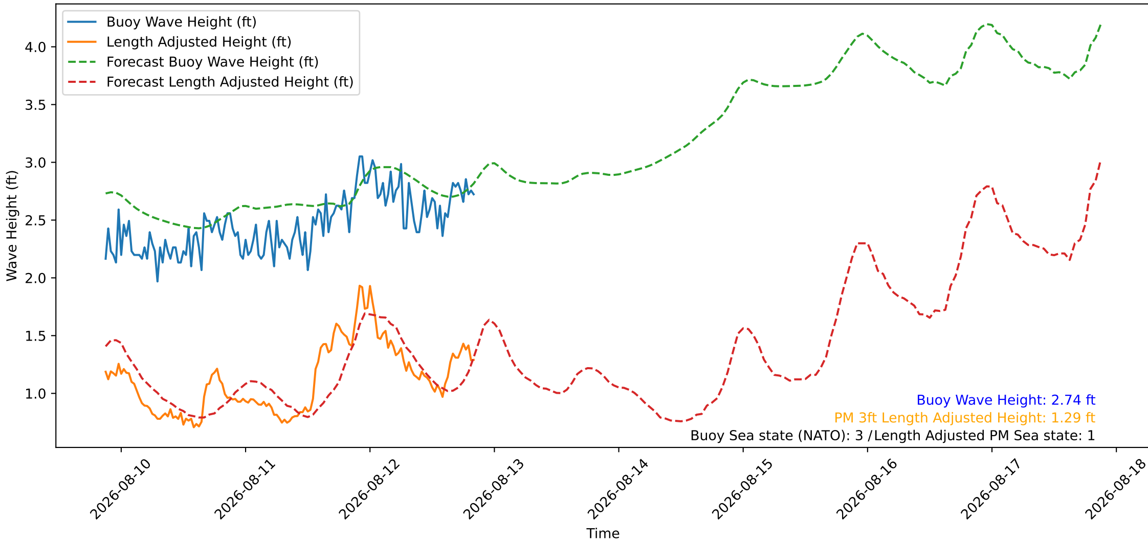
Wave Heights over Time for Oceanside Harbor at 2026-08-12 20:50:27
