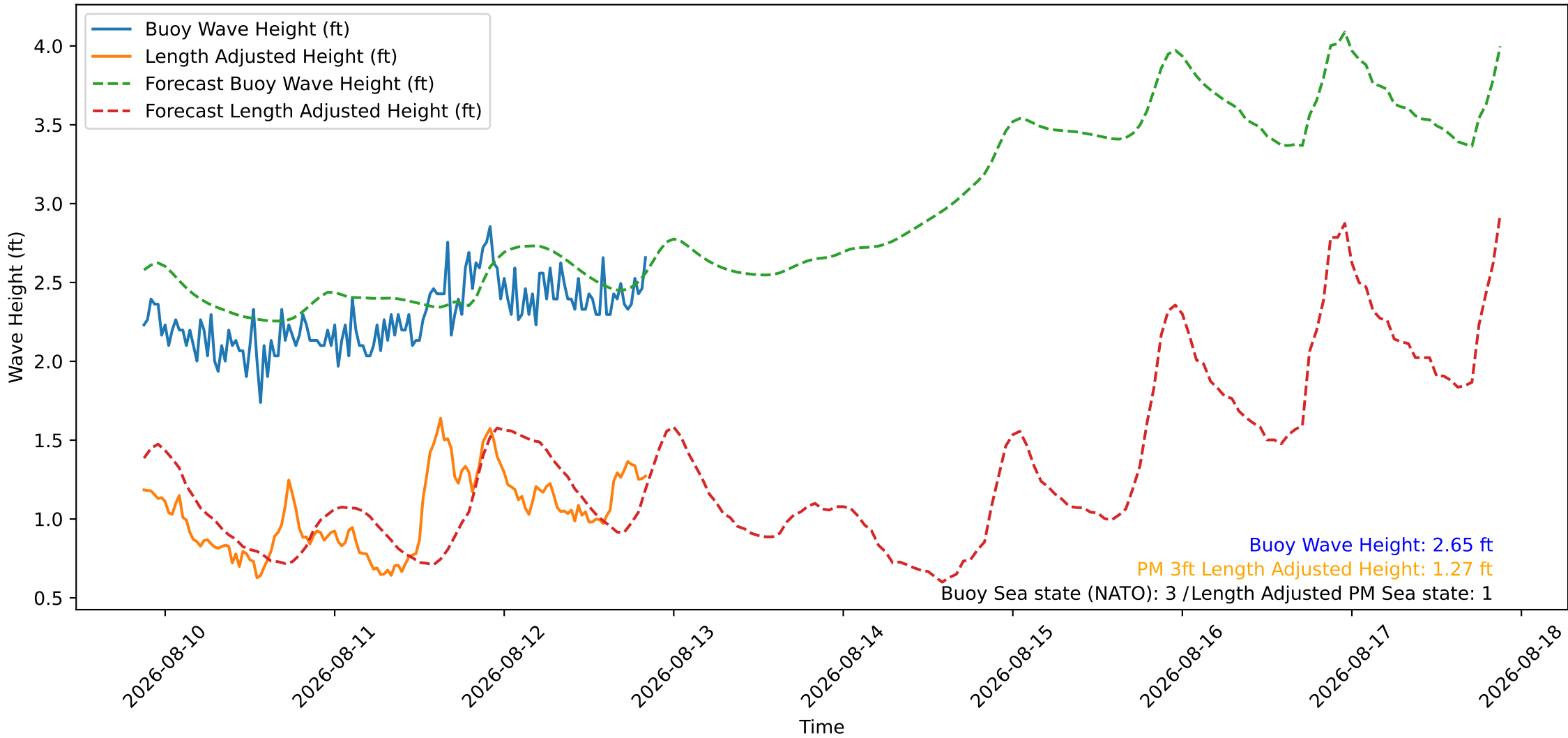
Wave Heights over Time for Red Beach at 2026-08-12 20:50:48
