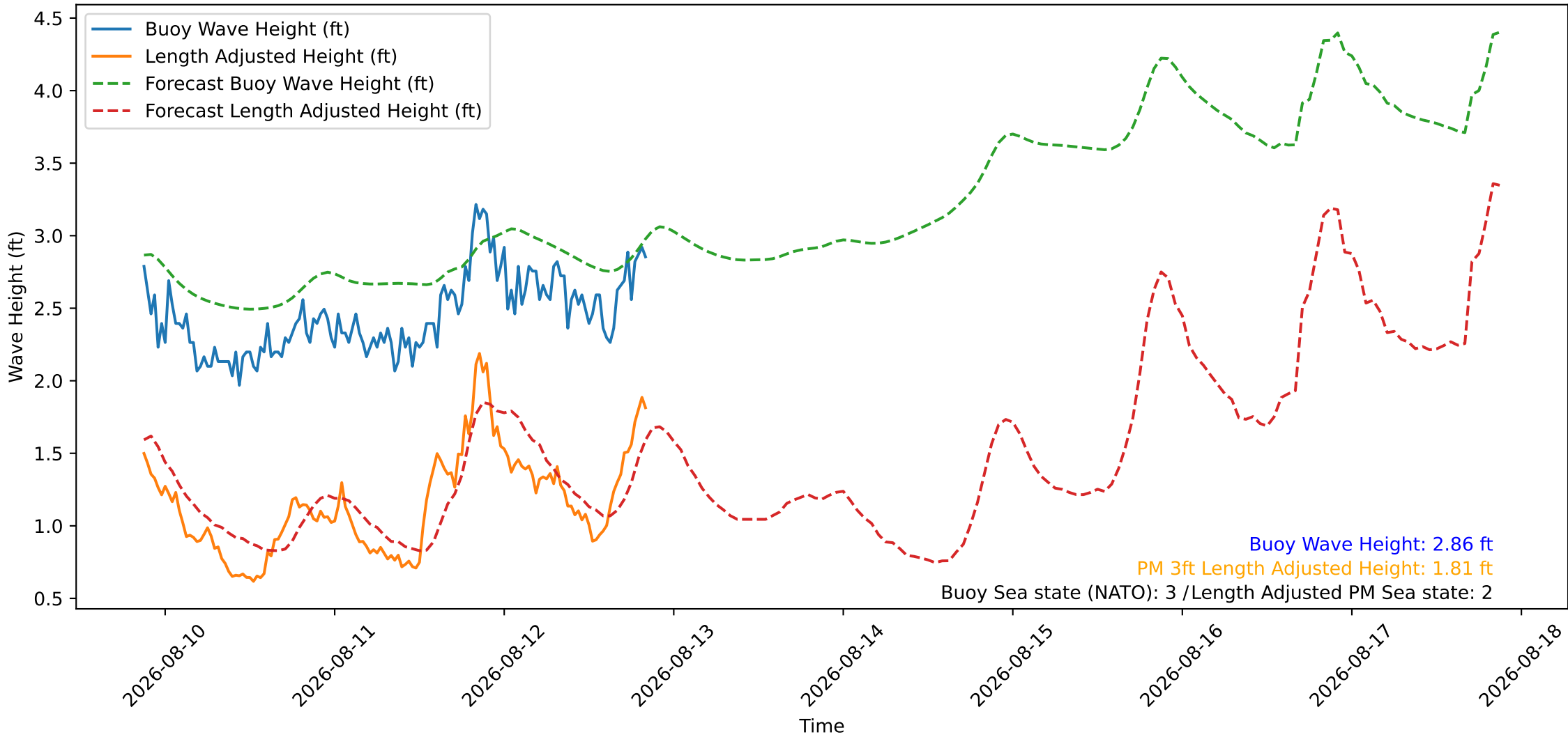
Wave Heights over Time for Green Beach at 2026-08-12 20:51:10
