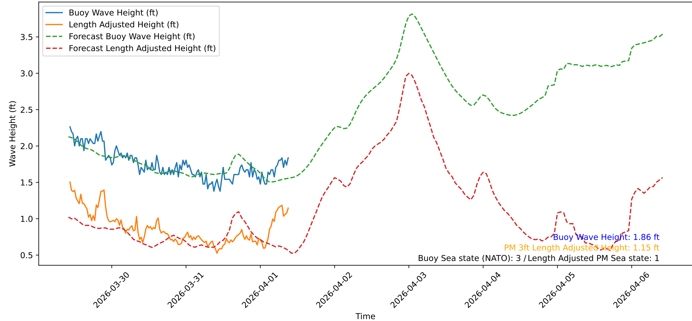
Wave Heights over Time for Red Beach at 2026-04-01 10:00:48
