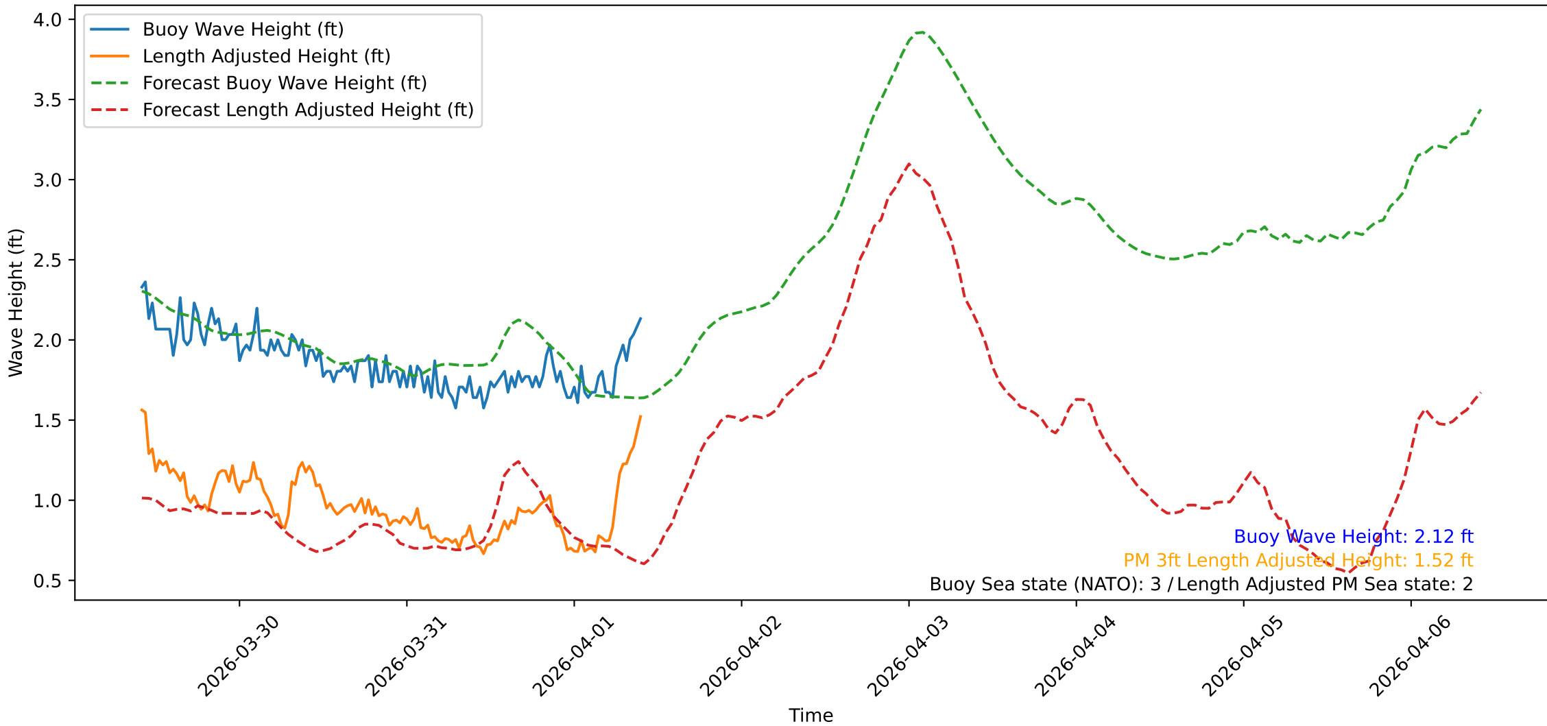
Wave Heights over Time for Oceanside Harbor at 2026-04-01 10:00:32
