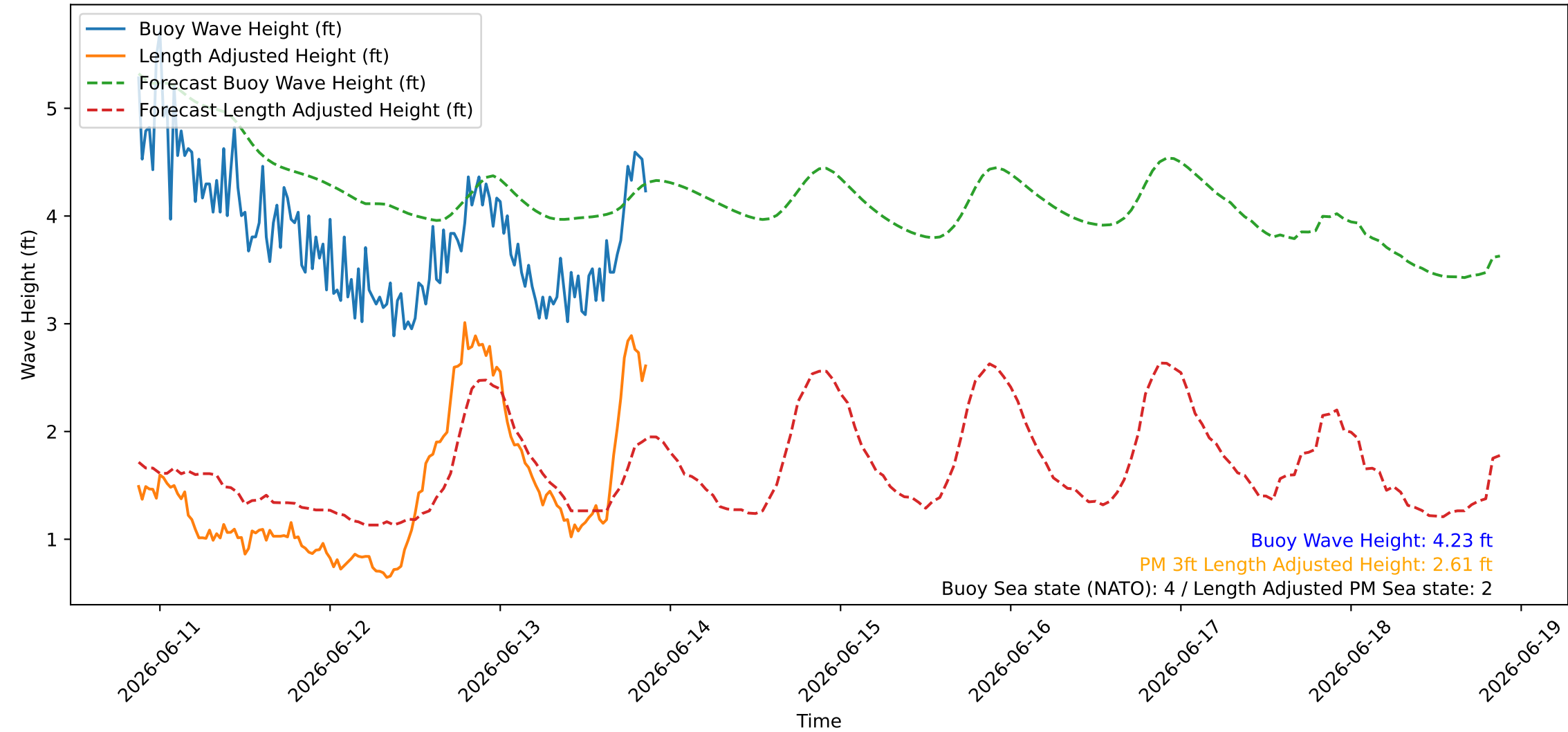
Wave Heights over Time for Green Beach at 2026-06-13 21:11:09
