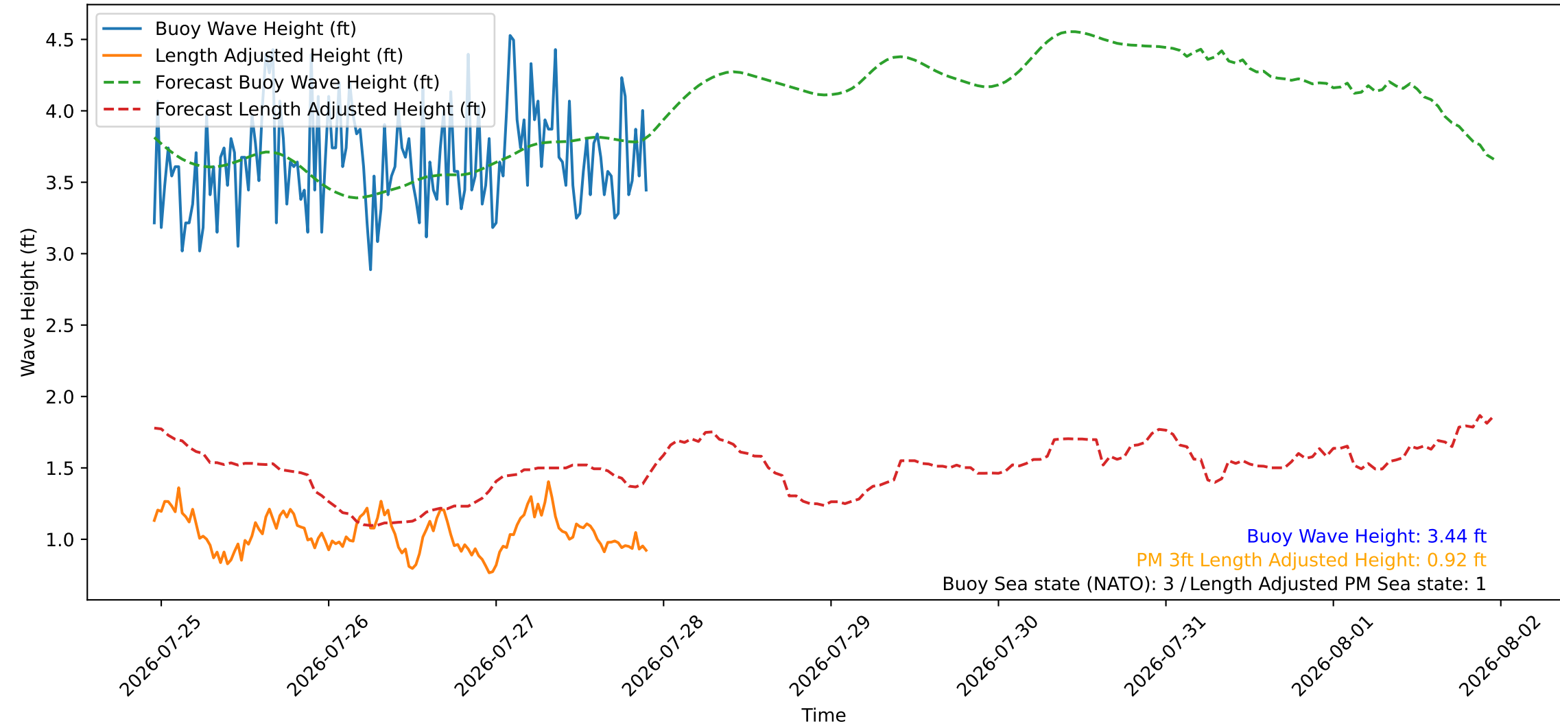
Wave Heights over Time for Red Beach at 2026-07-27 22:30:45
