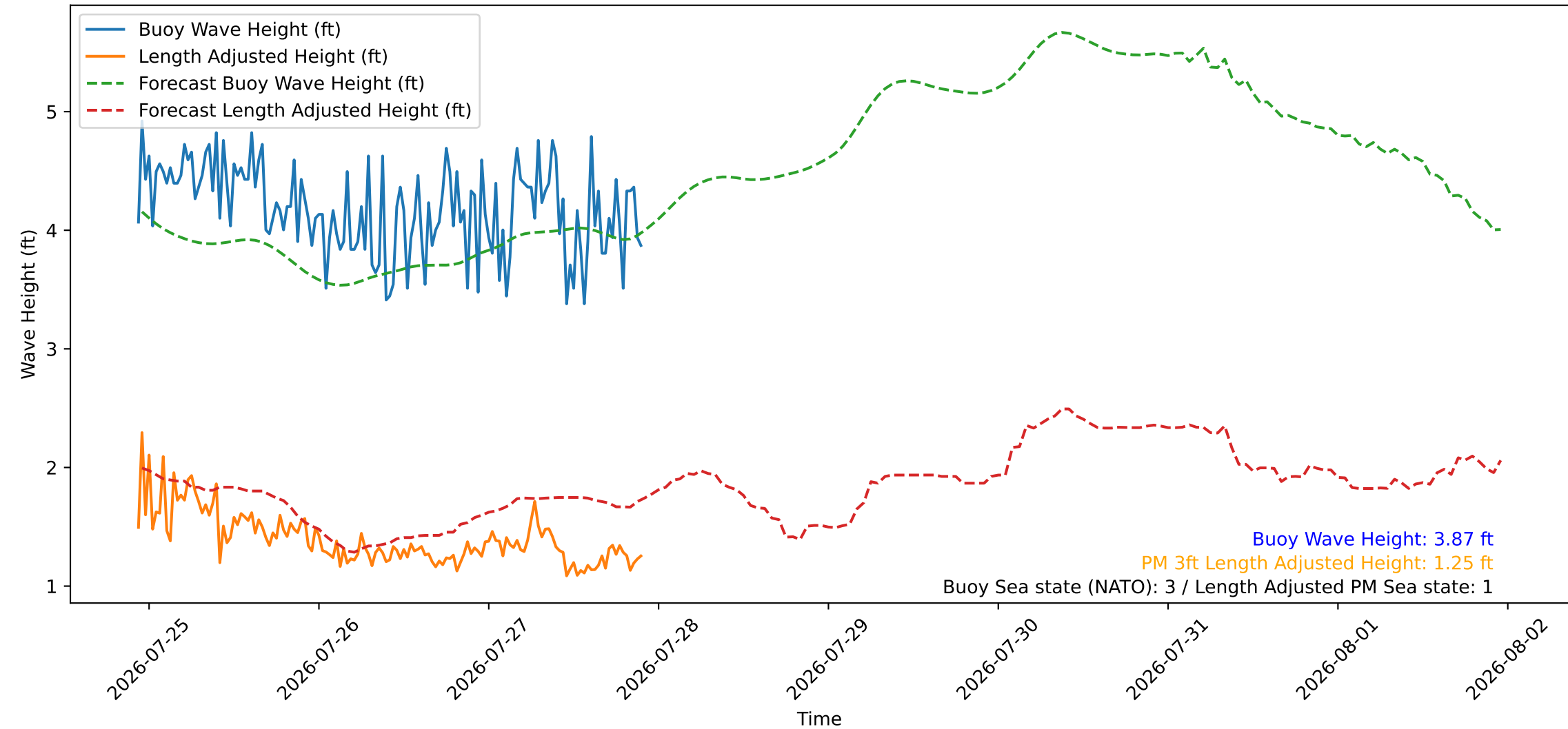
Wave Heights over Time for Green Beach at 2026-07-27 22:31:08
