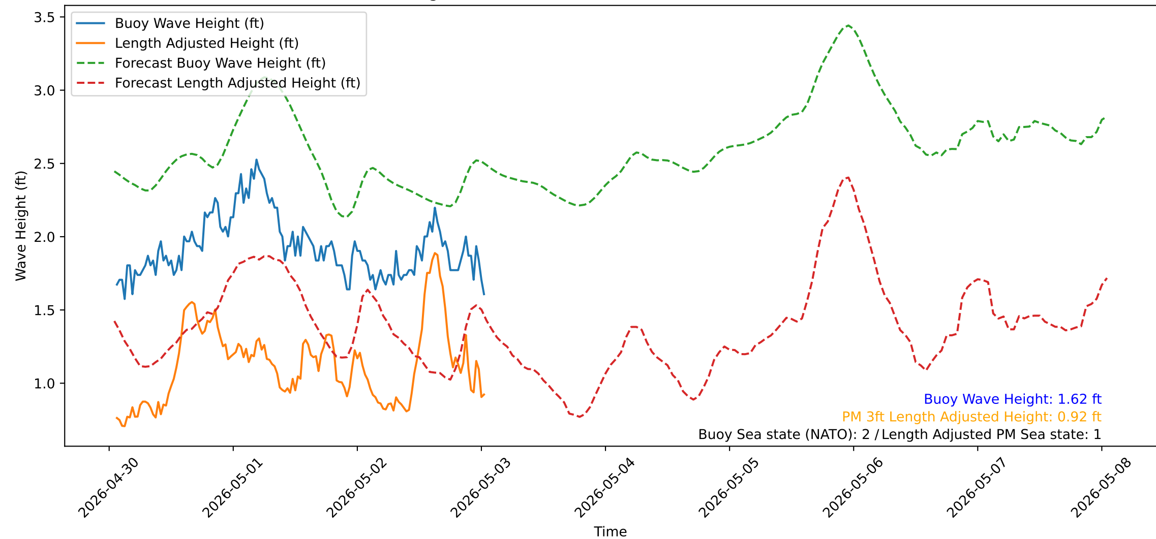
Wave Heights over Time for Red Beach at 2026-05-03 01:10:51
