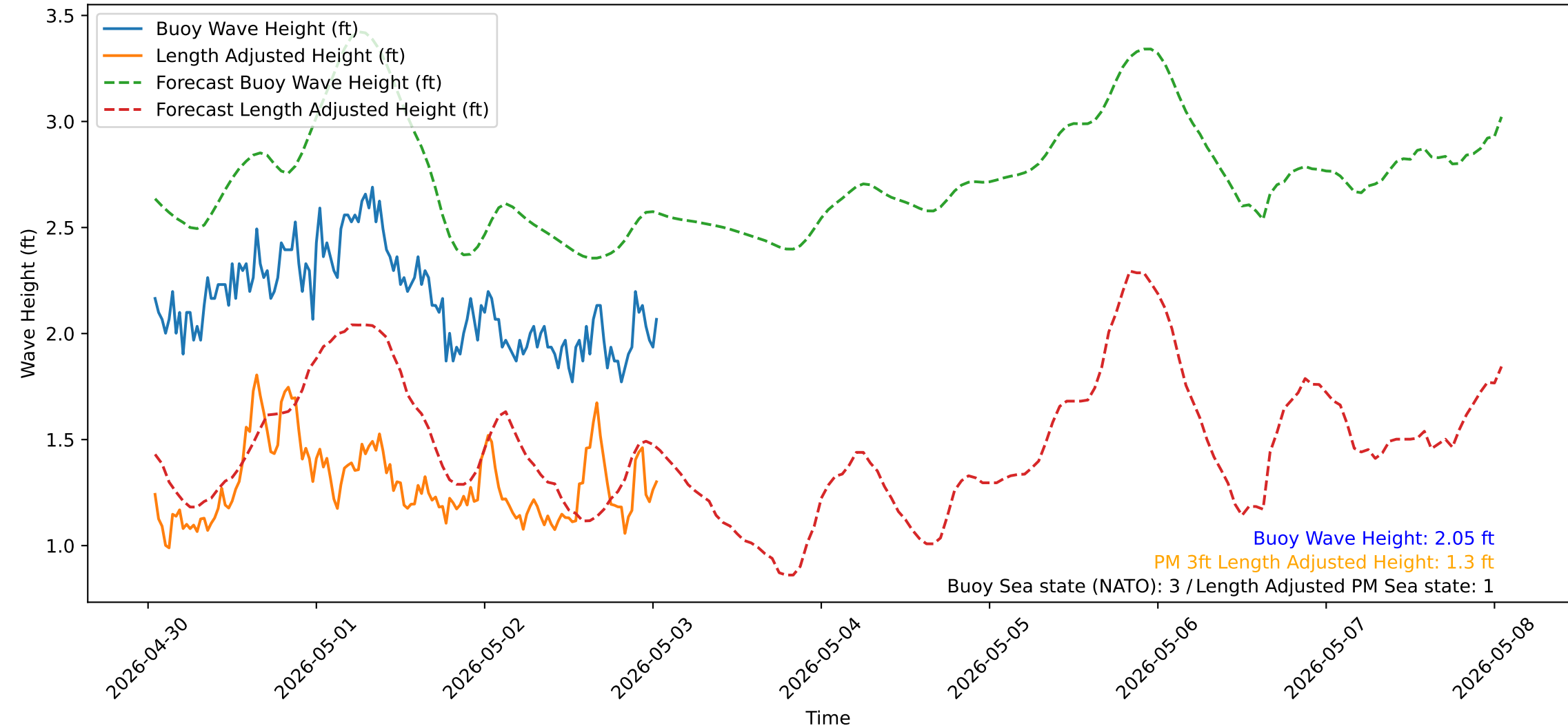
Wave Heights over Time for Oceanside Harbor at 2026-05-03 01:10:32
