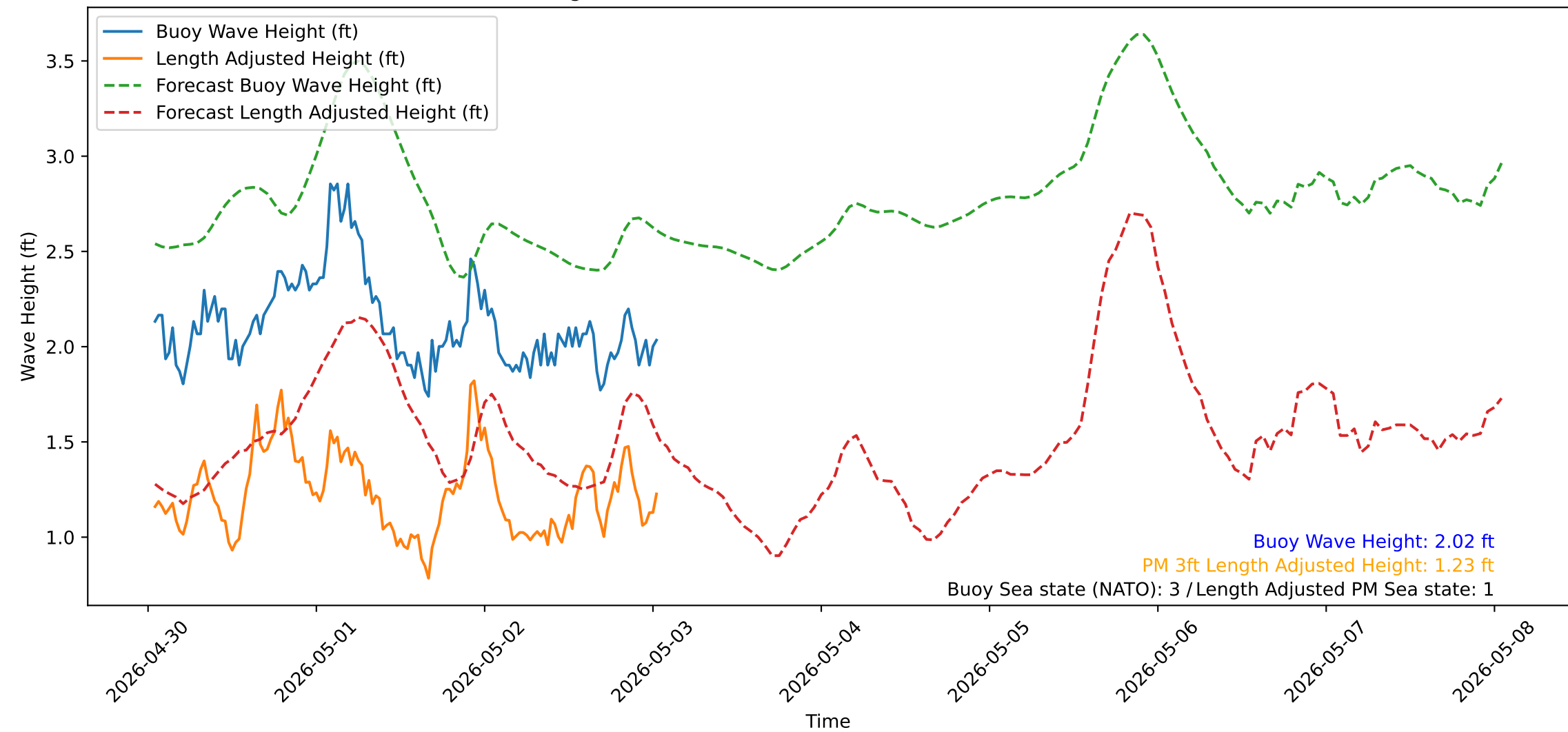
Wave Heights over Time for Green Beach at 2026-05-03 01:11:13
