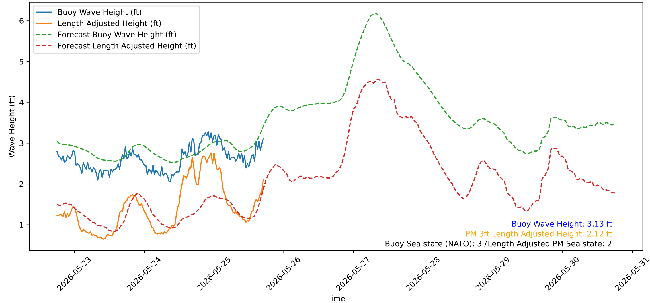
Wave Heights over Time for Green Beach at 2026-05-25 18:01:11
