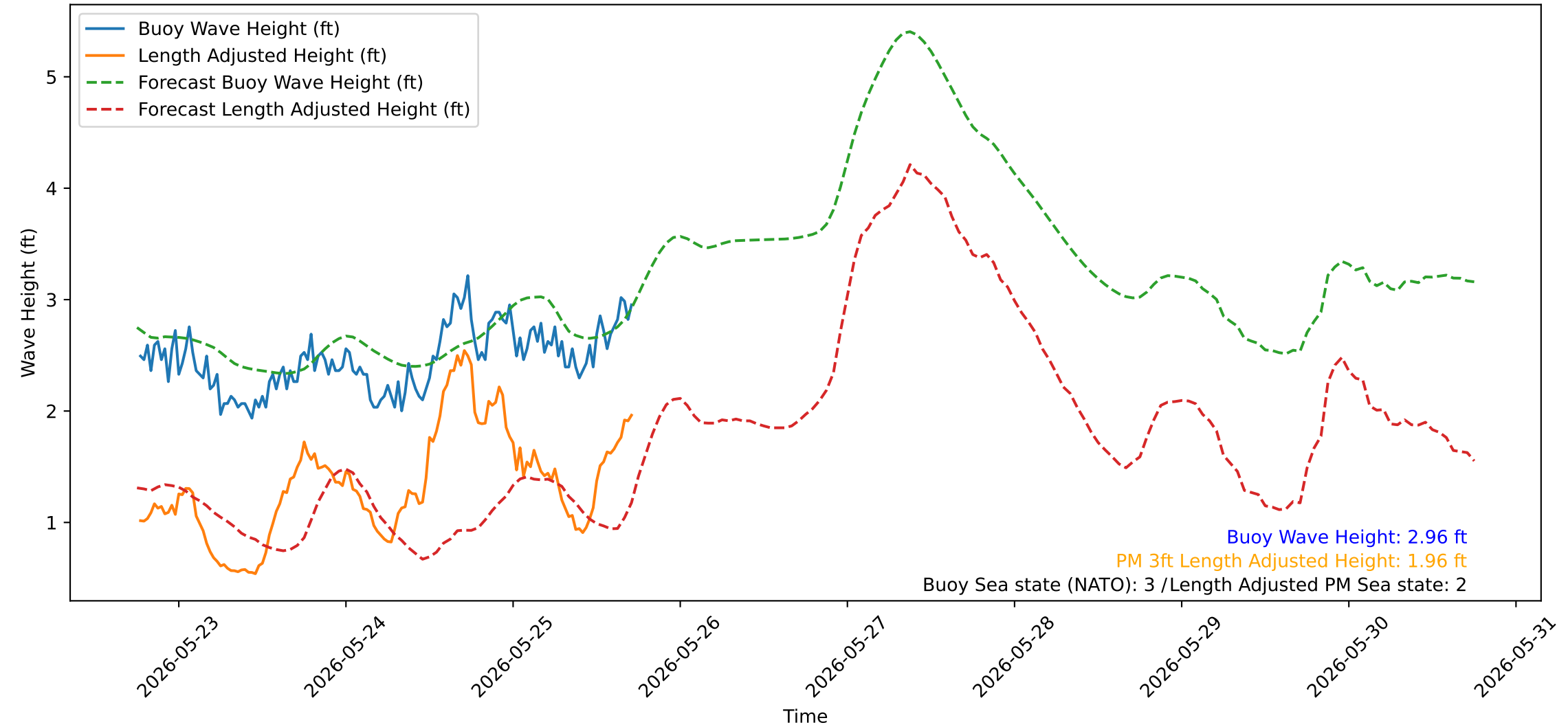
Wave Heights over Time for Red Beach at 2026-05-25 18:00:48
