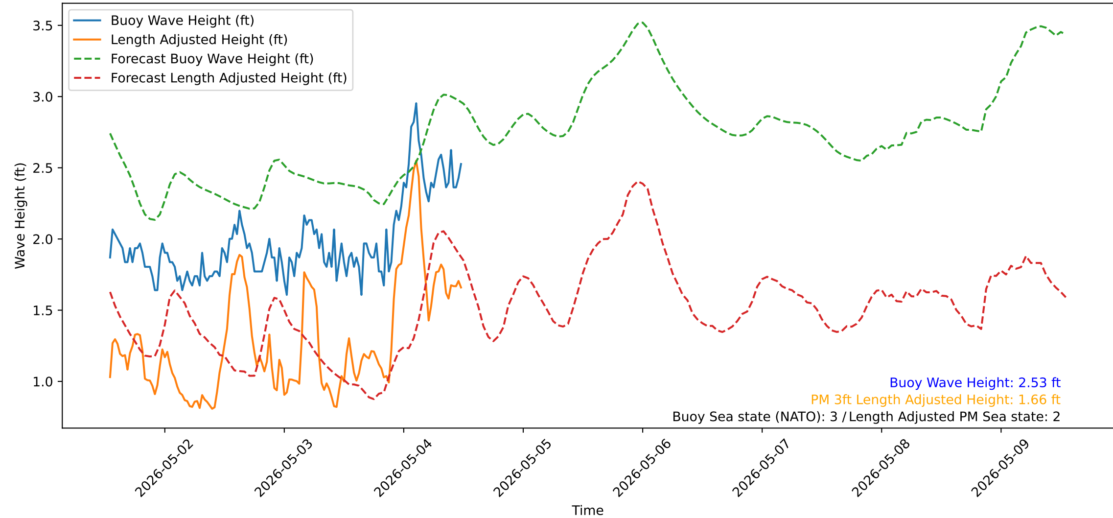
Wave Heights over Time for Red Beach at 2026-05-04 12:30:51
