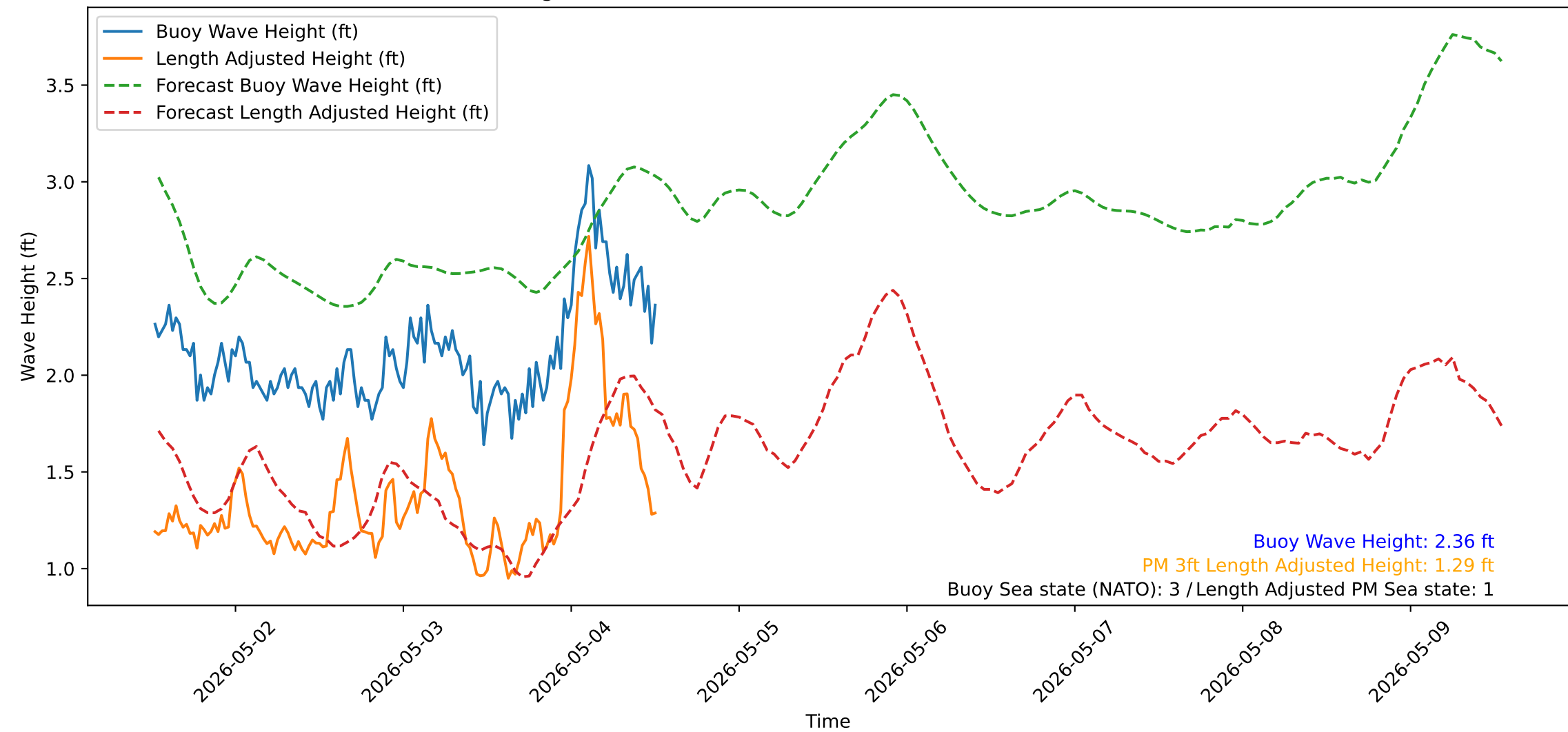
Wave Heights over Time for Oceanside Harbor at 2026-05-04 12:30:32
