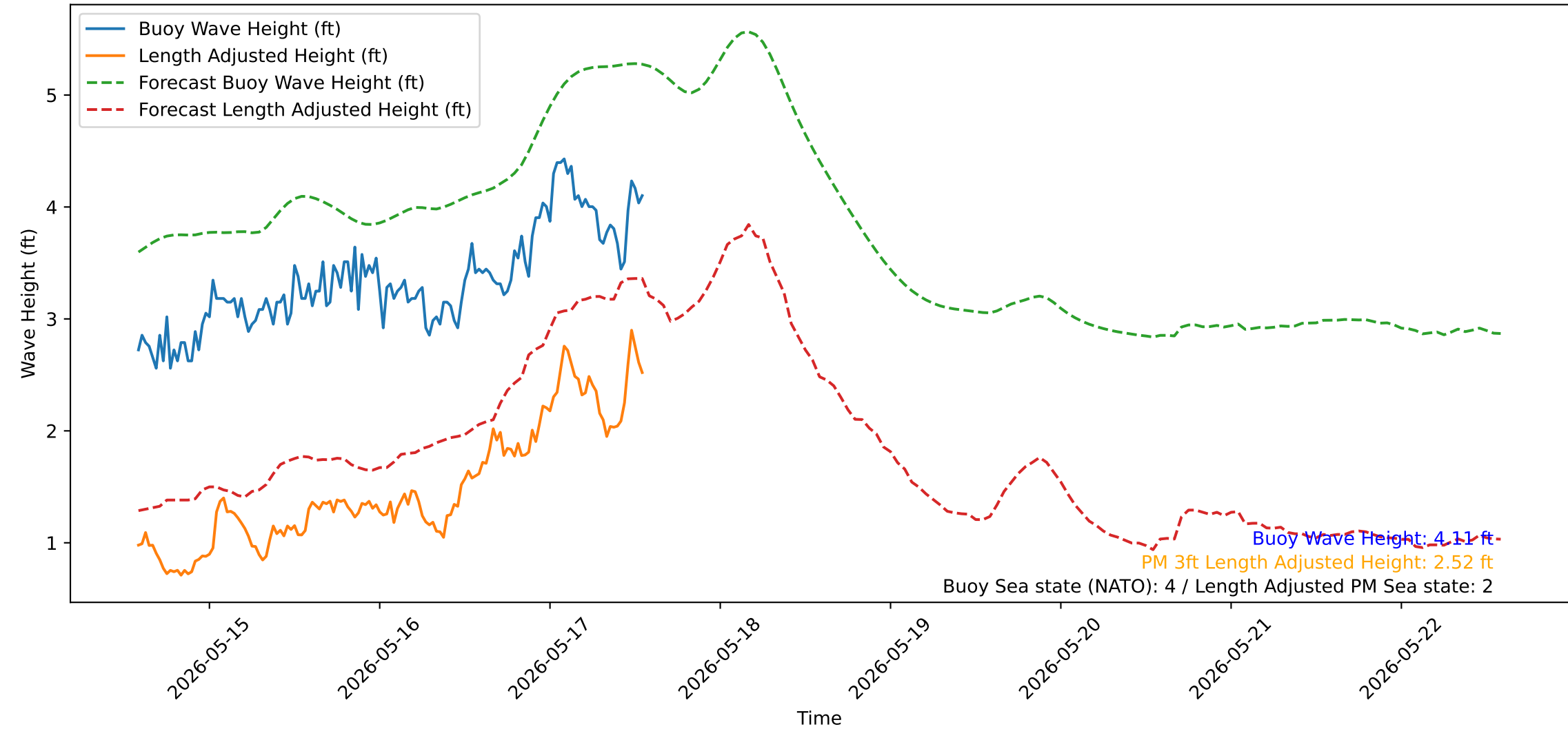
Wave Heights over Time for Green Beach at 2026-05-17 13:51:14
