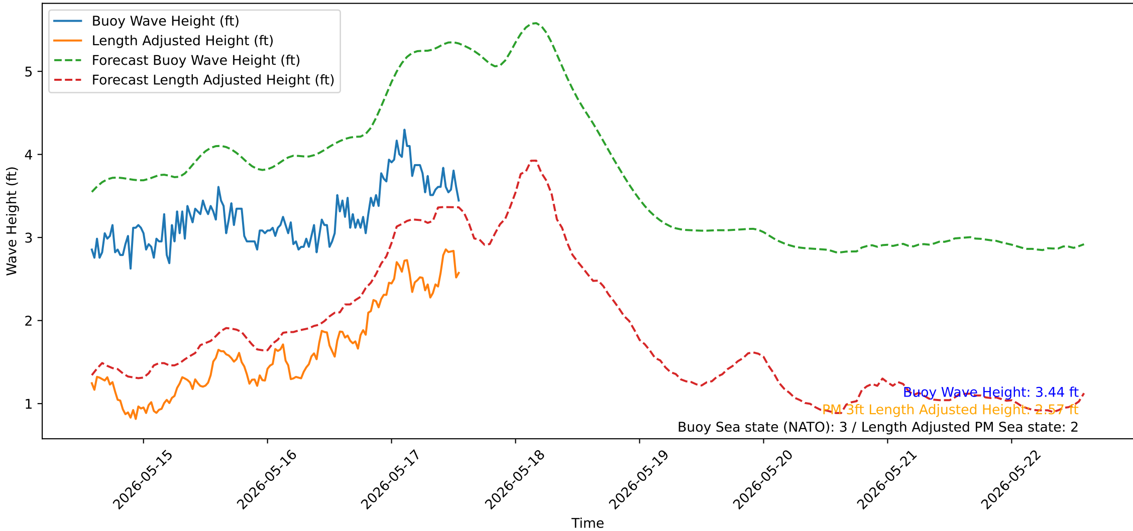
Wave Heights over Time for Oceanside Harbor at 2026-05-17 13:50:31
