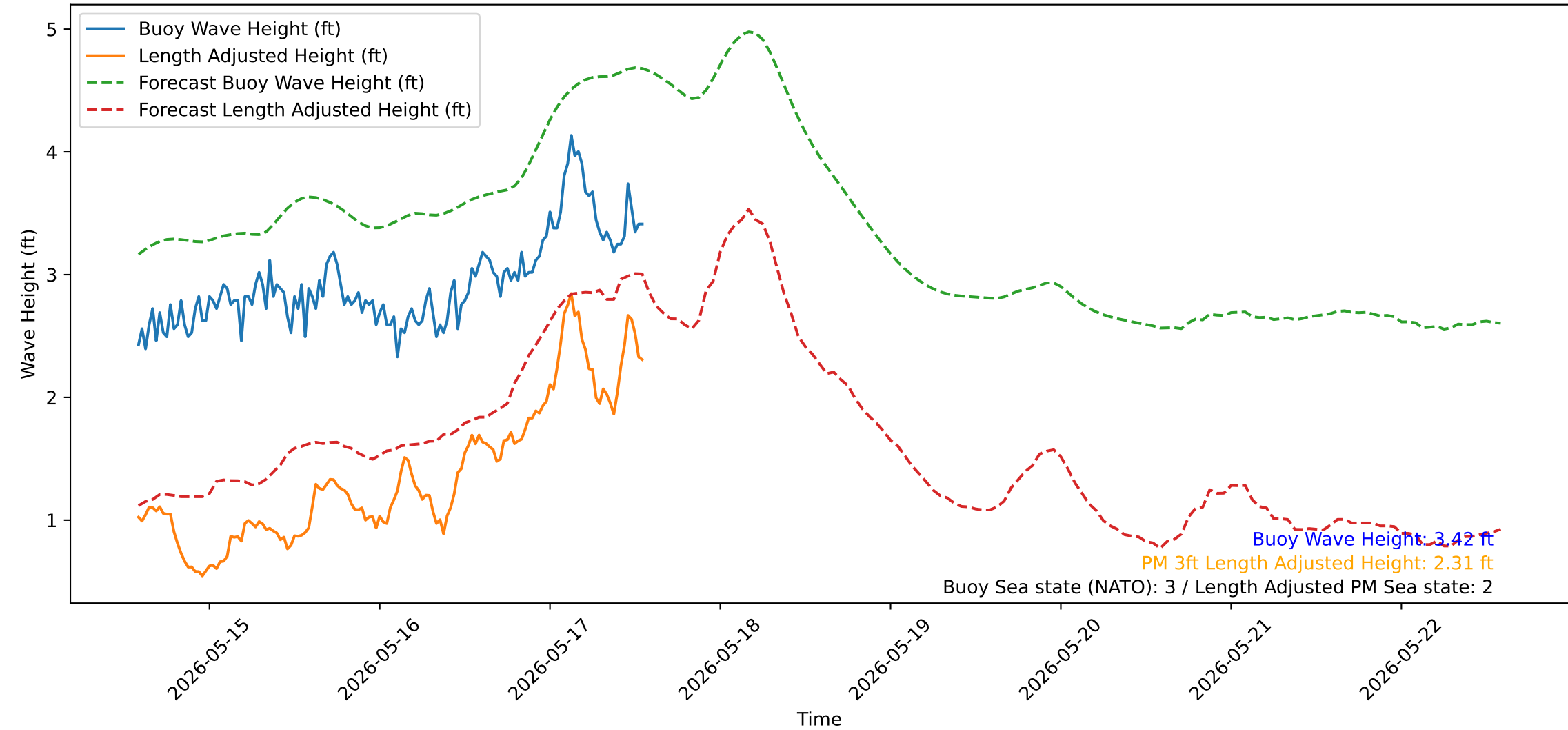
Wave Heights over Time for Red Beach at 2026-05-17 13:50:51
