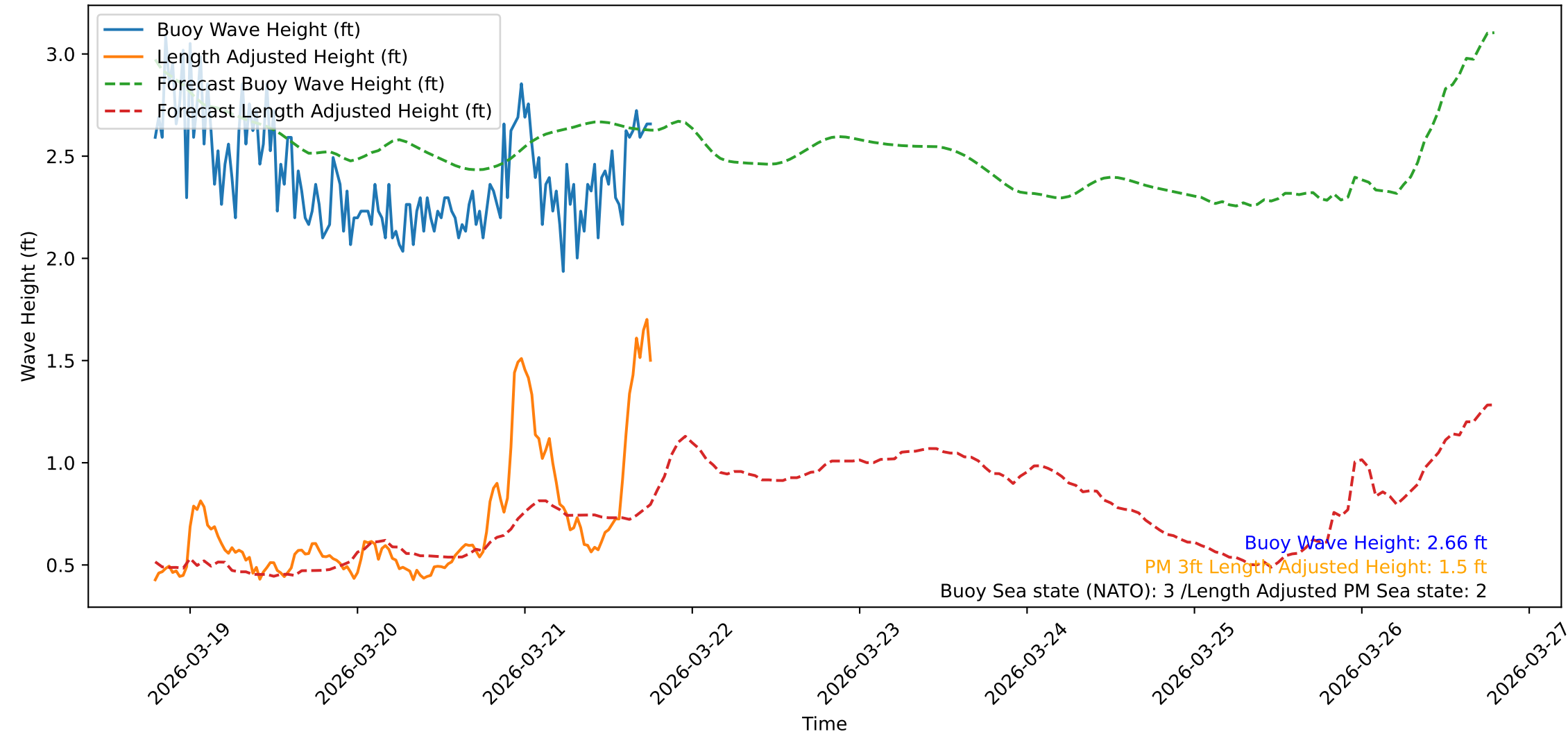
Wave Heights over Time for Green Beach at 2026-03-21 18:51:10
