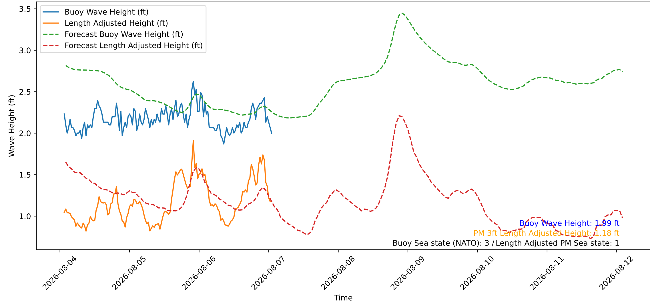
Wave Heights over Time for Green Beach at 2026-08-07 01:41:09
