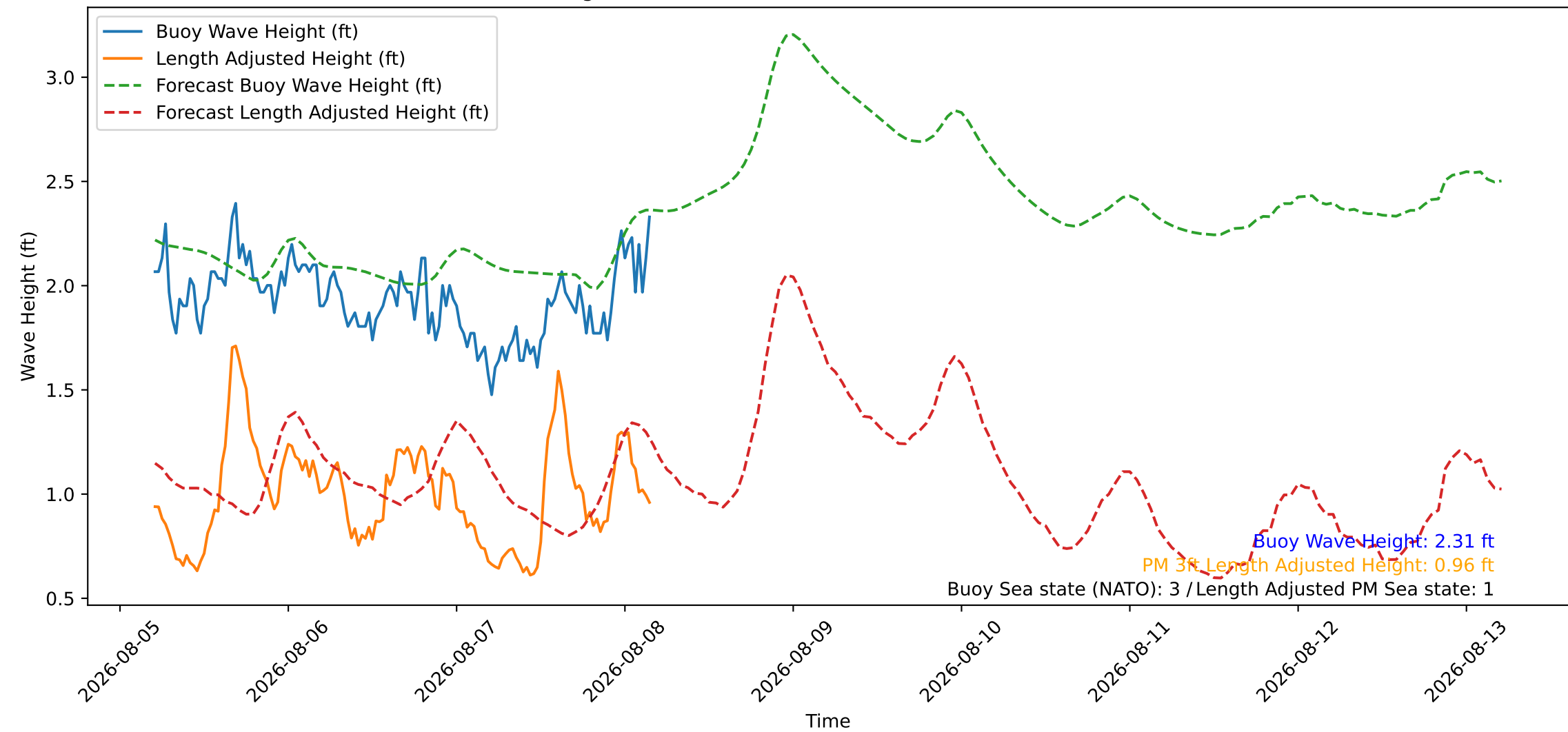
Wave Heights over Time for Red Beach at 2026-08-08 04:50:48
