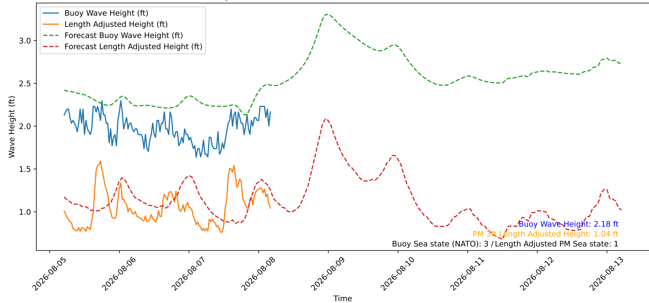
Wave Heights over Time for Oceanside Harbor at 2026-08-08 04:50:26
