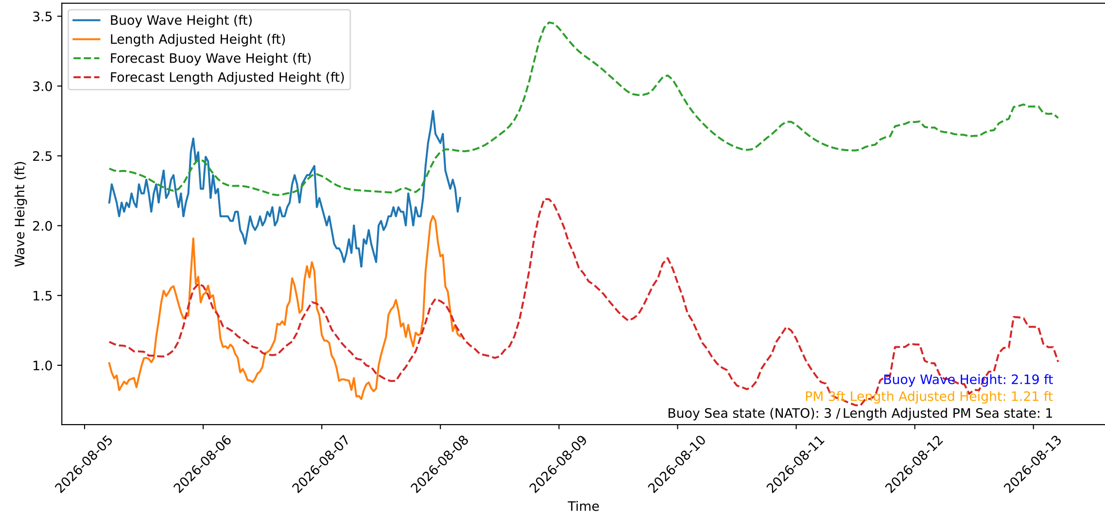
Wave Heights over Time for Green Beach at 2026-08-08 04:51:10
